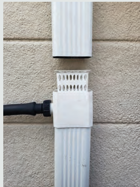
These downspout diverters are installed in line with the downspout. A portion of the rainwater flow will be diverted to the rain barrel through the hose attachment. Some come with built in screens to keep out debris.
