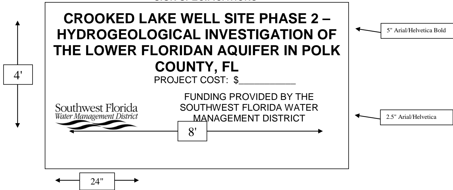
FIGURE 5 SIGN SPECIFICATIONS
