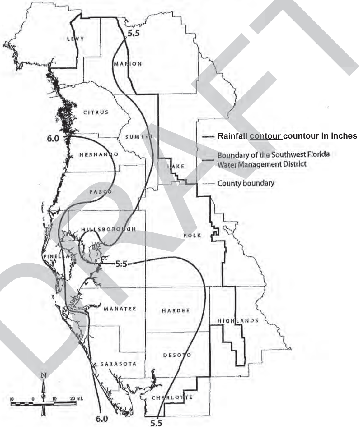
Figure D-3 Twenty-Four-Hour Five-Year Return Period Rainfall Map
