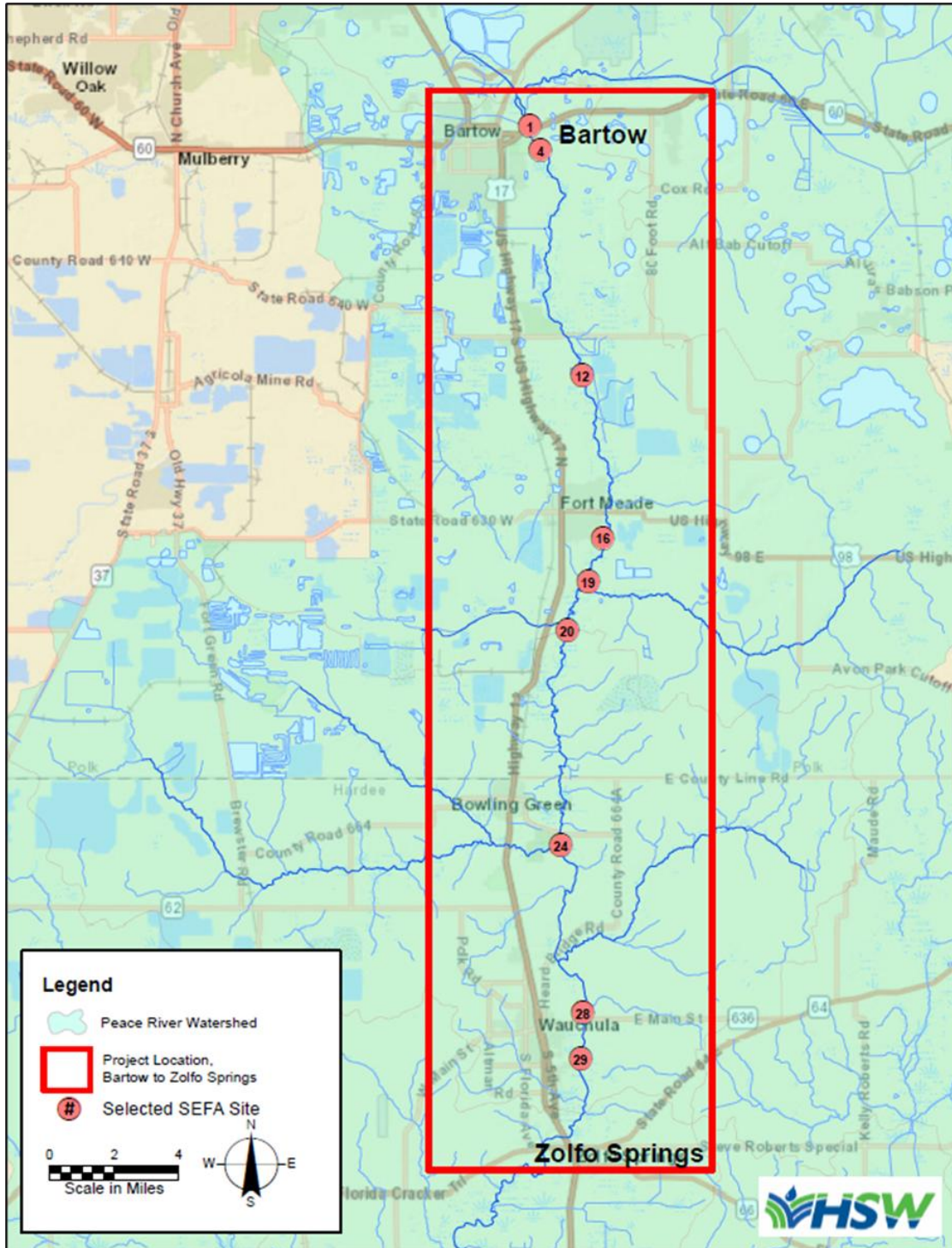
Figure 5-4. Locations of nine SEFA data collection sites in the Upper Peace River.
