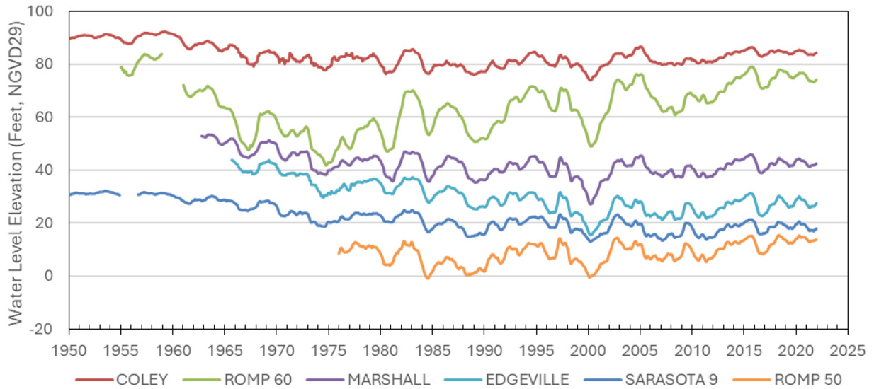
Figure 2-19. Water levels in Southern Water Use Causion Area (SWUCA) monitoring wells (12-month moving average).
