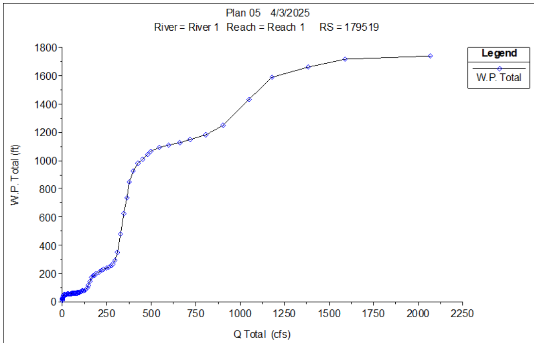
Figure 5-13. Total wetted perimeter versus discharge at Site 179519.
