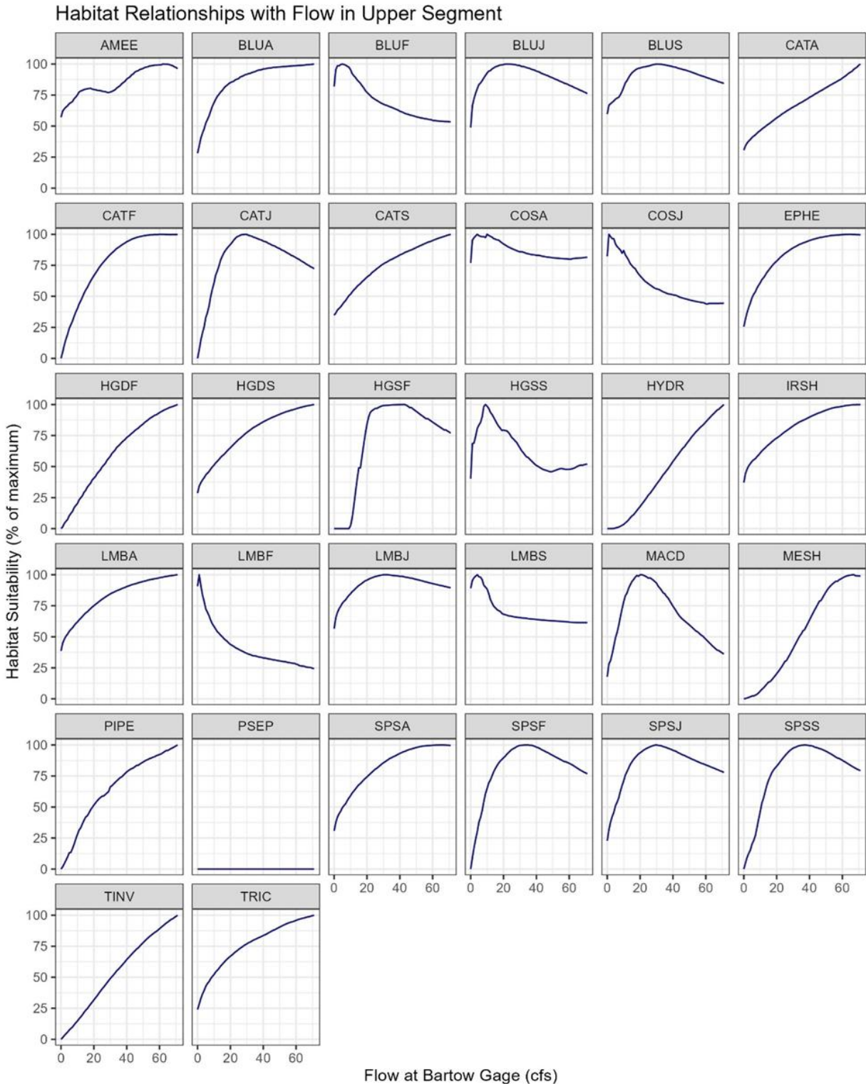
Figure 5-17. Average habitat – flow relationships in the upper segment of the Upper Peace River. Habitat suitability is expressed relative to the maximum for each species; all species with any habitat reach a maximum of 100% at some flow. The curves illustrate how habitat suitability responds to changes in flow. PSEP does not exhibit suitable habitat under any flow condition.
