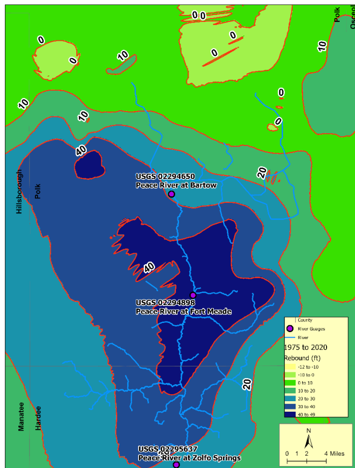
Figure 2-20. Estimated rebound of the potentiometric surface of the Upper Floridan aquifer from May 1975 to May 2020. Modified flow from Zhang (2024, Appendix C).
