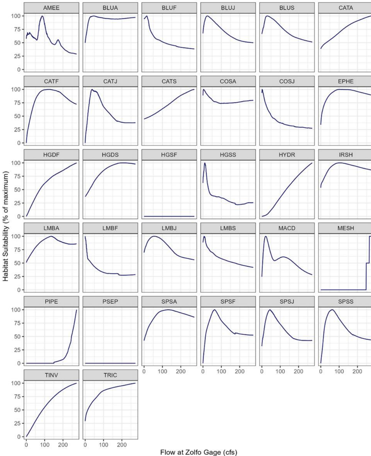
Figure 5-21. Average habitat – flow relationships in the upper segment of the Upper Peace River. Habitat suitability is expressed relative to the maximum for each species; all species with any habitat reach a maximum of 100% at some flow. The curves illustrate how habitat suitability responds to changes in flow. PSEP does not exhibit suitable habitat under any flow condition.
