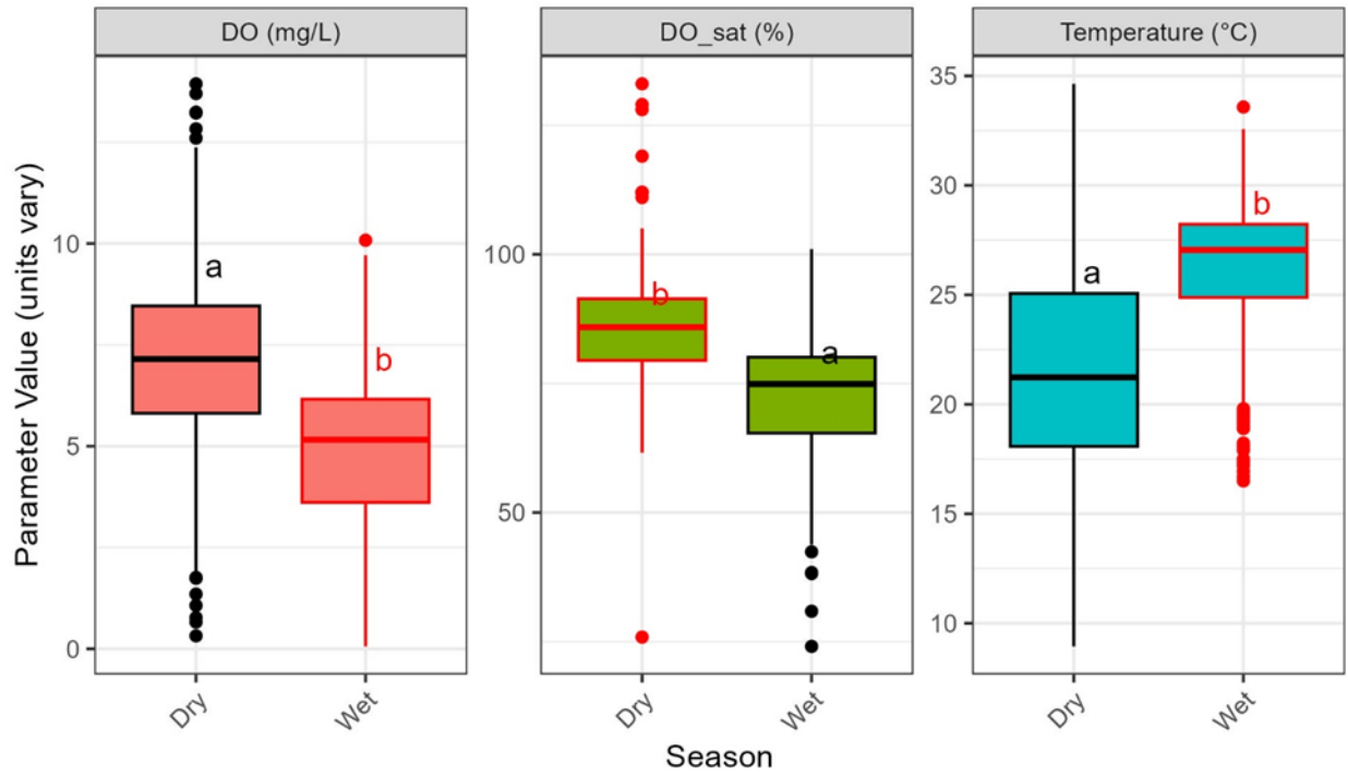
Figure 3-14. Seasonal differences in dissolved oxygen and water temperature. Boxes with different outline colors and letters are significantly different according to a Wilcoxon rank-sum test.
