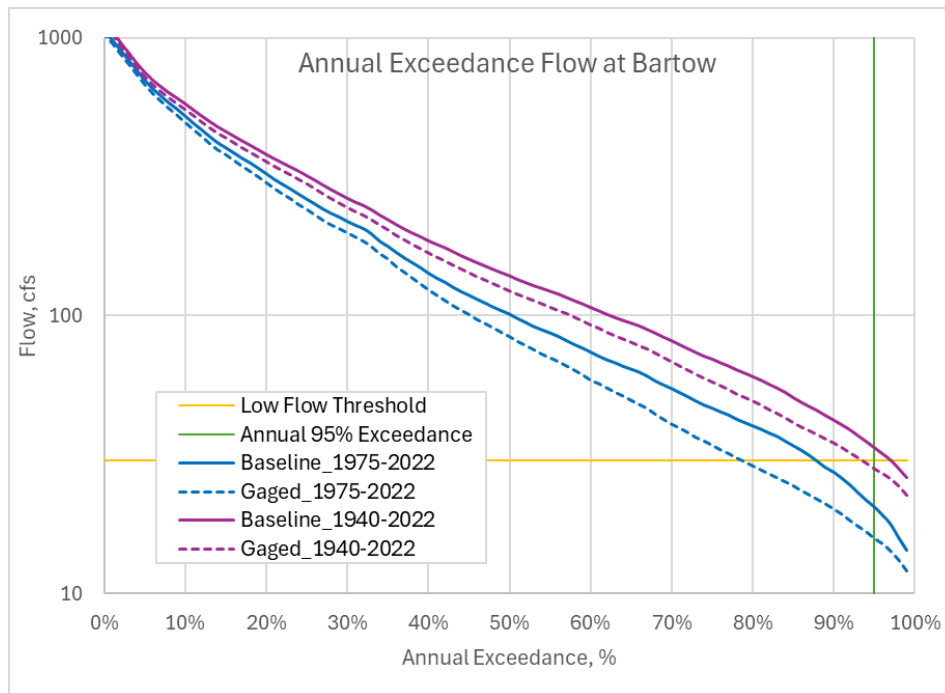
Figure 6-5. Annual exceedance flow for the USGS Peace River gage at Bartow for the periods 1975-2022 and 1940-2022, comparing baseline and gaged flows in relation to the low flow threshold.
