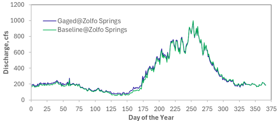
Figure 5-10. Median daily historical and baseline flow at the USGS Peace River gages: Bartow (upper), Fort Meade (middle), and Zolfo Springs (lower).
