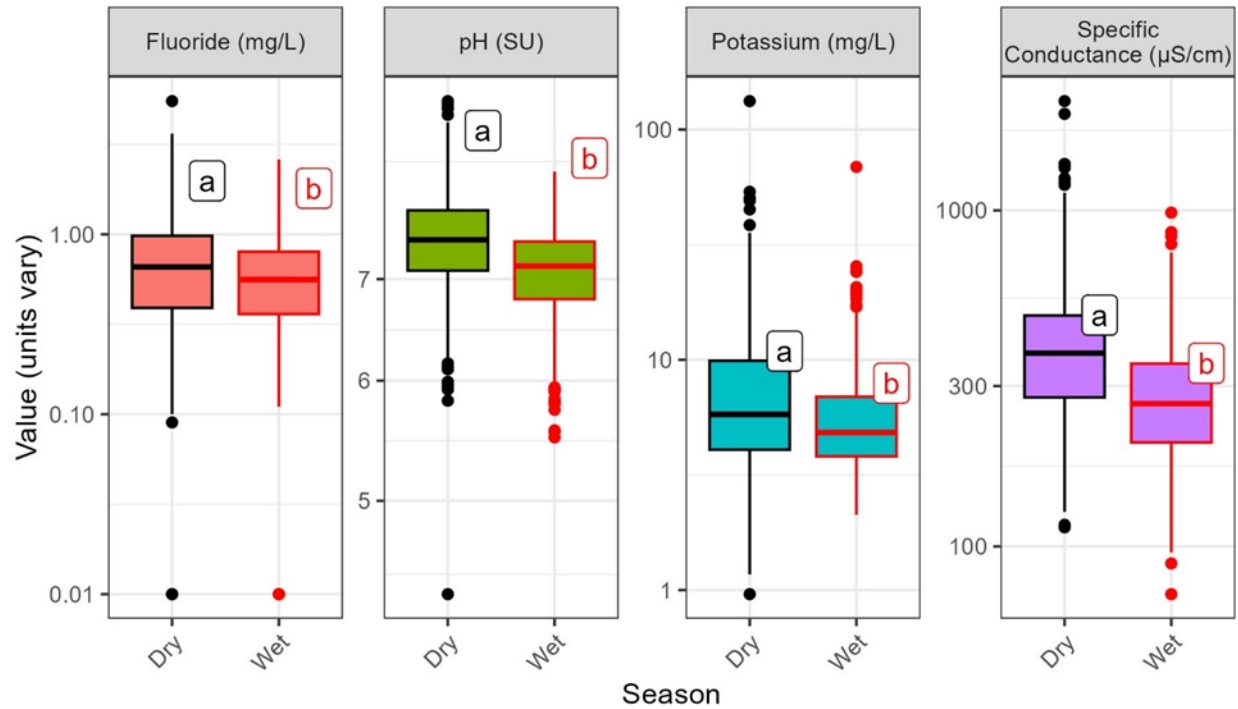
Figure 3-11. Seasonal differences in inorganic ions. Boxes with different outline colors and letters are significantly different according to a Wilcoxon rank-sum test.
