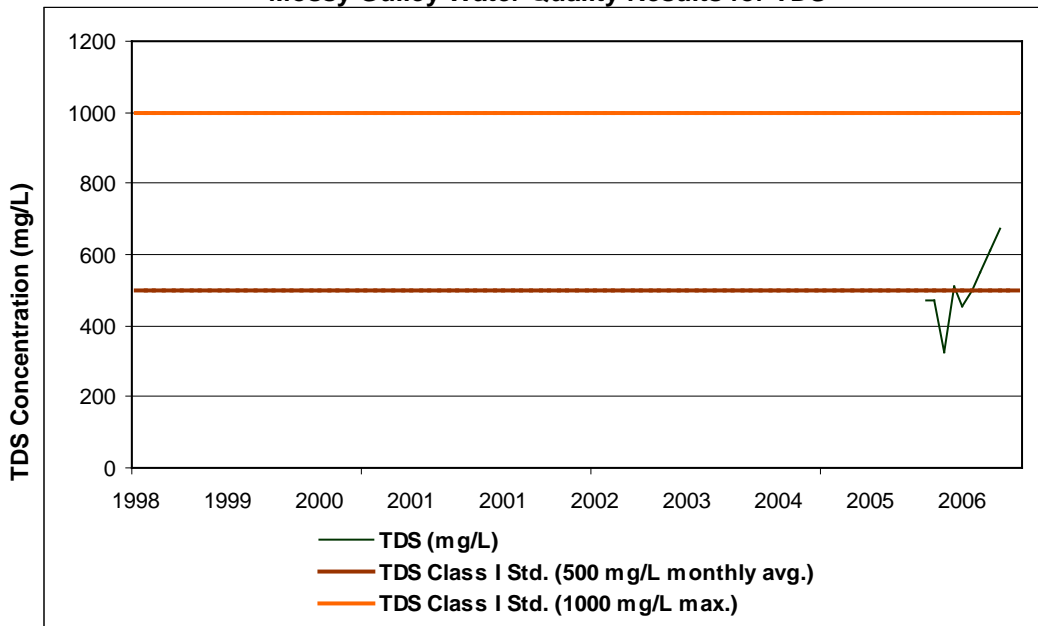
Mossy Gulley Water Quality Results for TDS
