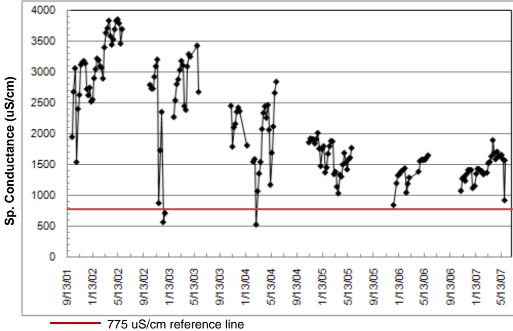
Hog Bay Slough In-Situ Data Sonde Logging Results
