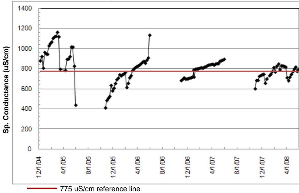
Gannett Slough In-Situ Data Sonde Logging Results
