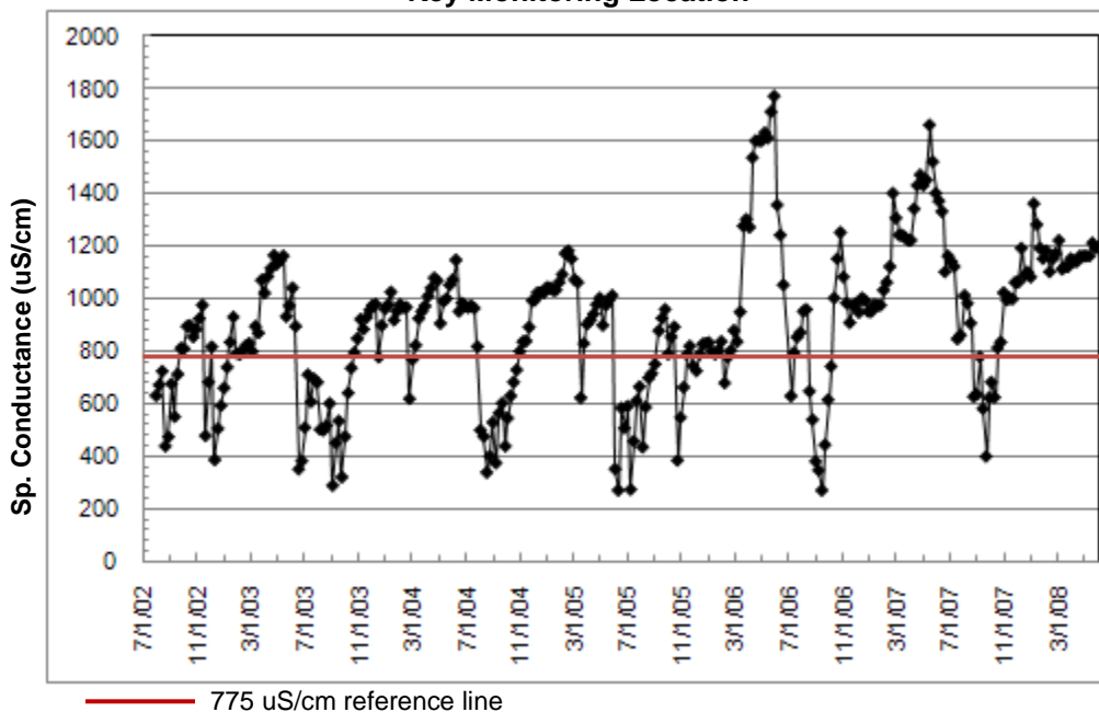
Specific Conductance Logging Results in WBID 2041 over Entire Period of Data Record Sites are listed as they are located from east to west throughout WBID 2041
