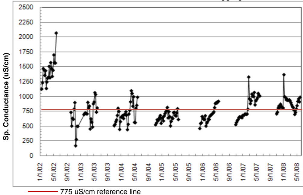
Emerald Isle East Canal In-Situ Data Sonde Logging Results
