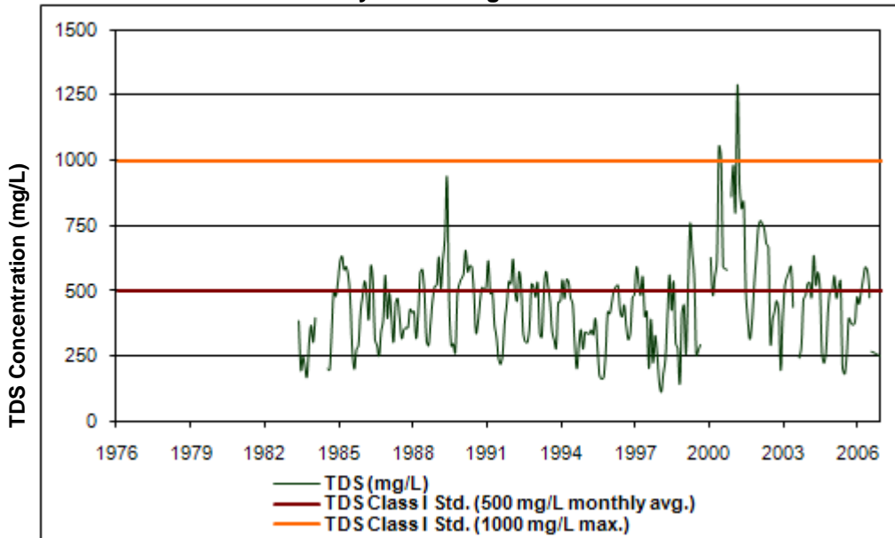
Prairie Creek @ Washington Loop Rd. Water Quality Results for TDS Key Monitoring Location
