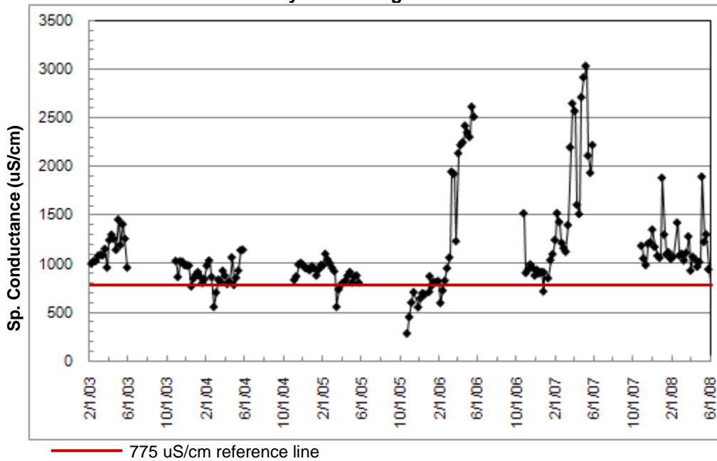
Shell Creek @ SR 31 In-Situ Data Sonde Logging Results Key Monitoring Location
