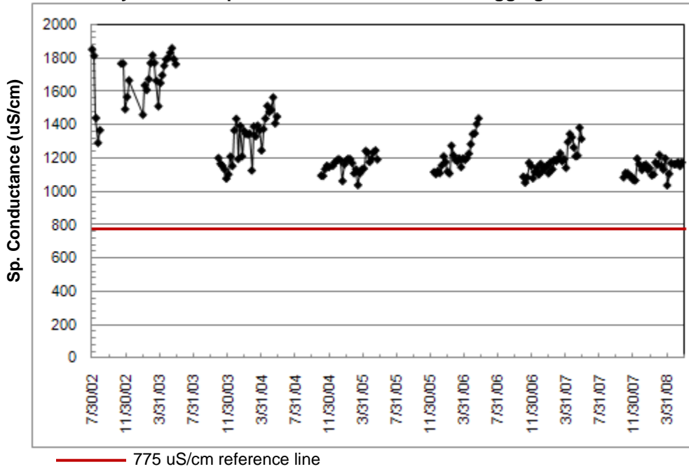
Symons Pump Canal In-Situ Data Sonde Logging Results
