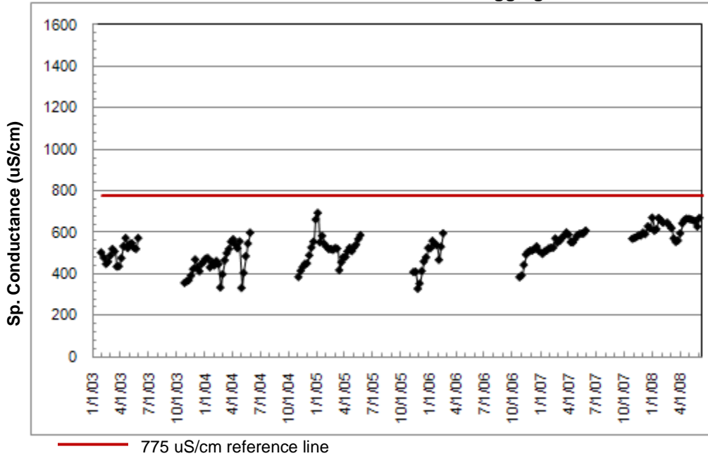
Doehill Main Canal In-Situ Data Sonde Logging Results
