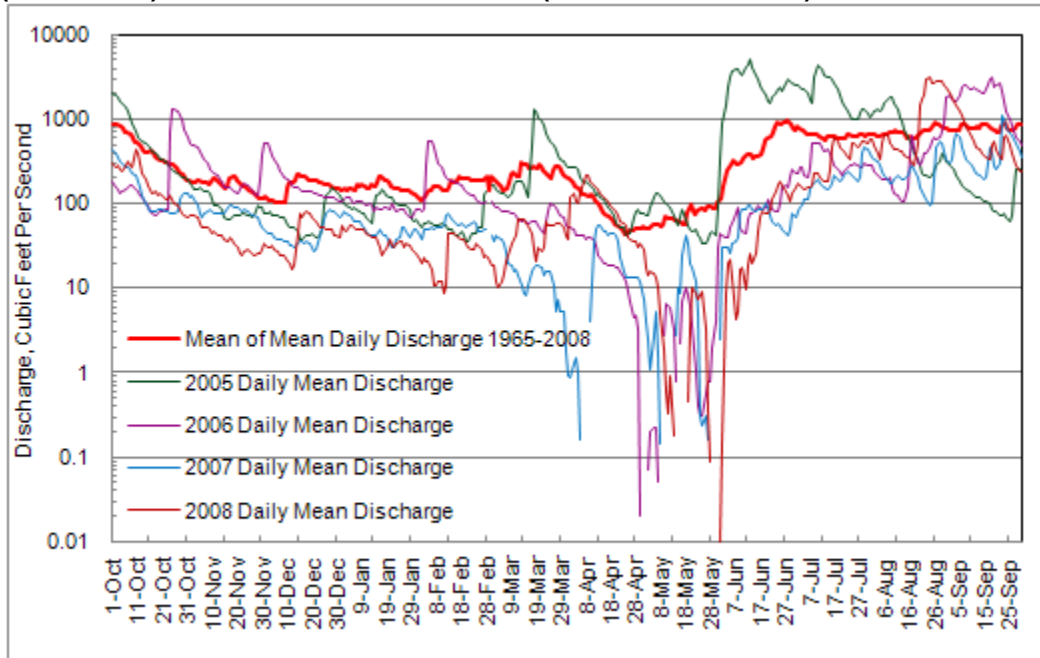
Figure 4. Long-term (1965-2008) mean of daily mean discharge, and daily mean discharge (2005 - 2008) for the Shell Creek Reservoir (USGS site 02298202).
