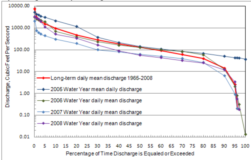
Figure 5. Discharge Duration Curves of 2005 - 2008 Annual Daily Discharge Compared to 43-year Long-Term Daily Discharge
