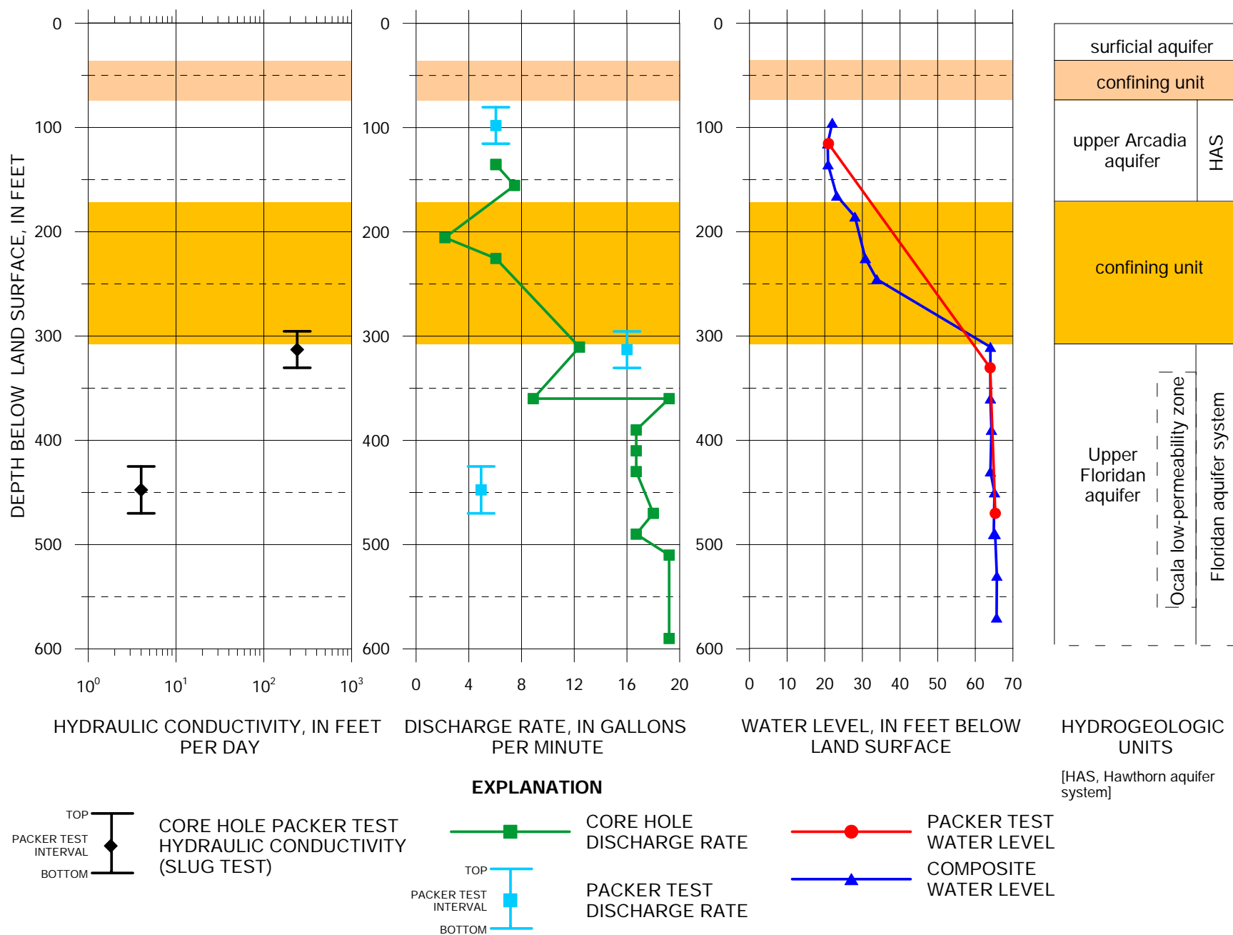
Figure 4. Horizontal hydraulic conductivity estimates and static water levels collected during core drilling at the ROMP 42 – Bereah well site in Polk County, Florida. Note: the higher discharge rates in the core hole within the Ocala low-permeability zone is coincident with an increase in the airline length by 100 feet.
