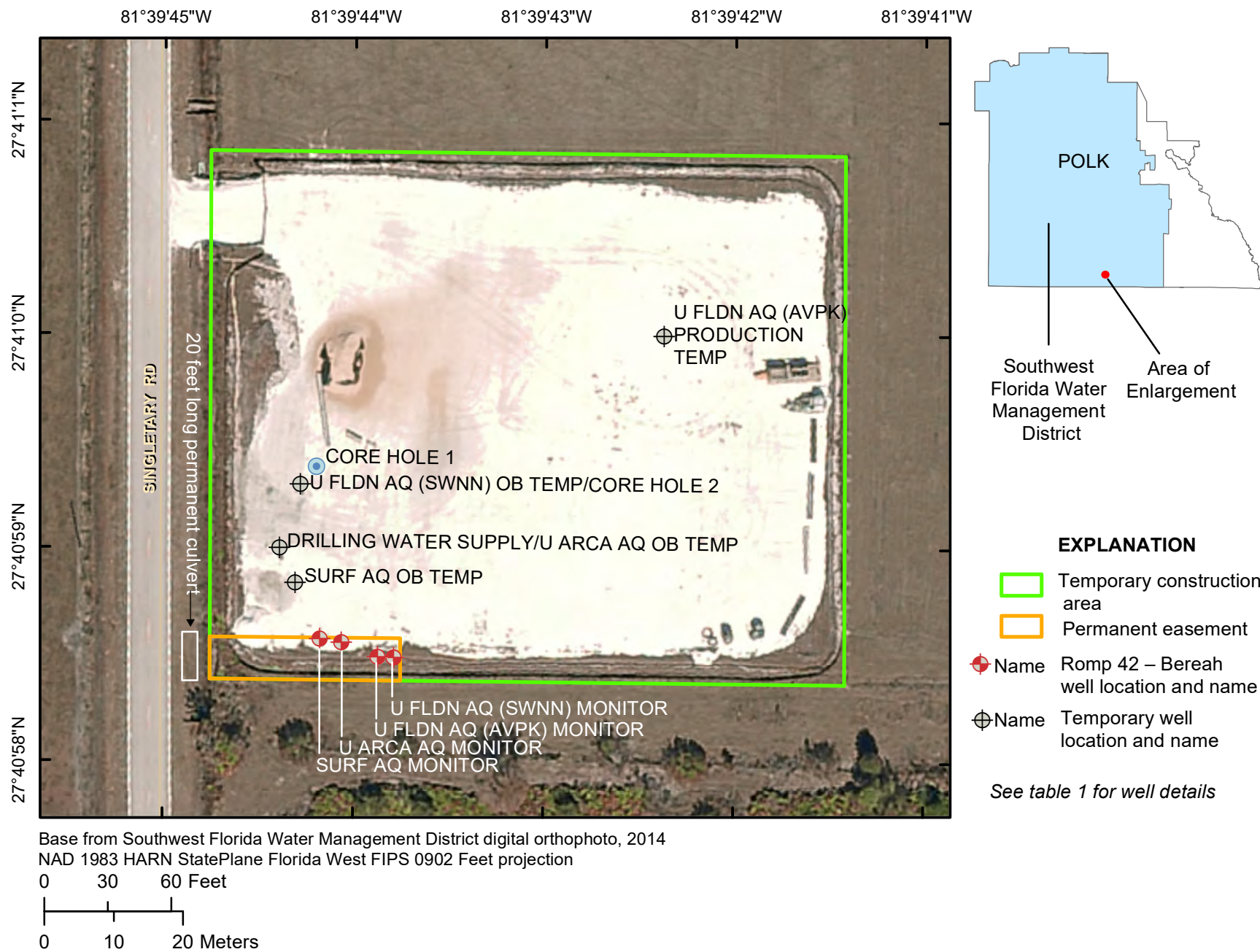
Figure 2. Well site layout for the ROMP 42 – Bereah well site in Polk County, Florida.
