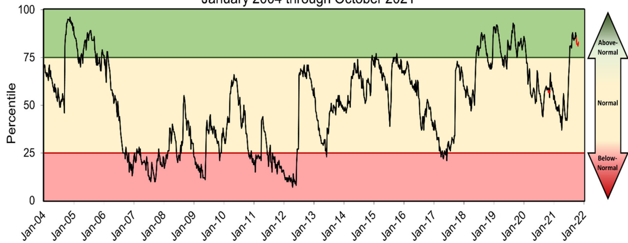
Groundwater Levels: Northern Counties January 2004 through October 2021
