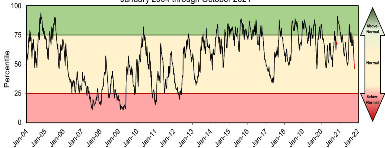
Groundwater Levels: Central Counties January 2004 through October 2021
