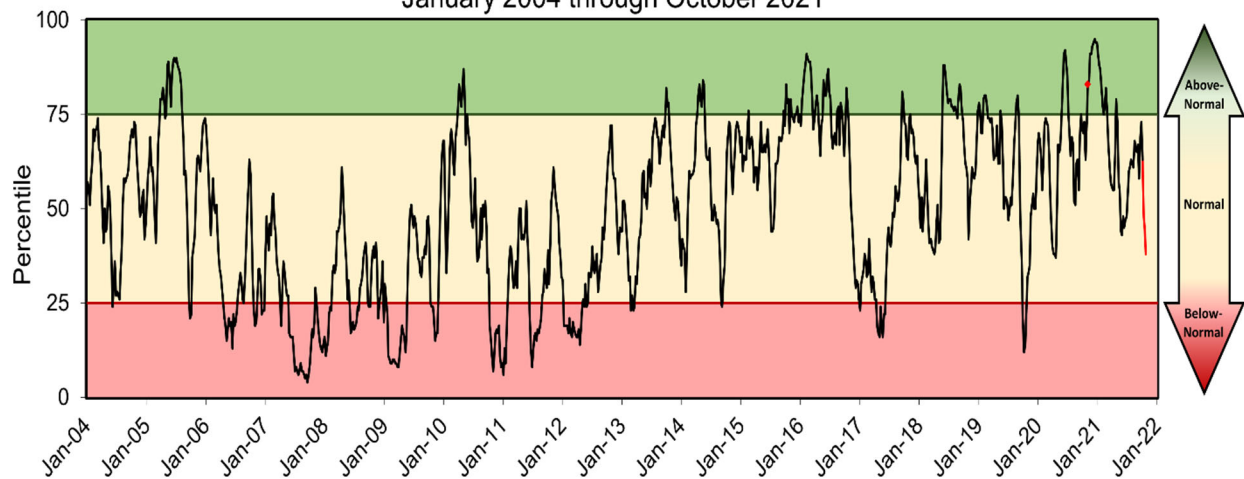
Groundwater Levels: Southern Counties January 2004 through October 2021
