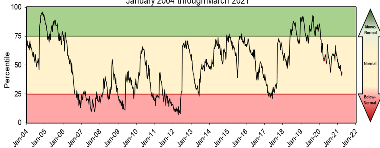
Groundwater Levels: Northern Counties January 2004 through March 2021
