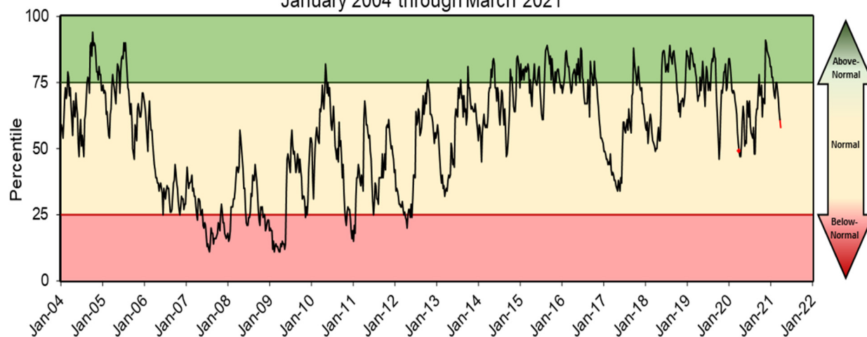
Groundwater Levels: Central Counties January 2004 through March 2021
