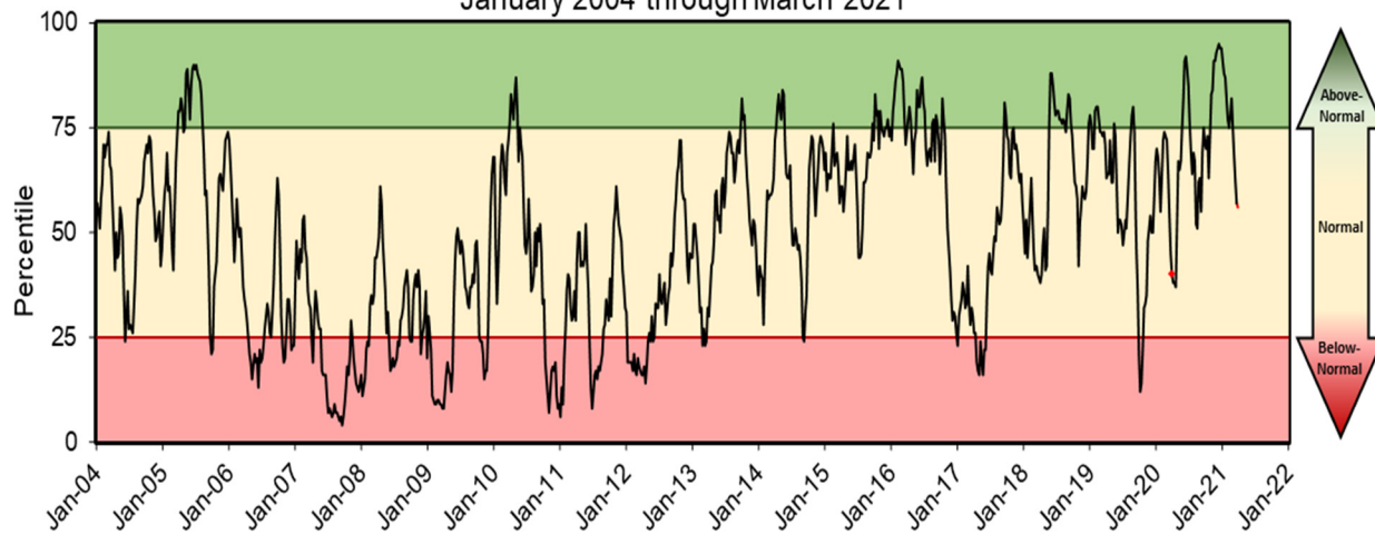
Groundwater Levels: Southern Counties January 2004 through March 2021
