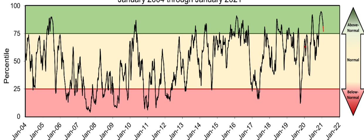
Groundwater Levels: Southern Counties January 2004 through January 2021
