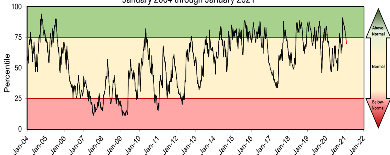
Groundwater Levels: Central Counties January 2004 through January 2021
