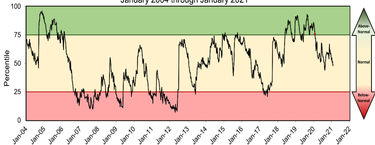
Groundwater Levels: Northern Counties January 2004 through January 2021
