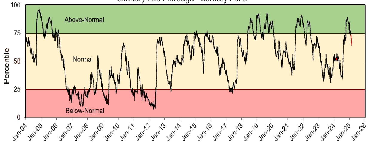
Groundwater Levels: Northern Counties January 2004 through February 2025
