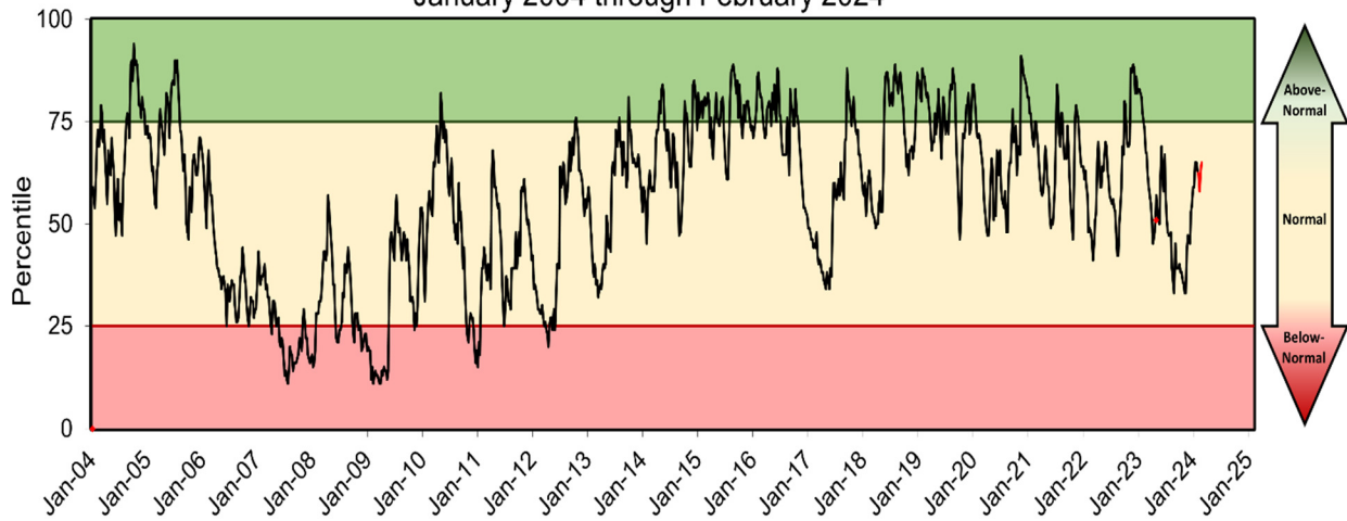
Groundwater Levels: Central Counties January 2004 through February 2024
