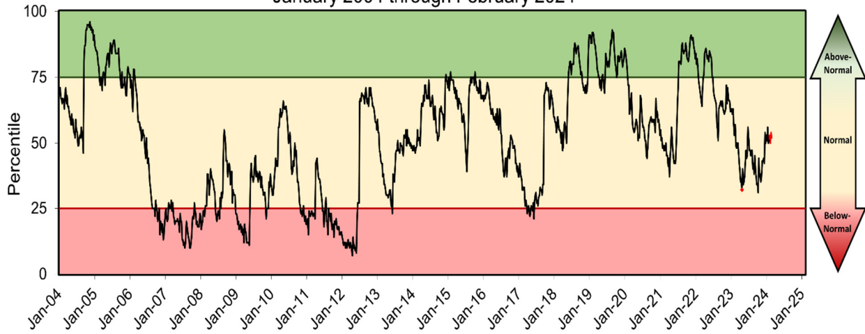
Groundwater Levels: Northern Counties January 2004 through February 2024
