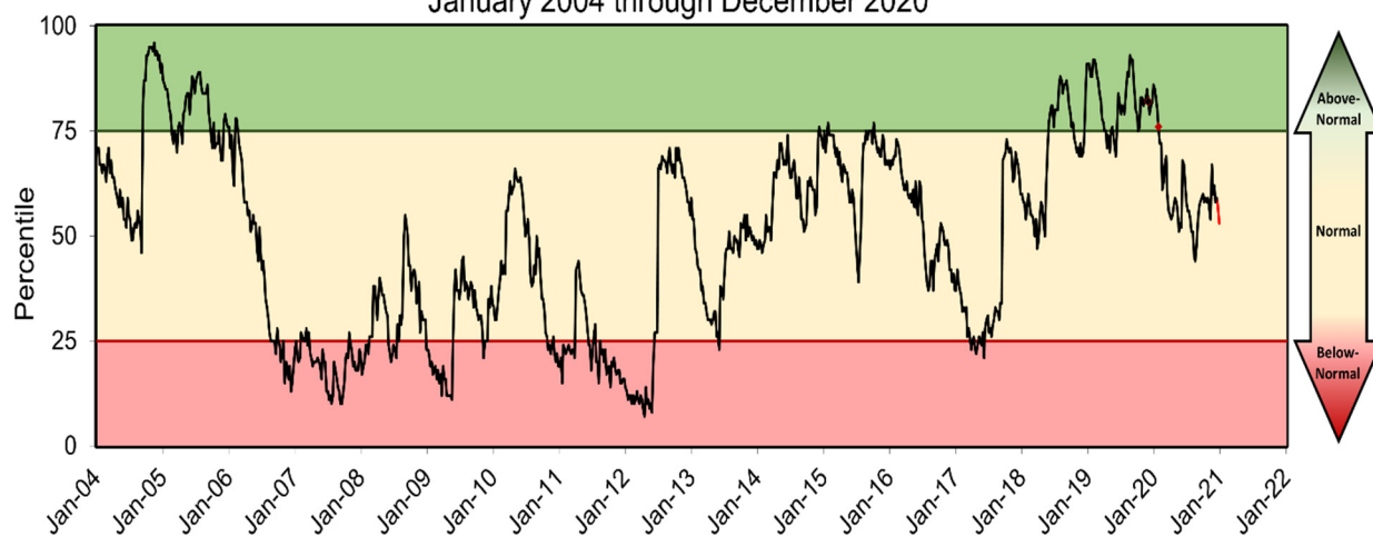
Groundwater Levels: Northern Counties January 2004 through December 2020
