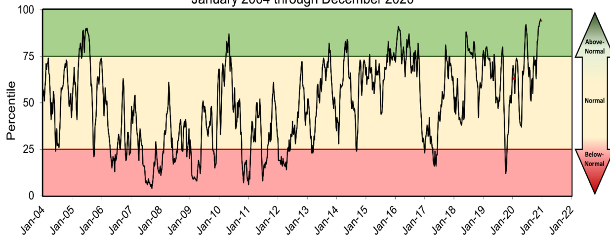
Groundwater Levels: Southern Counties January 2004 through December 2020
