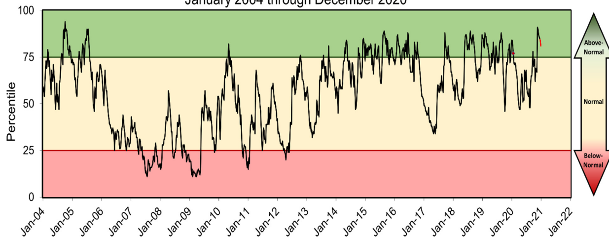
Groundwater Levels: Central Counties January 2004 through December 2020
