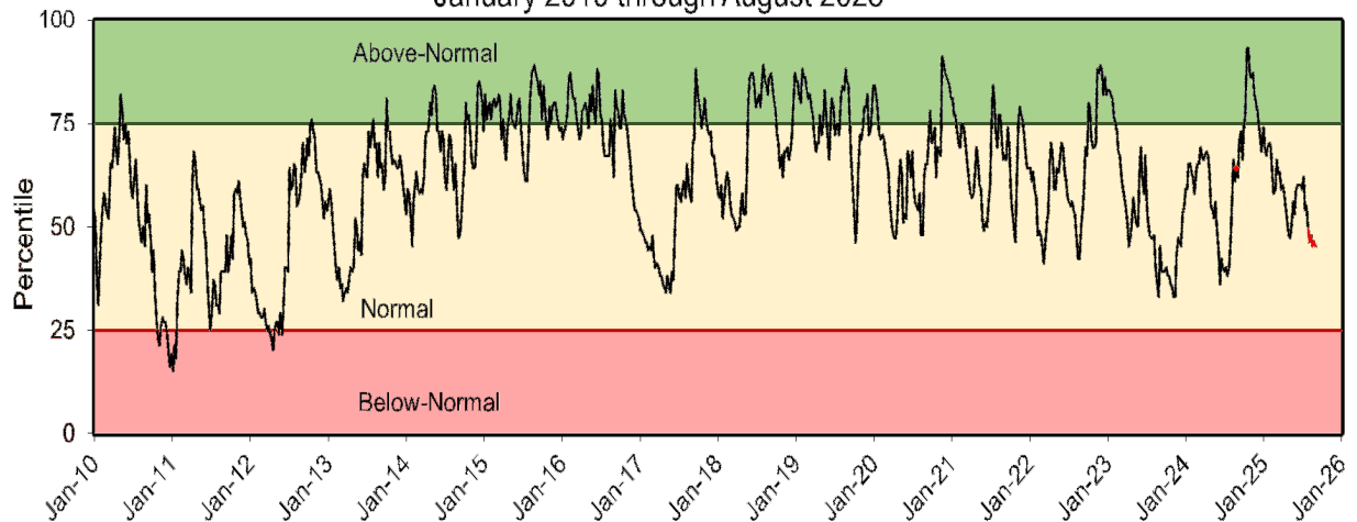
Groundwater Levels: Central Counties January 2010 through August 2025
