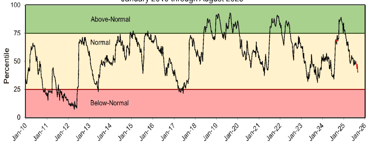
Groundwater Levels: Northern Counties January 2010 through August 2025
