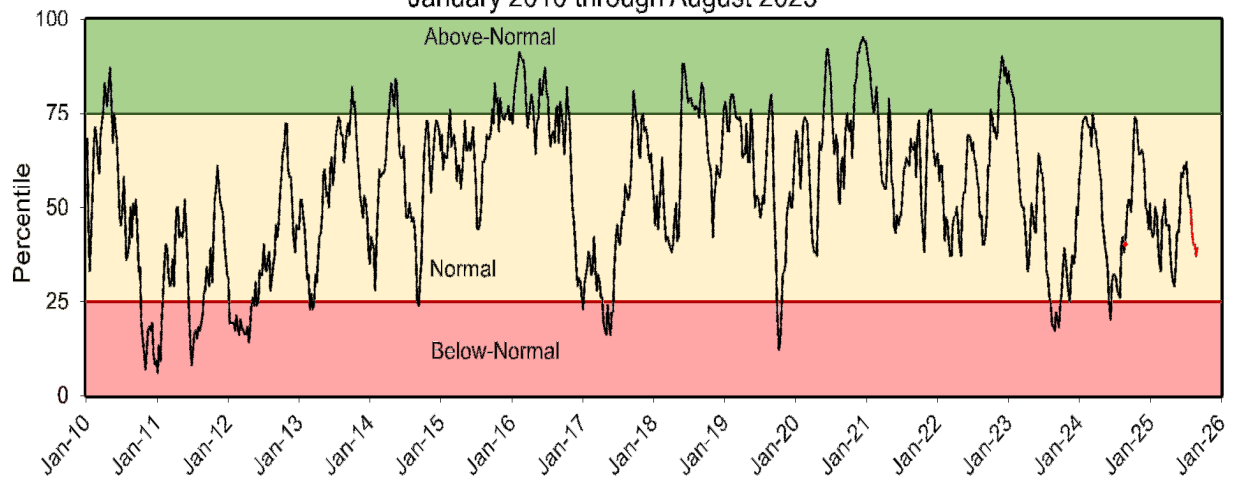
Groundwater Levels: Southern Counties January 2010 through August 2025
