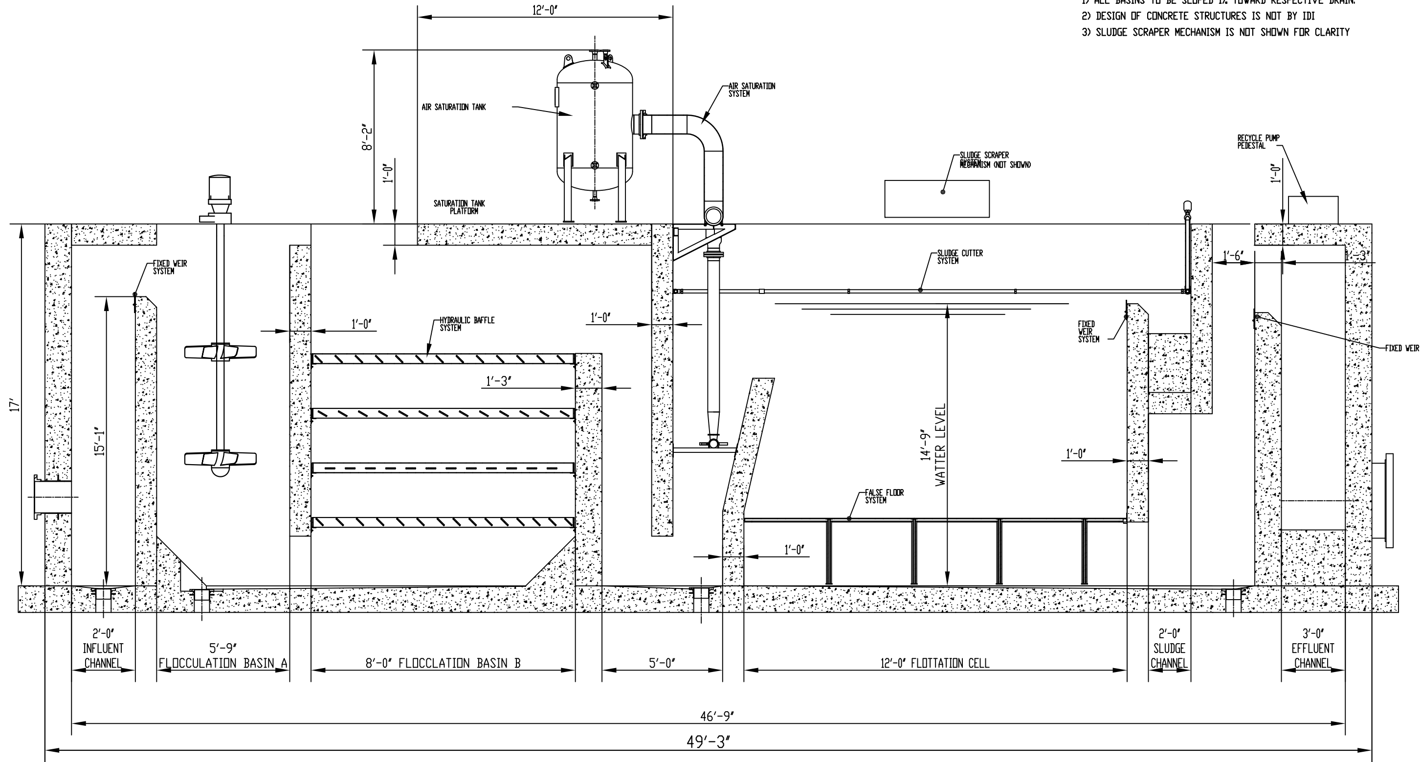
SECTION B-B
