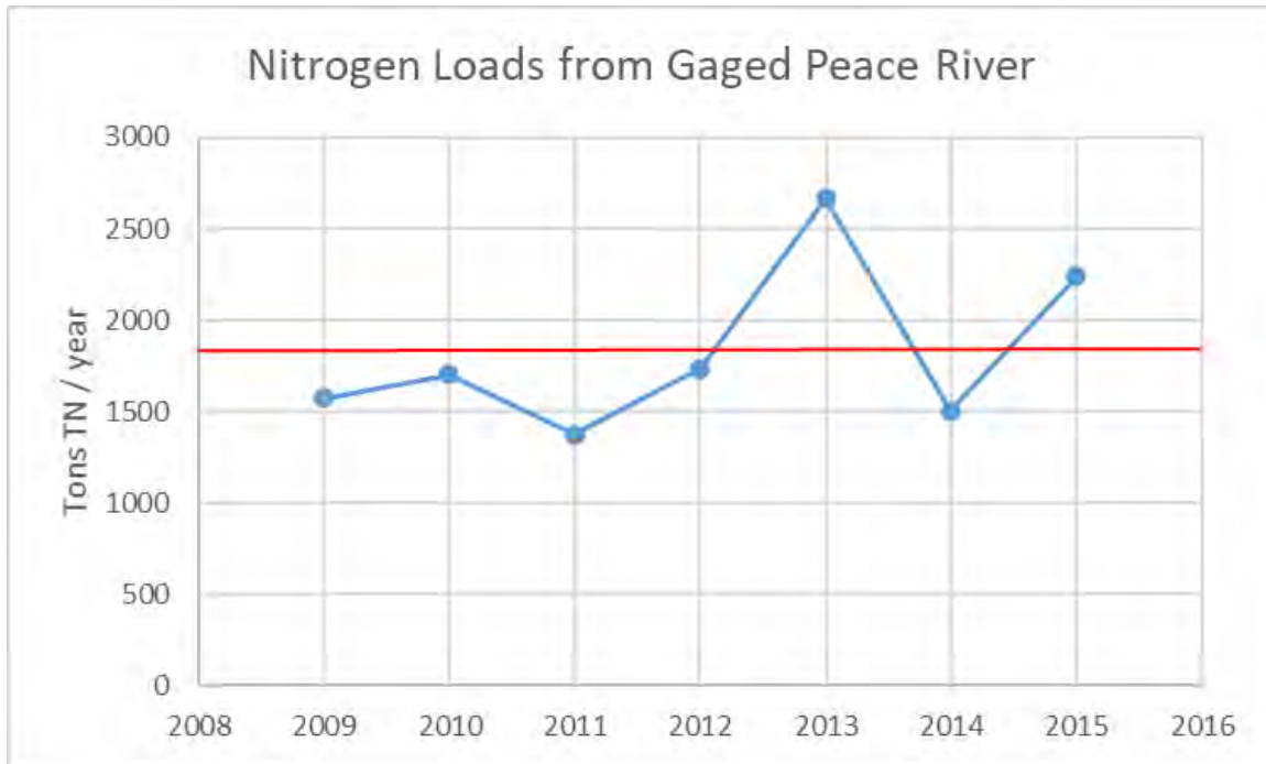
Figure 4 – Nitrogen loads, expressed as tons of TN per year, from the gaged Peace River watershed for the years 2009 to 2015. Red line represents average value for the years 1985 to 1992.
