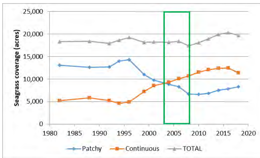
Figure 4 – Seagrass coverage in Charlotte Harbor. Values are in units of acres of patchy, continuous and total (patchy plus continuous) seagrass. The area in the green box indicates the reference period of 2003 to 2007.
