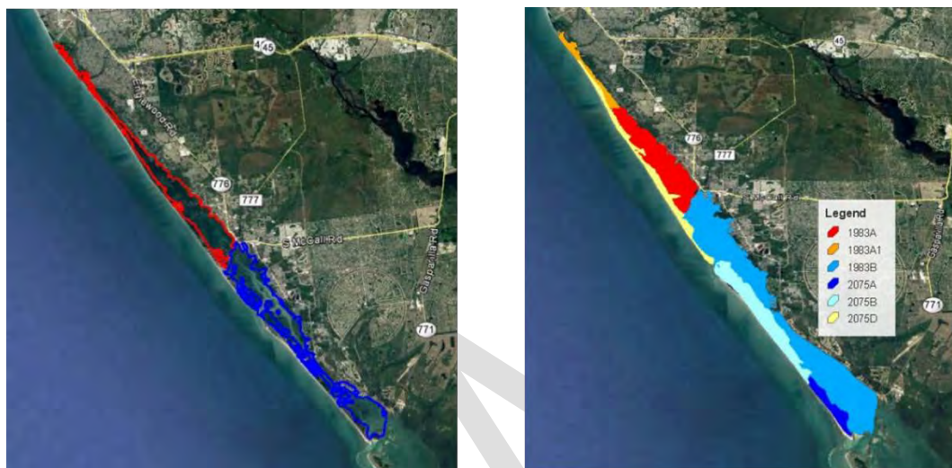
Figure 2 – Comparison of boundaries of regions from which NNC criteria were derived (left) vs. the boundaries of the WBIDs for which the NNC criteria were applied (right) for Charlotte Harbor.
