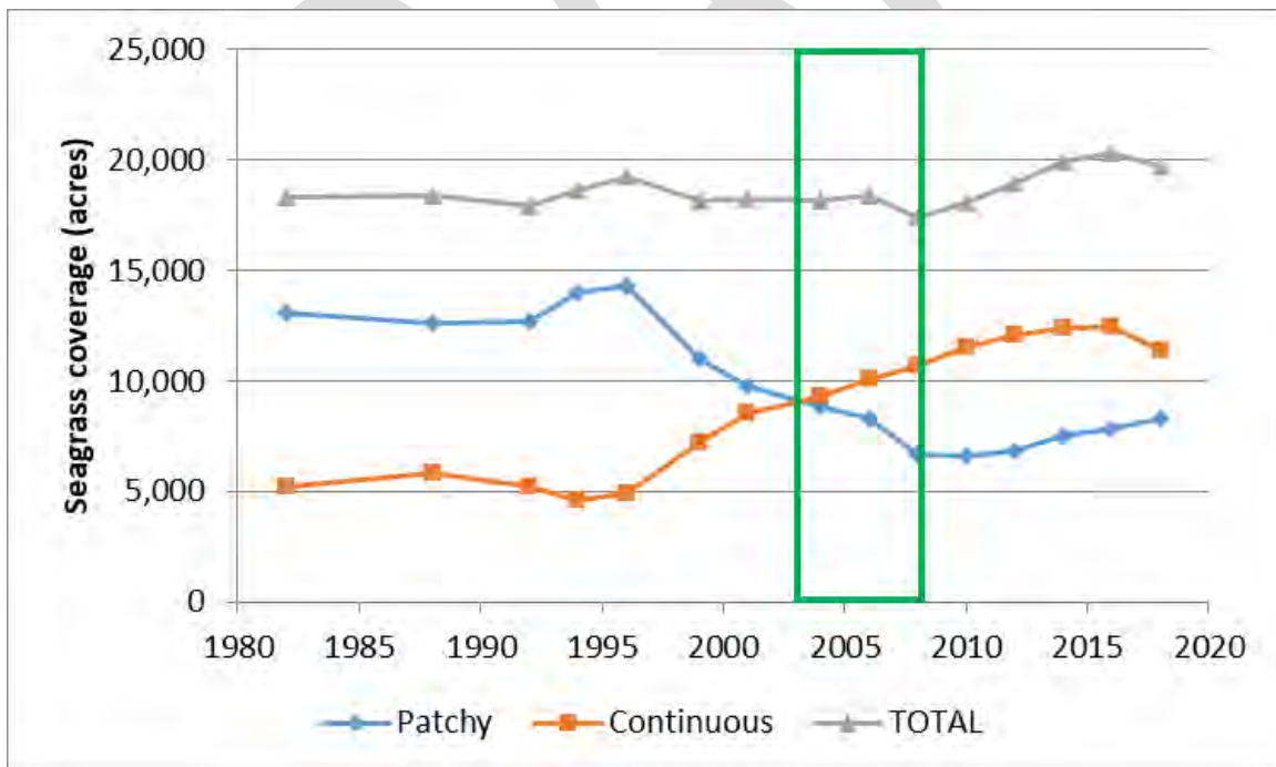
Figure 14 – Seagrass coverage in Charlotte Harbor. Values are in units of acres of patchy, continuous and total (patchy plus continuous) seagrass. The area in the green box indicates the reference period for the establishment of NNC criteria of 2003 to 2007.
