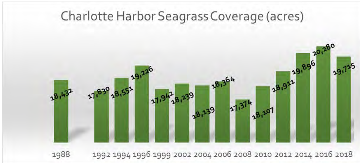
Figure 13 – Mapped seagrass acreage over time for Charlotte Harbor over the period of 1988 to 2018.
