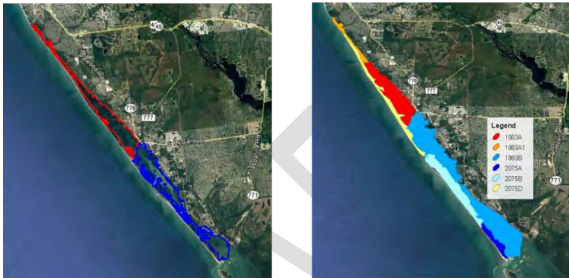
Figure 2 – Comparison of boundaries of regions from which NNC criteria were derived (left) vs. the boundaries of the WBIDs for which the NNC criteria were applied (right) for Lemon Bay.
