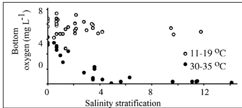
Figure 1 – Relationship between salinity stratification (difference in salinity in surface vs. bottom waters) and the amount of oxygen in the bottom waters of Charlotte Harbor in warm vs. cool temperature conditions (from Figure 5 in Turner et al. 2006).
