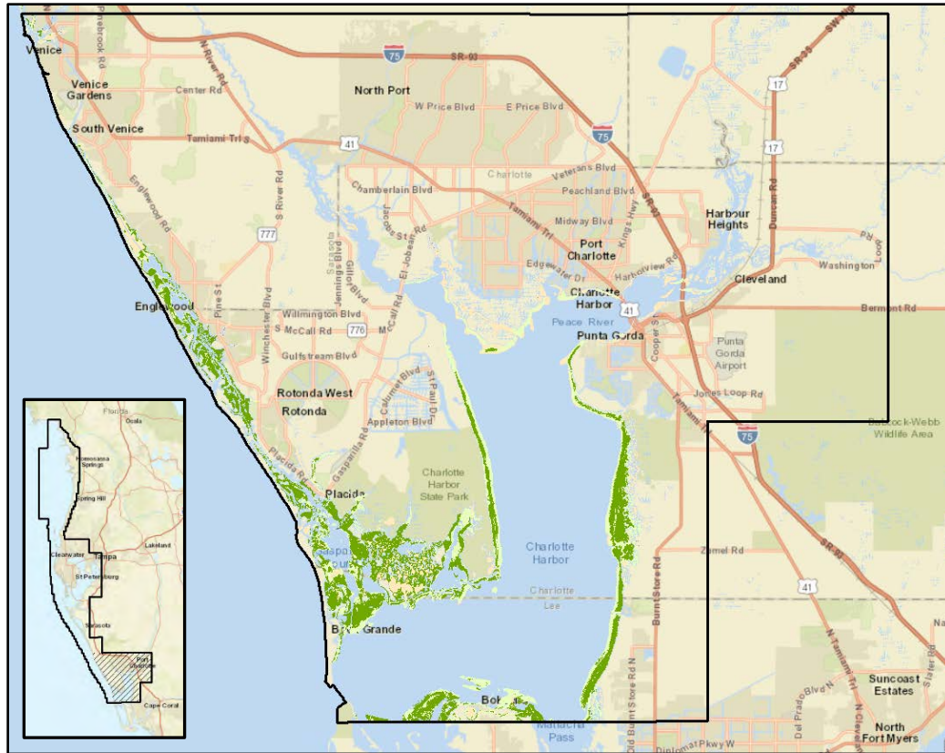
Figure 11 – Boundary of the Charlotte Harbor and Lemon Bay portion of the SWFWMD Biennial Seagrass Mapping Project. Dona & Roberts Bay falls within the northern edge of the Lemon Bay seagrass mapping boundary. Shaded green areas represent the extent of seagrass meadows mapped in 2018.
