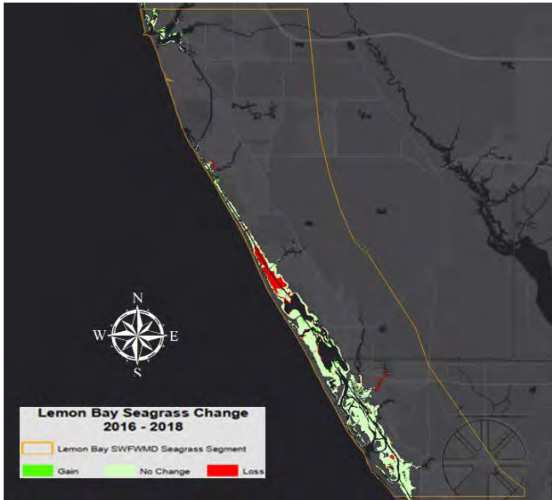
Figure 17 – Spatial distribution of gains, losses and areas with stable seagrass coverage in Lemon Bay between 2016 and 2018. GIS data from SWFWMD.
