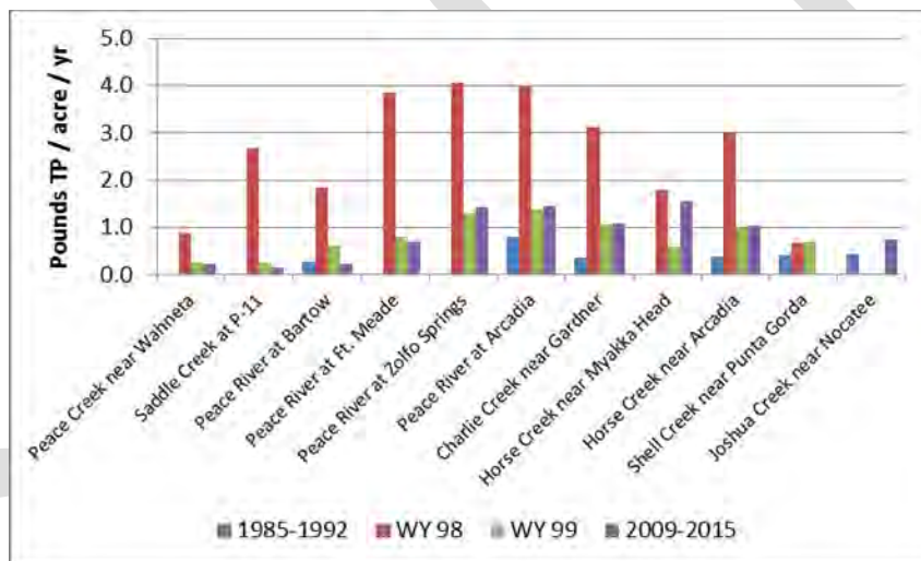
Figure 11 – Area normalized TP loads for the Peace River watershed by gaged location. Values are in units of pounds of TP per acre per year. Gaged locations are arrayed along the x-axis from upstream to downstream within the watershed.
