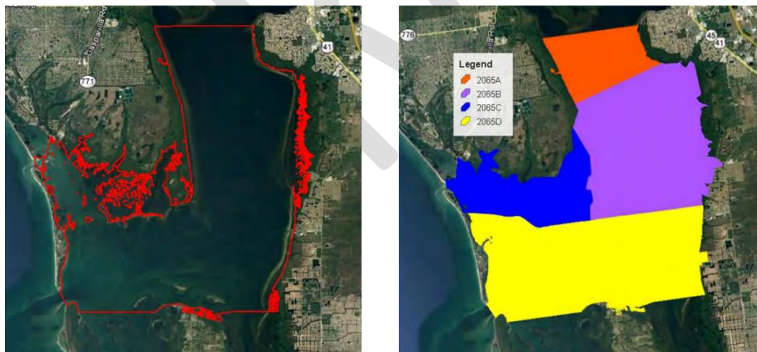
Figure 2 – Comparison of boundaries of regions from which NNC criteria were derived (left) vs. the boundaries of the WBIDs for which the NNC criteria were applied (right) for Charlotte Harbor.
