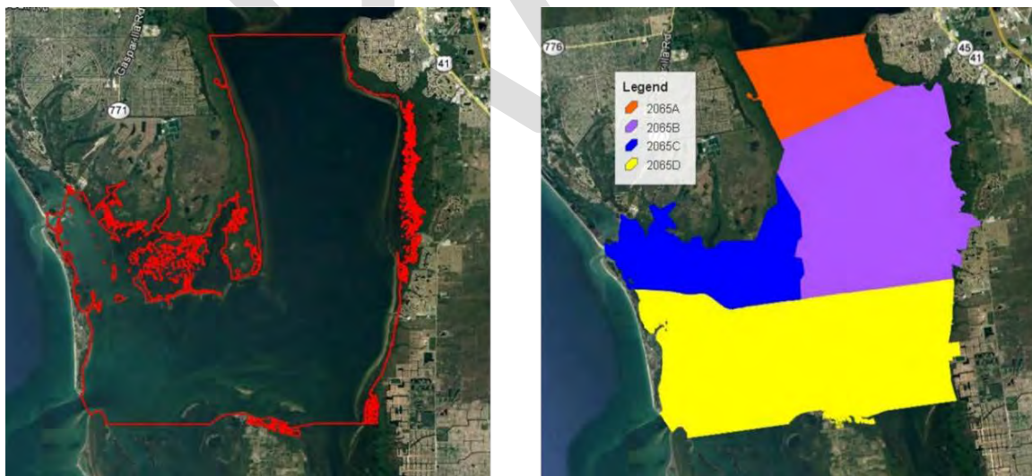
Figure 3 – Comparison of boundaries of regions from which NNC criteria were derived (left) vs. the boundaries of the WBIDs for which the NNC criteria were applied (right) for Charlotte Harbor.
