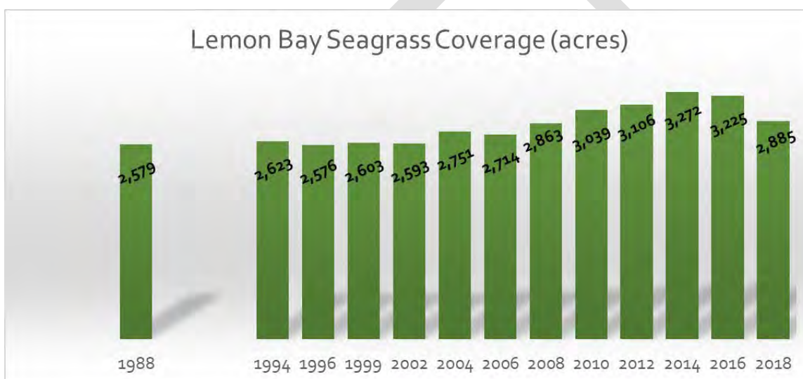
Figure 15 – Mapped seagrass acreage over time for Lemon Bay over the period of 1988 to 2018. Data include Dona & Roberts Bay.
