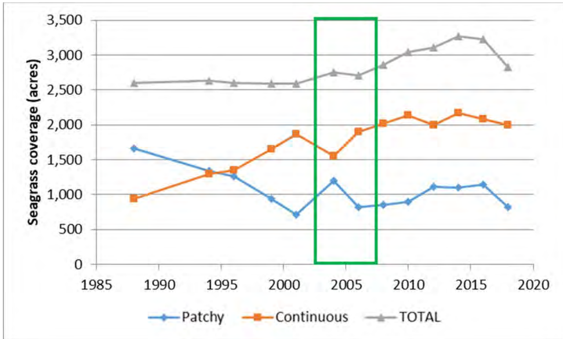
Figure 16 – Seagrass coverage in Lemon Bay. Values are in units of acres of patchy, continuous and total (patchy plus continuous) seagrass. The area in the green box indicates the reference period for the establishment of NNC criteria of 2003 to 2007.
