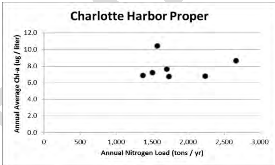
Figure 6 – Annual TN load from the gaged Peace River plotted against annual average chlorophyll-a concentrations for the Charlotte Harbor Numeric Nutrient Concentration (NNC) region.
