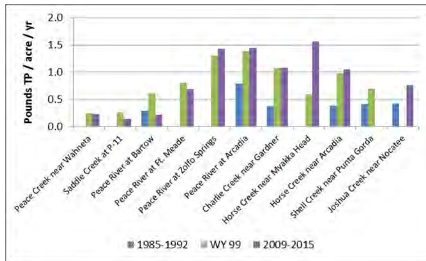
Figure 12– Area normalized TP loads for the Peace River watershed by gaged location, without results from WY 1998. Values are in units of pounds of TP per acre per year. Gaged locations are arrayed along the x-axis from upstream to downstream within the watershed.
