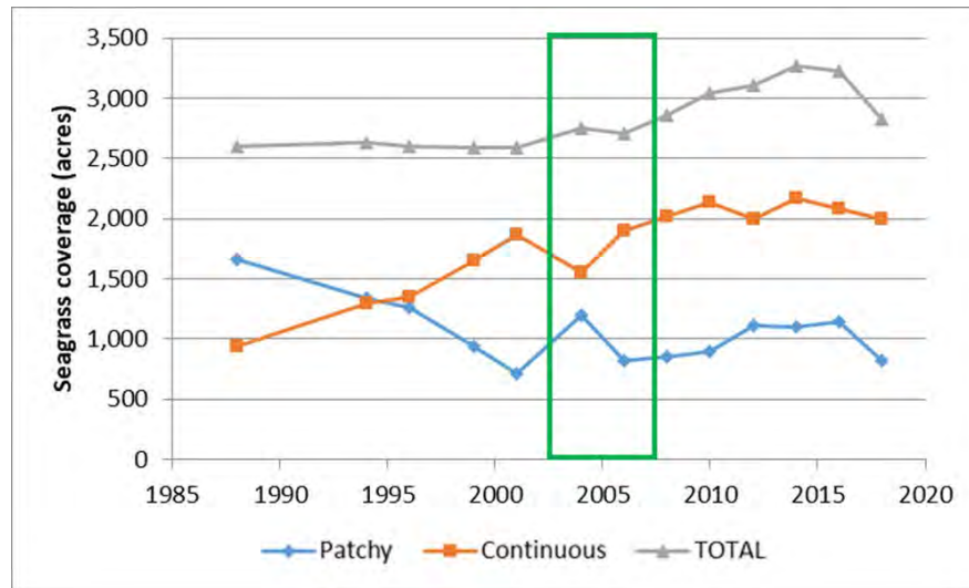
Figure 5 – Seagrass coverage in Lemon Bay. Values are in units of acres of patchy, continuous and total (patchy plus continuous) seagrass meadows. The area in the green box indicates the reference period of 2003 to 2007.
