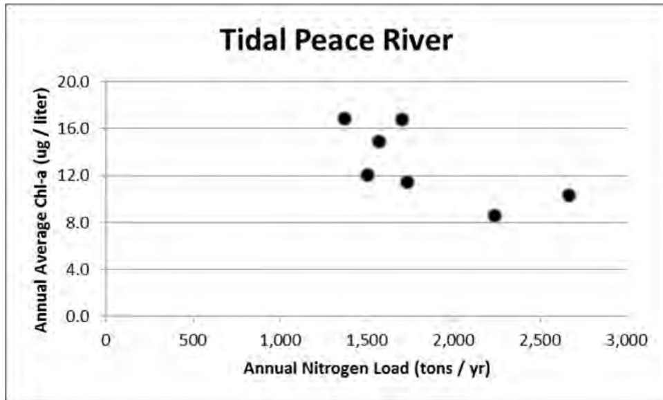
Figure 5 – Annual TN load from the gaged Peace River plotted against annual average chlorophyll-a concentrations for the Tidal Peace River Numeric Nutrient Concentration (NNC) region.
