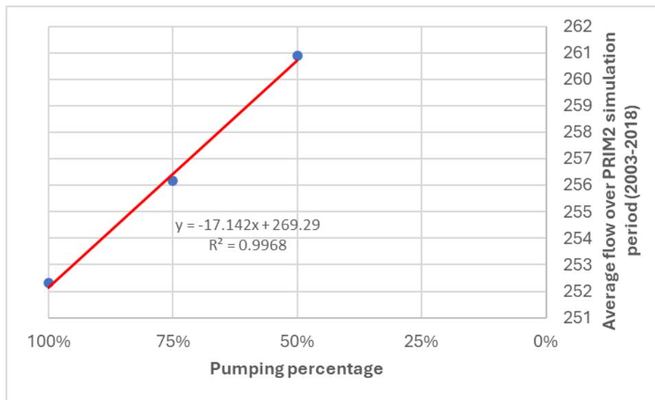
Figure 3. Average flow over the simulation period (2003-2018) versus pumping rates.
