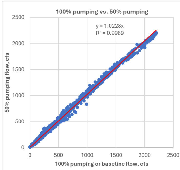
Figure 2. Comparison of simulated daily flow under the 100% pumping scenario versus the 50% pumping scenario.
