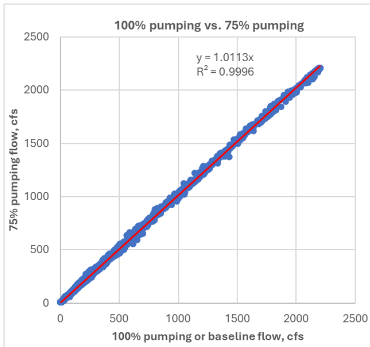
Figure 1. Comparison of simulated daily flow under the 100% pumping scenario versus the 75% pumping scenario.
