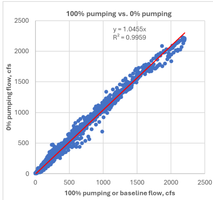
Figure 4. Comparison of simulated daily flow under the 100% pumping scenario versus the extrapolated daily flow under the 0% pumping scenario.
