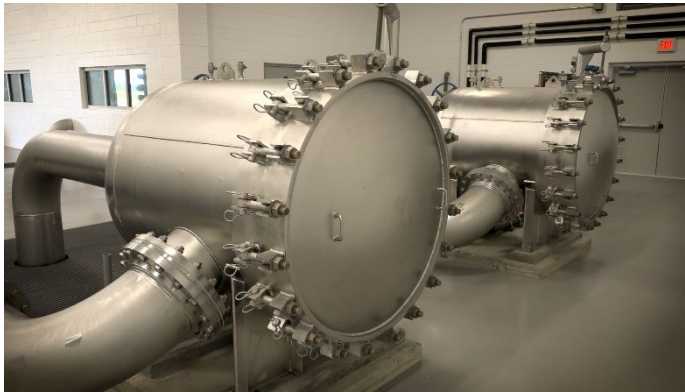
City of Punta Gorda reverse osmosis water production facility.
