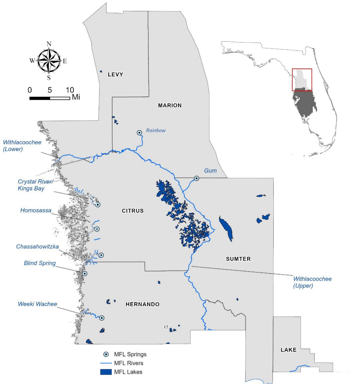
Figure 2-2. Minimum flows and levels priority water resources in the Northern Planning Region
