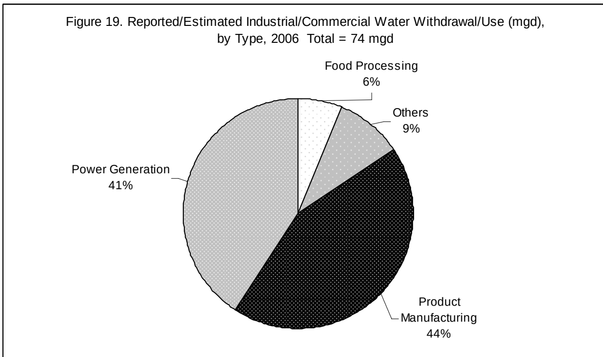
Figure 19. Reported/Estimated Industrial/Commercial Water Withdrawal/Use (mgd), by Category 2006
