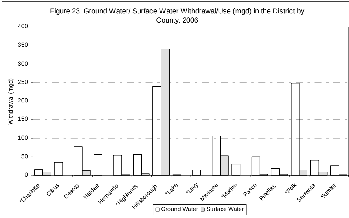
Figure 23. Ground Water/Surface Water Withdrawal/Use (mgd) in the District by County, 2006
