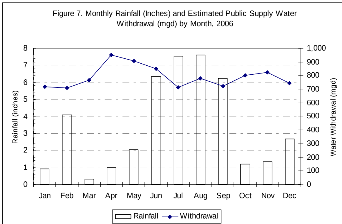
Figure 7. Average Rainfall (inches) and Estimated Public Supply Water Use (mgd), 2006
