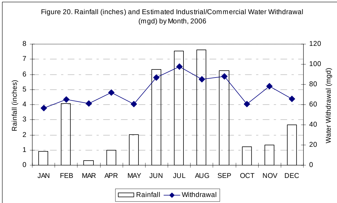
Figure 20. Rainfall (inches) and Estimated Industrial/Commercial Water Withdrawal/Use (mgd) by Month, 2006
