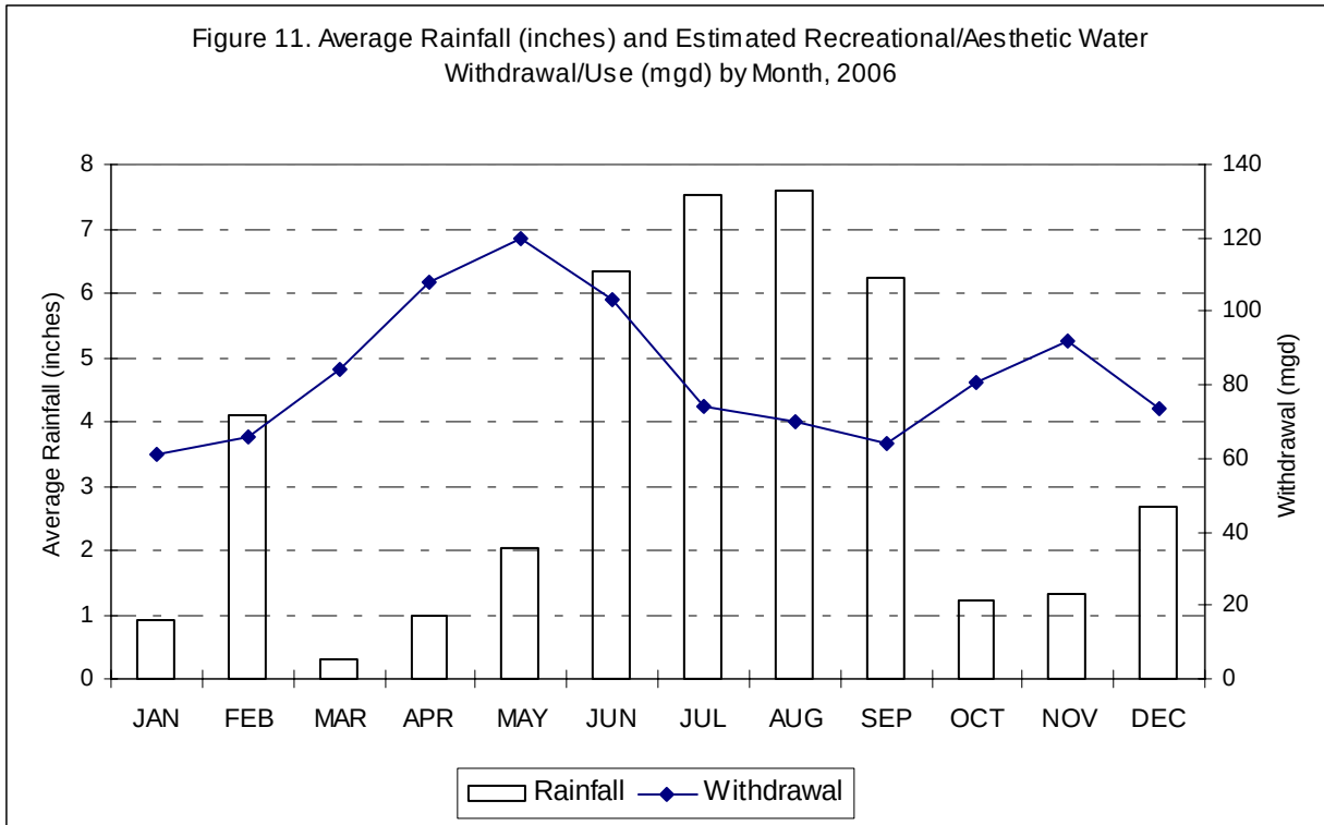
Figure 11. Average Rainfall (inches) and Estimated Recreational/Aesthetic Water Withdrawal/Use (mgd) by Month, 2006
