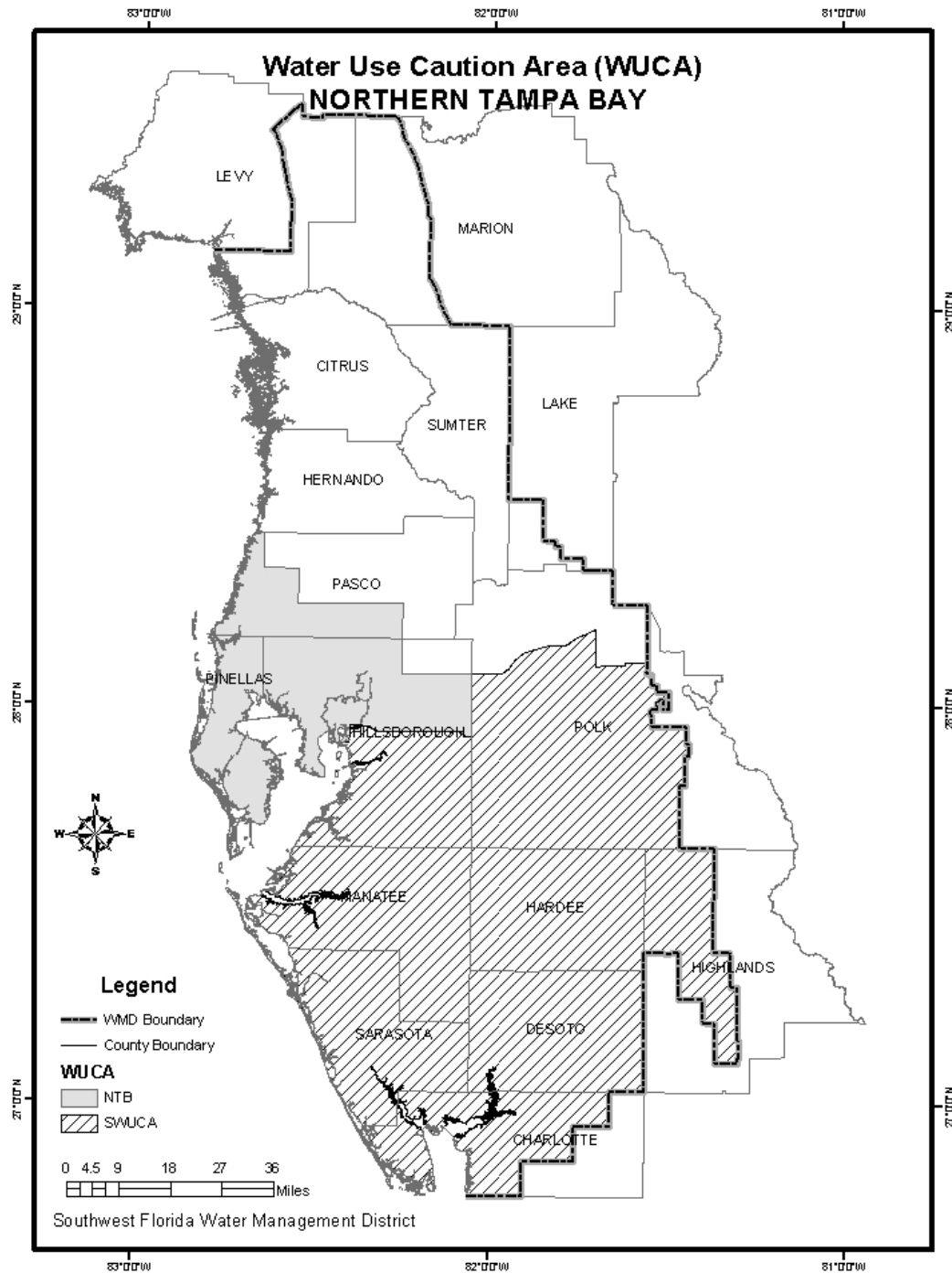
Figure 3. Northern Tampa Bay Water Use Caution Area (NTBWUCA)
