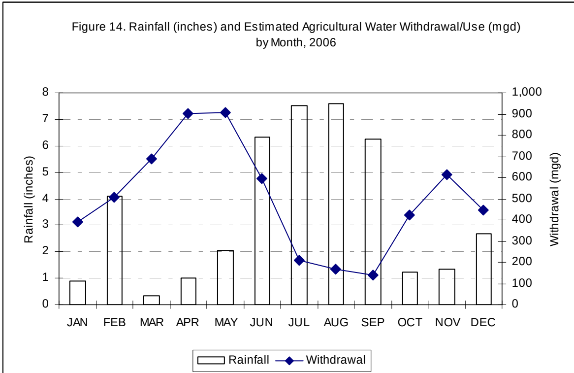
Figure 14. Average Rainfall (inches) and Estimated Agricultural Water Withdrawal/Use (mgd) by Month, 2006
