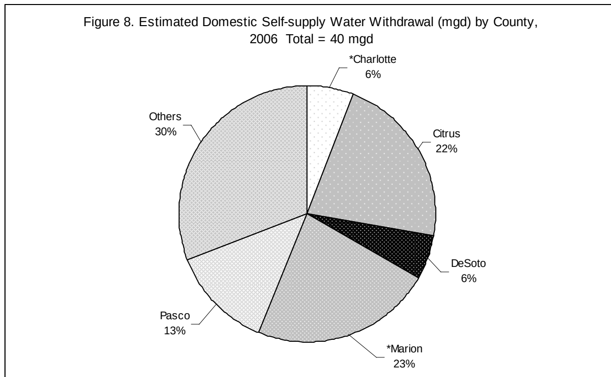
Figure 8. Estimated Domestic Self-supply Water Withdrawal (mgd), by County, 2006
