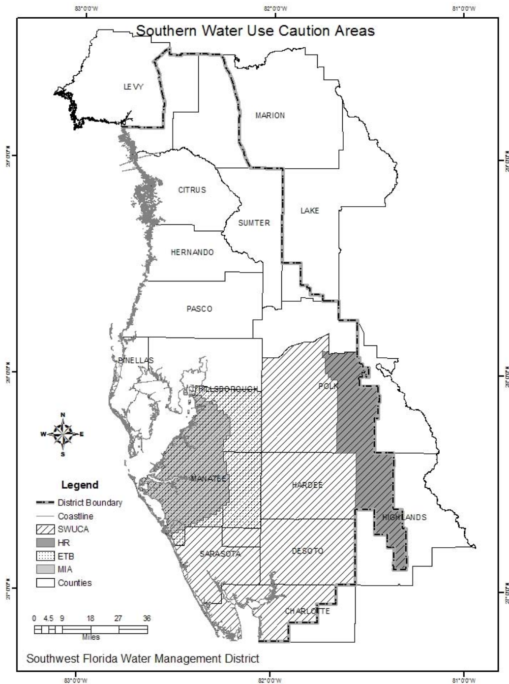
Figure 4. Southern Water Use Caution Areas (SWUCA)
