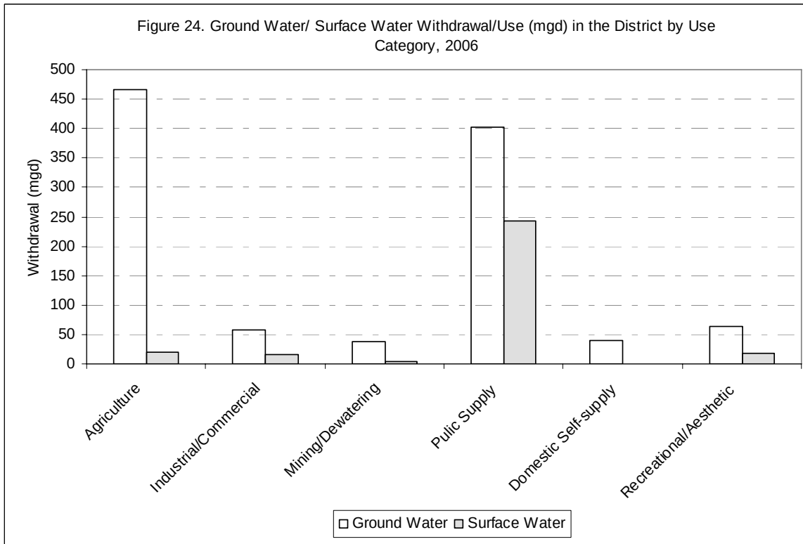
Figure 24. Ground Water/Surface Water Withdrawal/Use (mgd) in the District by Use Category, 2006
