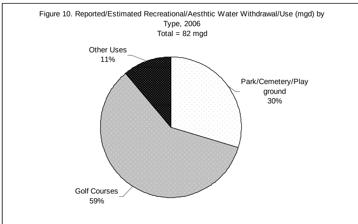
Figure 10. Reported/Estimated Recreational/Aesthetic Water Withdrawal/Use (mgd) by Type, 2006
