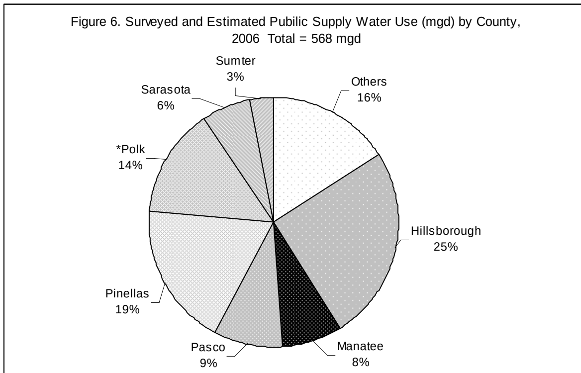
Figure 6. Surveyed and Estimated Public Supply Water Use (mgd) by County, 2006
