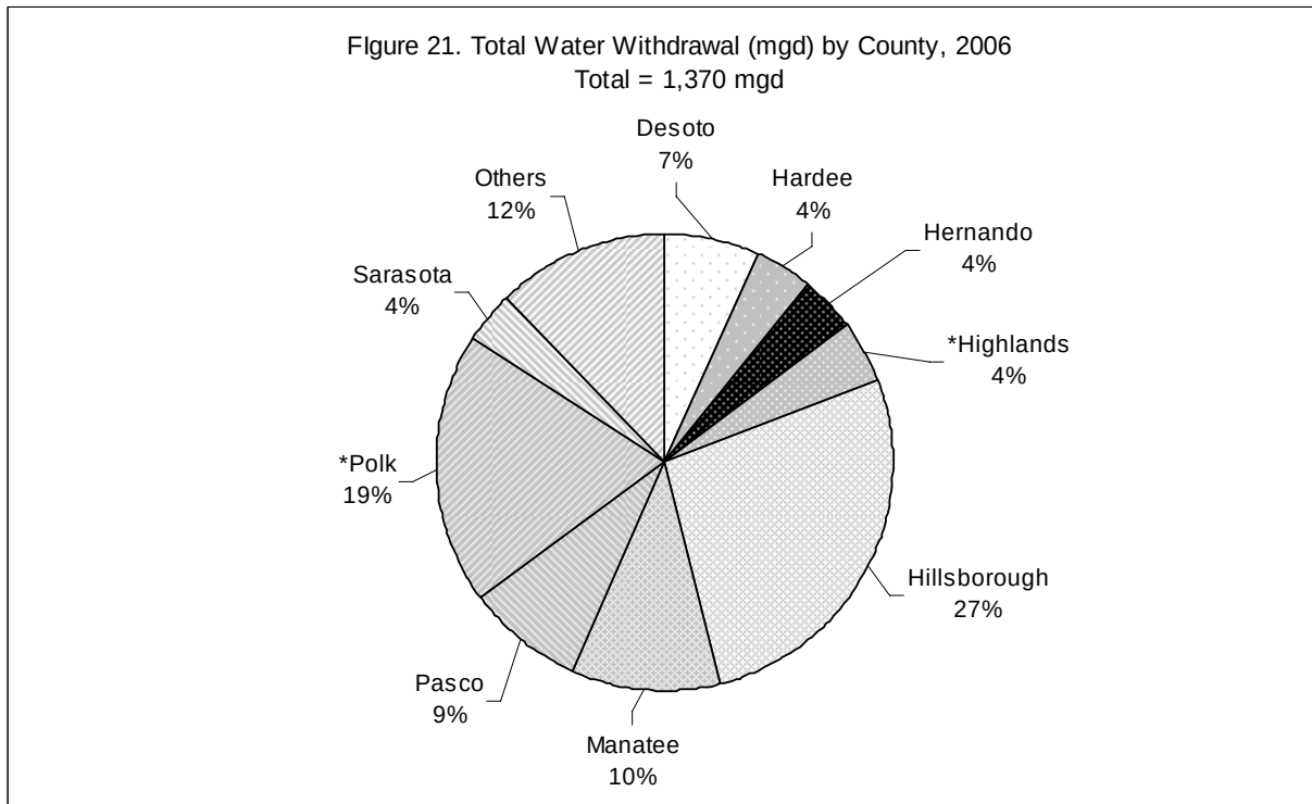
Figure 21. Total Water Withdrawal (mgd) by County, 2006
