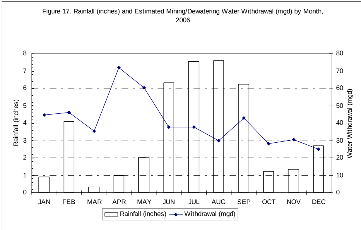
Figure 17. Average Rainfall (inches) and Estimated Mining/Dewater Water Withdrawal (mgd) by Month, 2006
