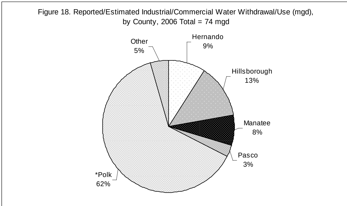
Figure 18. Reported/Estimated Industrial/Commercial Water Withdrawal/Use (mgd) by County, 2006
