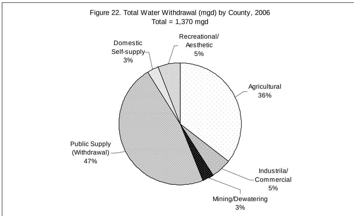
Figure 22. Total Water Withdrawal (mgd), by Use Category, 2006
