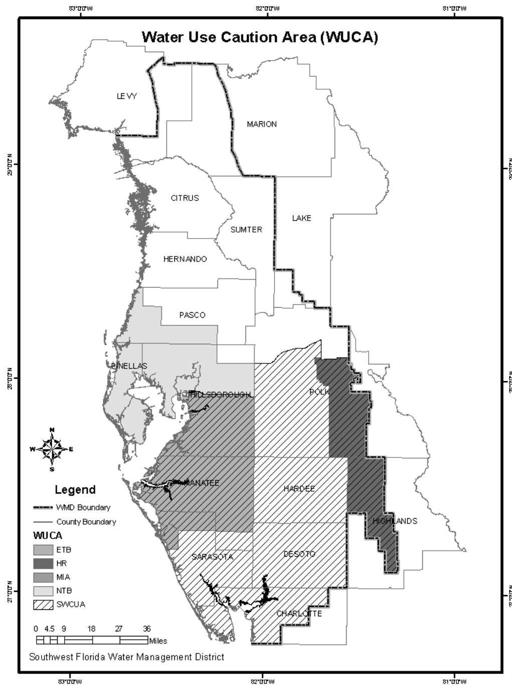
Figure 2. Water Use Caution Areas (WUCAs)
