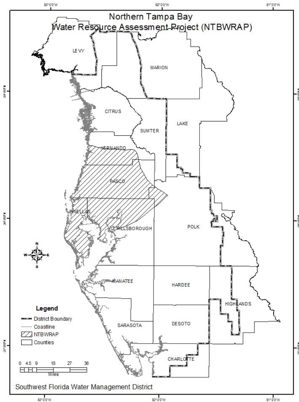
Figure 5. Northern Tampa Bay Water Resource Assessment Project Area, 2006
