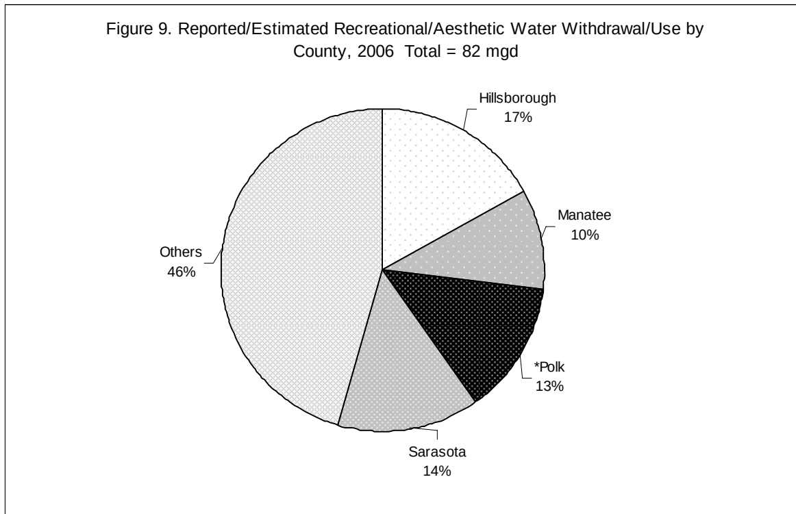
Figure 9. Reported /Estimated Recreational/Aesthetic Water Withdrawal/Use (mgd), by County, 2006
