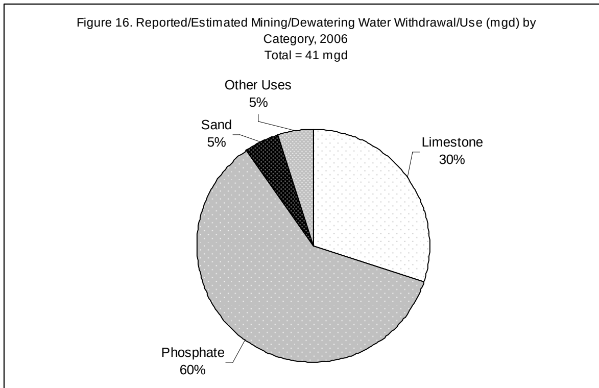
Figure 16. Reported/Estimated Mining/Dewatering Water Withdrawal/Use (mgd) by Category, 2006
