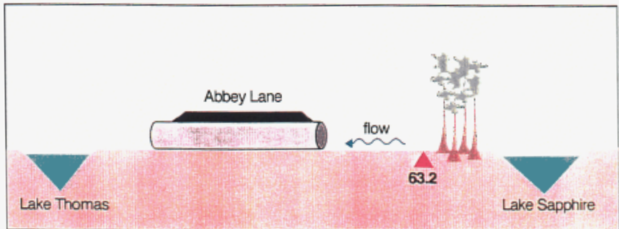
Profile of Outlet Conveyance System
