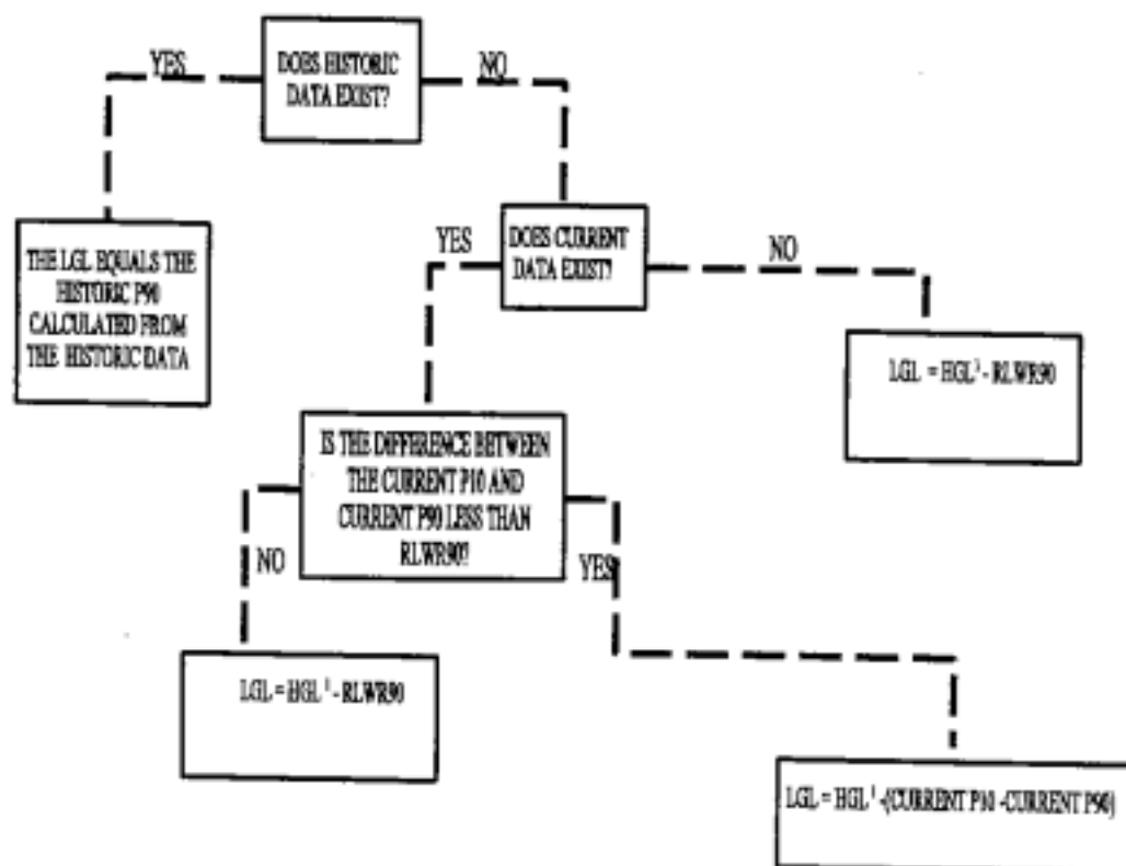
Figure 16 : METHOD FOR CALCULATION OF THE LOW GUIDANCE LEVEL (LGL)
