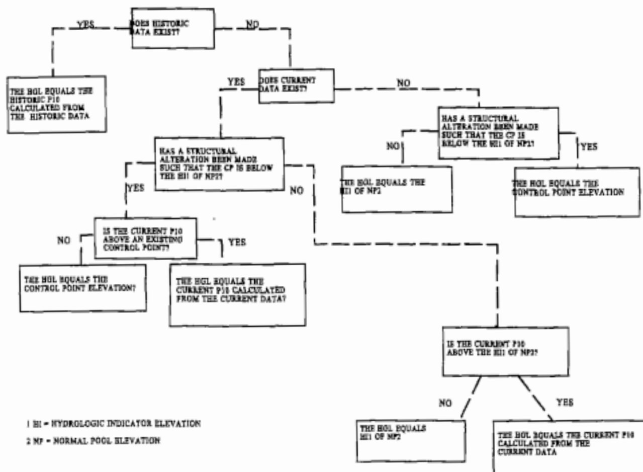
Figure 13 : METHOD FOR CALCULATION OF THE HIGH GUIDANCE LEVEL (HGL)
