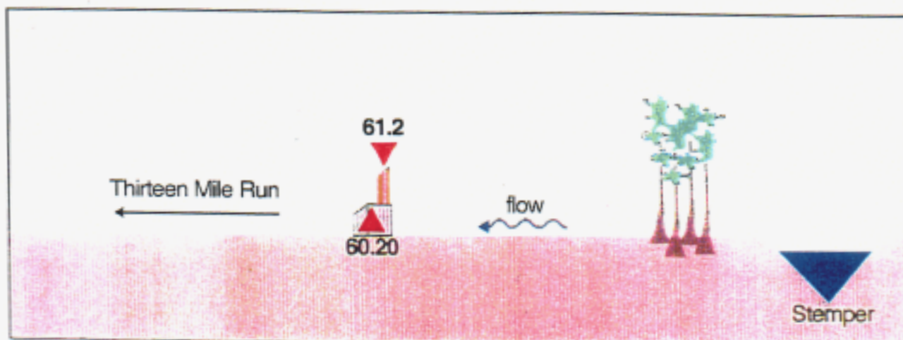
Profile of Outlet Conveyance System
