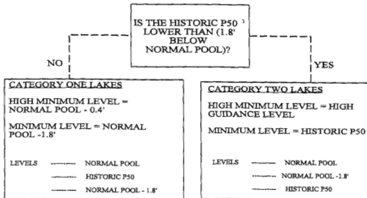
Figure 15 : METHOD FOR CALCULATION OF HIGH MINIMUM AND MINIMUM LAKE LEVELS
