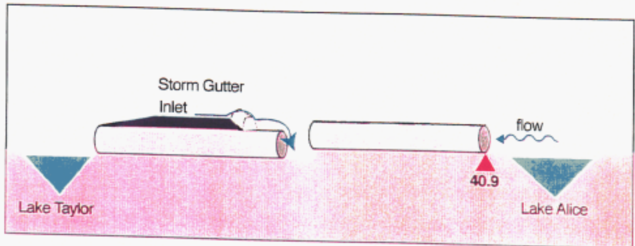
Profile of Outlet Conveyance System
