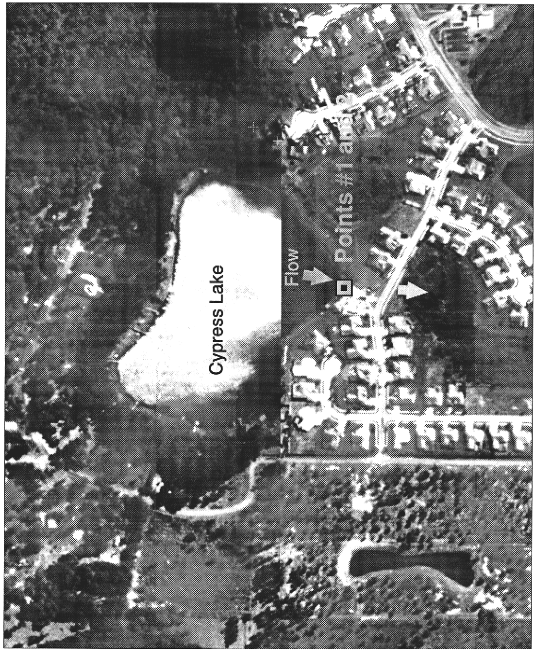
Figure 6-26. Outlet conveyance system for Cypress Lake, Hillsborough County, Florida. Numbered sites are described in Table 6-23.
