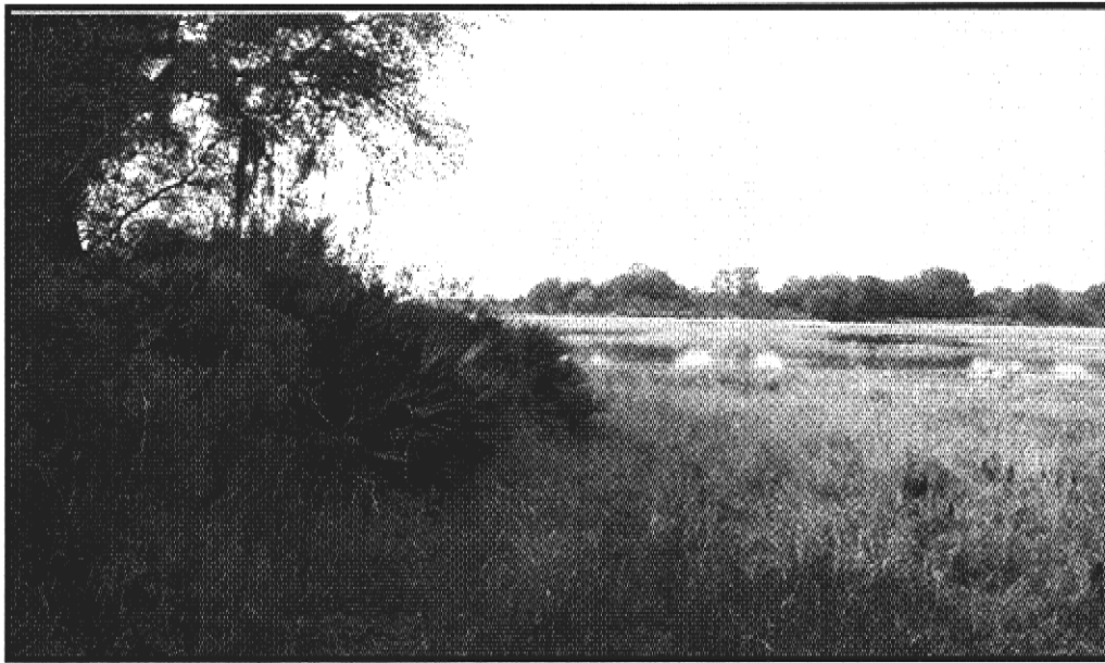
Figure 2-1. Vegetation in lake basins may provide some indication of high lake levels. Panel A shows the saw palmetto ( Serenoa repens ) line at Big Fish Lake in Pasco County, Florida. Panel B shows buttressed trunks of cypress ( Taxodium sp.) trees at Worrell (Bass) Lake in Pasco County, Florida.
