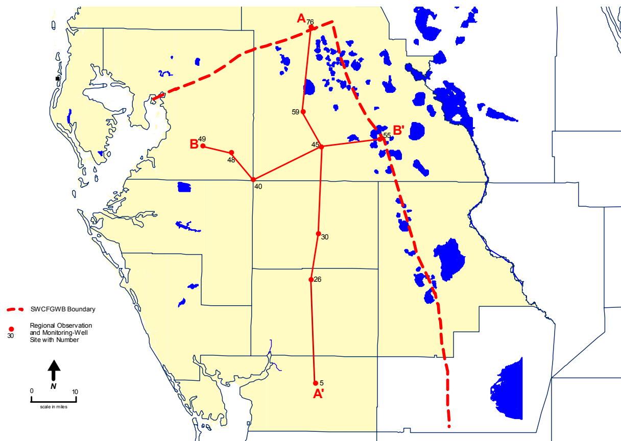
Figure 2. Location of hydrostratigraphic cross-sections A-A' and B-B'.
