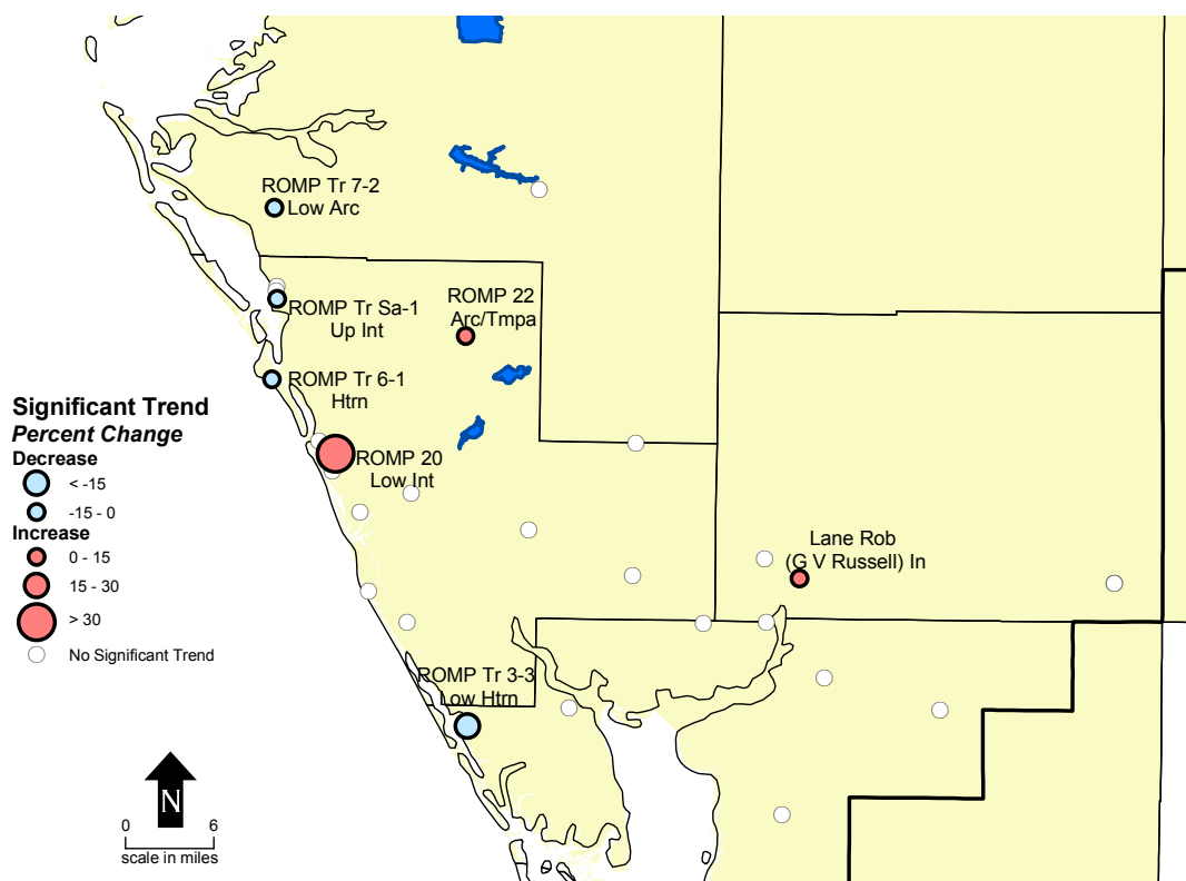
Figure 44. Chloride/Sulfate Ratio Trends in PZ 3.
