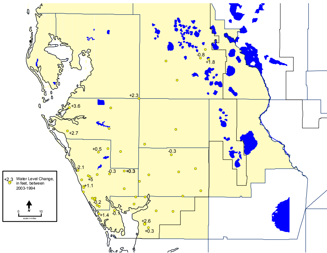
Figure 28. PZ 2 water level change from 1994-2003.
