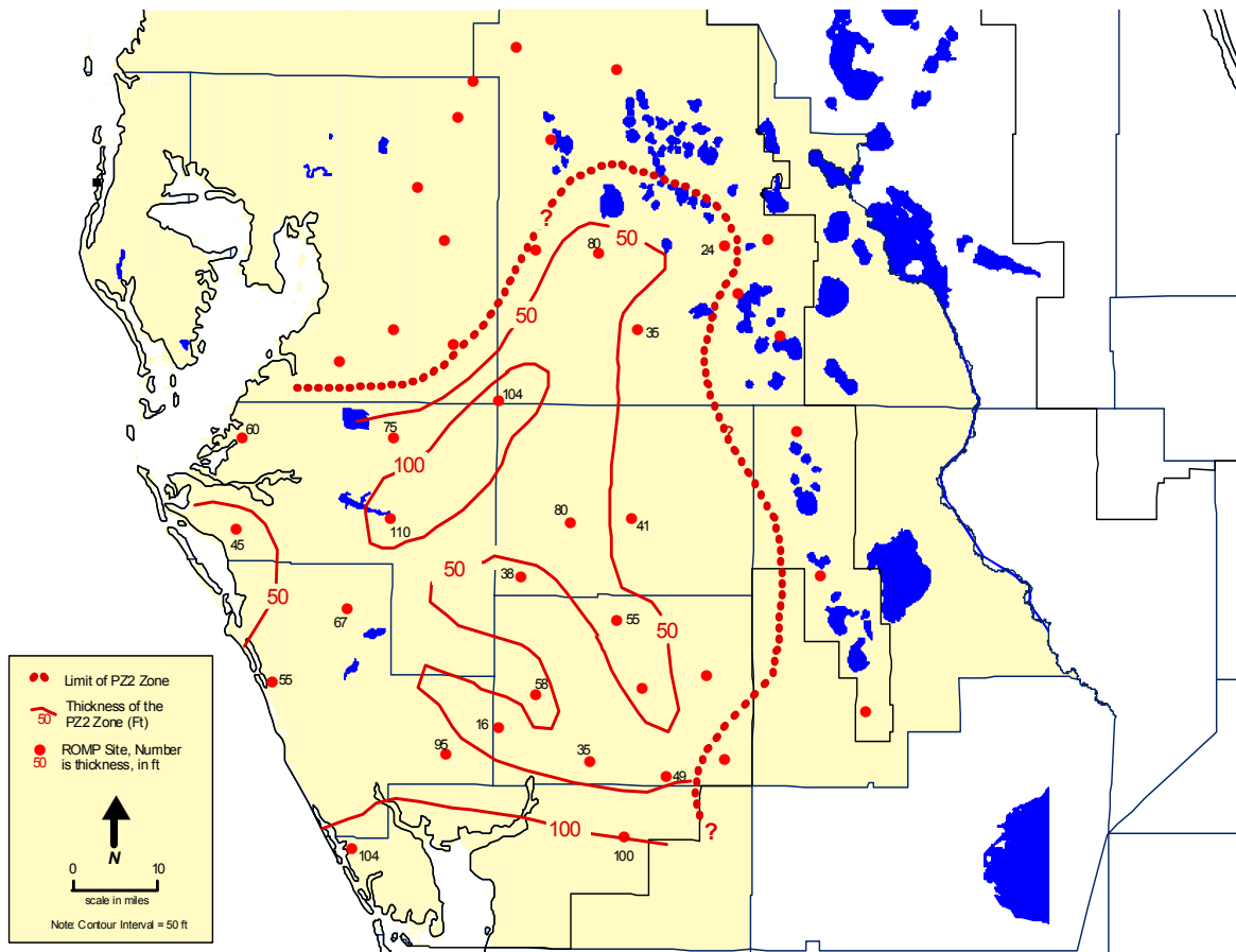
Figure 7. Thickness of IAS PZ 2.
