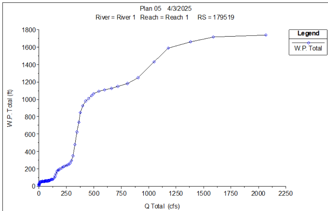
Figure 5-13. Total wetted perimeter versus discharge at Site 179519.
