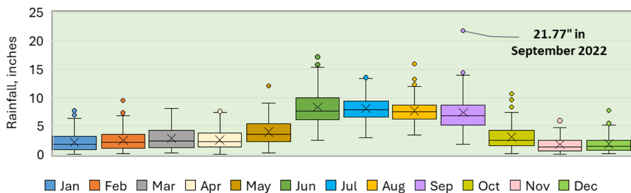
Figure 2-4. Box-and-whisker plot of monthly rainfall for the period of record (1915-2022), based on the District's rainfall summary for the Peace River watershed. For each month, the minimum and maximum values (lower and upper ends of the whisker), median (line within the box), first and third quartiles (lower and upper edges of the box), interquartile range (the box), whisker (vertical line), and outliers (circle markers) are shown.
