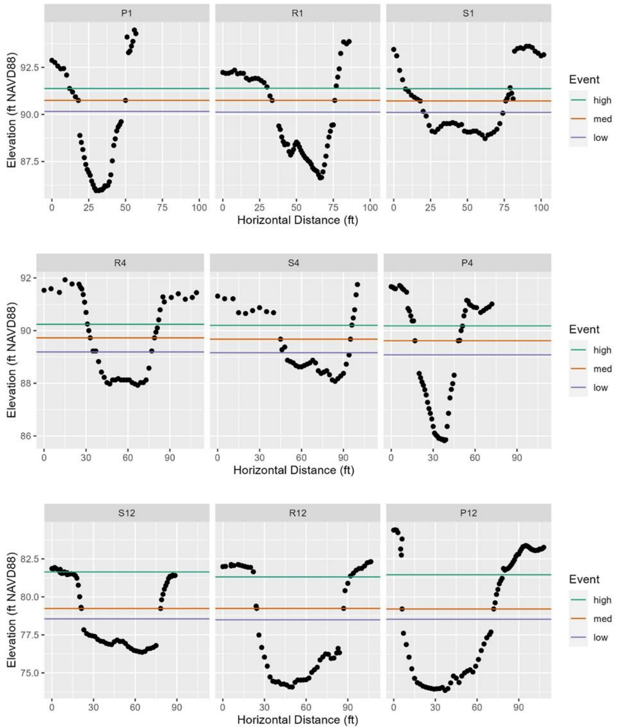
Figure 5-16. Cross-section elevations in the upper segment of the Upper Peace River. Horizontal lines are water surface elevations at high, medium, and low flow events. P, R and S indicate the pool, run and shoal transects, respectively at each site. Within each numbered site, cross sections are arranged from left to right, upstream to downstream.
