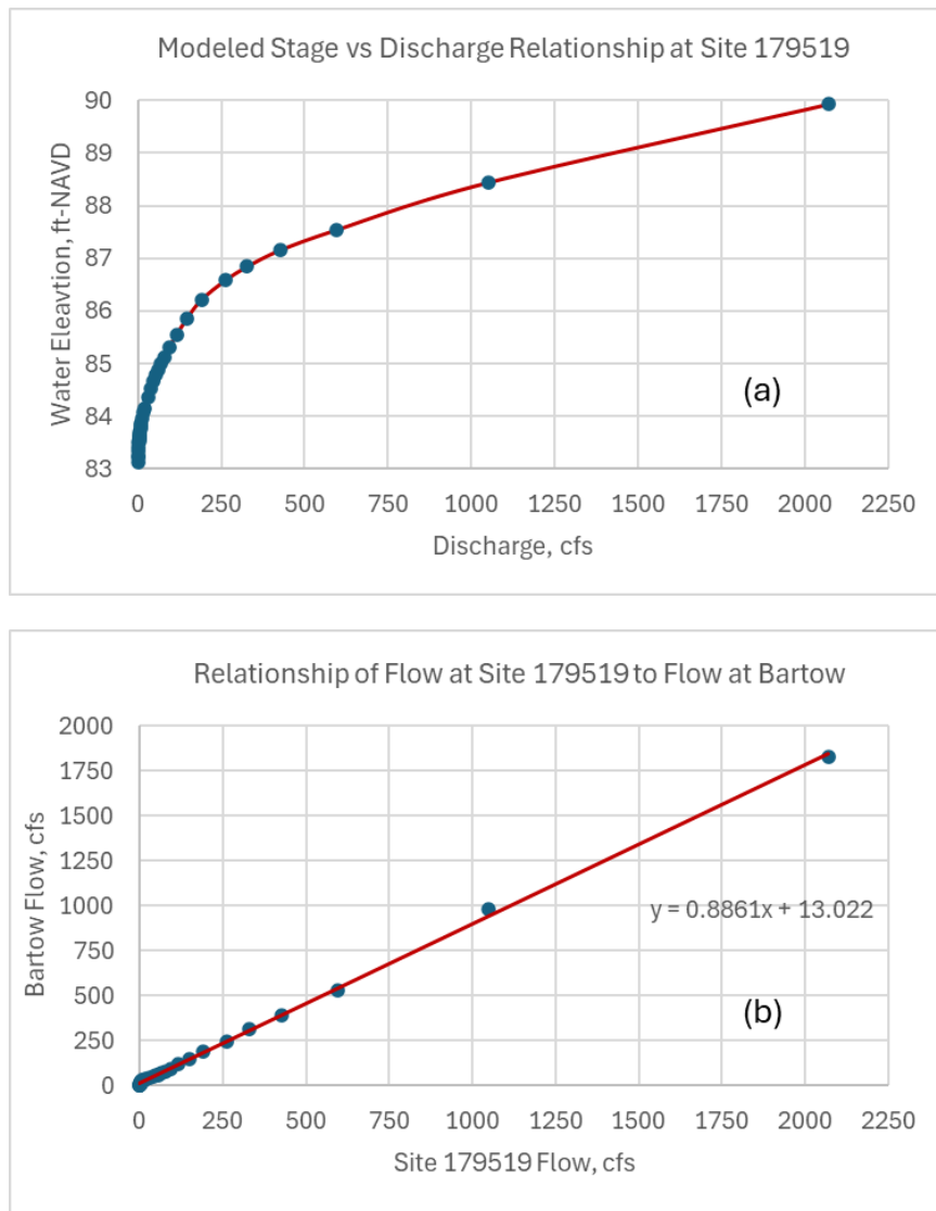
Figure 5-12. Example of graphic outputs generated from modeled flow data used to (a) develop stage-discharge curves at each site to determine the discharge needed to achieve a target water level, and (b) to convert from site flow to gage site flow.
