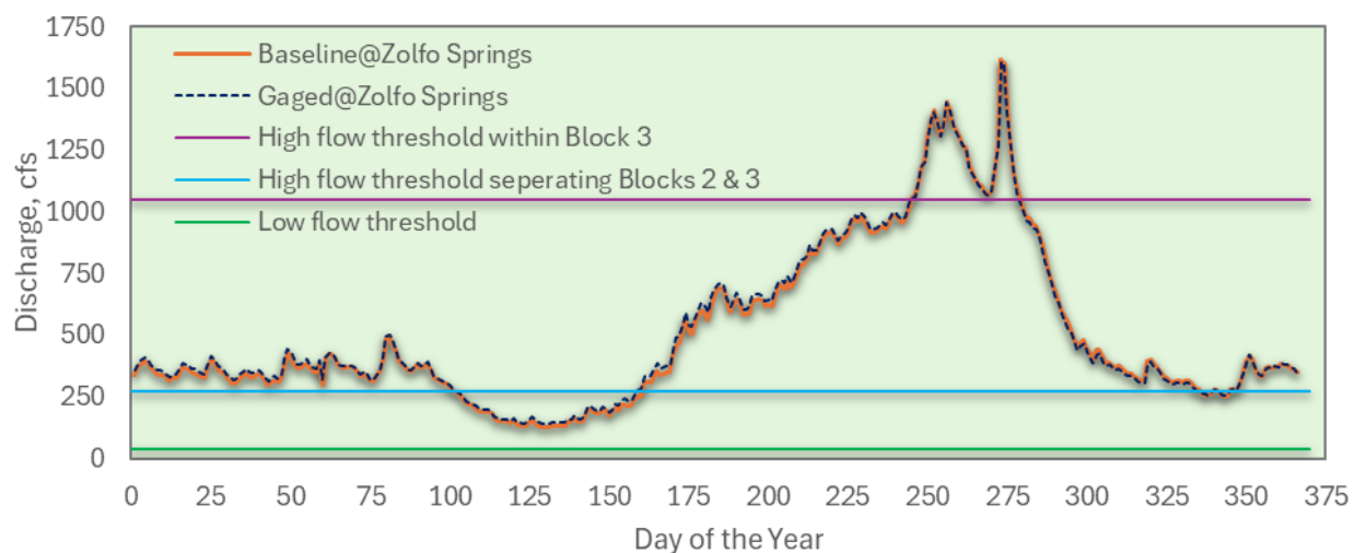
Figure 1-3. Flow blocks are superimposed on hydrographs displaying the mean observed daily flows (dash blue line) and mean baseline daily flows (solid gold line) at the USGS Peace River gaging station at US 17 at Zolfo Springs, FL (No. 02295637). High-flow Block 3 is subdivided into two sub-blocks, as indicated by a purple horizontal line. The boundary between the high-flow (Block 3) and medium-flow (Block 2) blocks is shown by a blue line,
