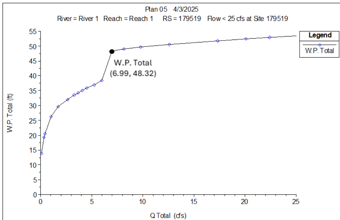
Figure 5-14. Total wetted perimeter versus discharge at Site 179519 for flows below 25 cfs.
