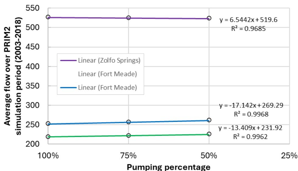
Figure 5-9. Relationship between average simulated flow (2003-2018) and groundwater pumping rates at the Bartow, Fort Meade gage, and Zolfo Springs index gages.
