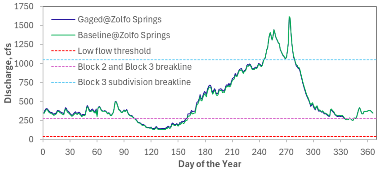
Figure 5-11. Flow blocks are superimposed on hydrographs displaying the mean observed daily flows (solid blue line) and mean baseline daily flows (solid green line) at three USGS Peace River gaging stations: SR60 at Bartow, FL (upper panel, No. 02294650); Fort Meade, FL (middle panel, No. 02294898); and US 17 at Zolfo Springs, FL (lower panel, No. 02295637). High flow Block 3 is subdivided into two sub-blocks, as indicated by a blue dashed horizontal line. The boundary between high-flow (Block 3) and medium-flow (Block 2) is shown by a purple dashed line, while the boundary between medium-flow (Block 2) and low-flow (Block 1) is marked with a red dashed line. Although the mean hydrographs are included for reference, the flow blocks were determined using criteria based on fish passage, wetted perimeter, and floodplain inundation rather than mean flows.
