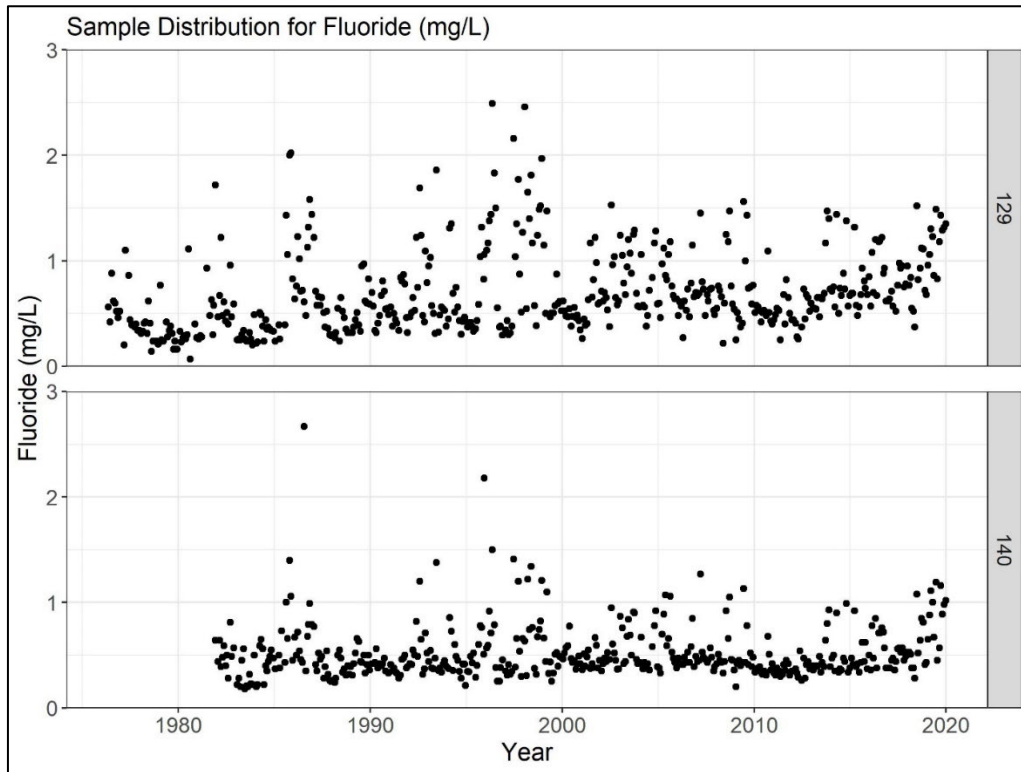
Figure 3-10. Time series of fluoride concentrations (mg/L) for Hillsborough County Environmental Protection Commission Stations 129 and 140 in the Upper Little Manatee River.
