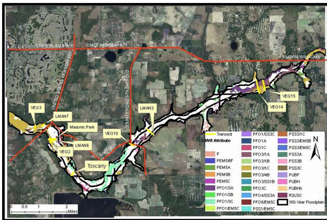
Figure 4-1. Location of vegetation transects and their extent along the Upper Little Manatee River study corridor (from PBS&J 2008 in Appendix J). The legend refers to National Wetlands Inventory (NWI) Attributes of community types within the riparian corridor, which are defined in PBS&J (2008, Appendix J).
