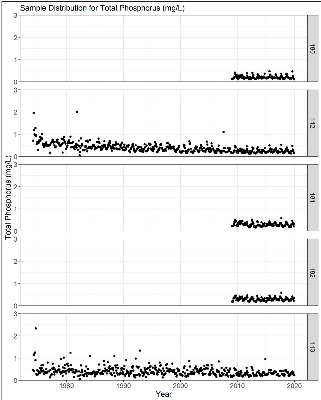
Figure 3-18. Time series of total phosphorus concentrations (mg/L) at five Hillsborough County Environmental Protection Commission stations in the Lower Little Manatee River, shown from downstream (top) to upstream (bottom).
