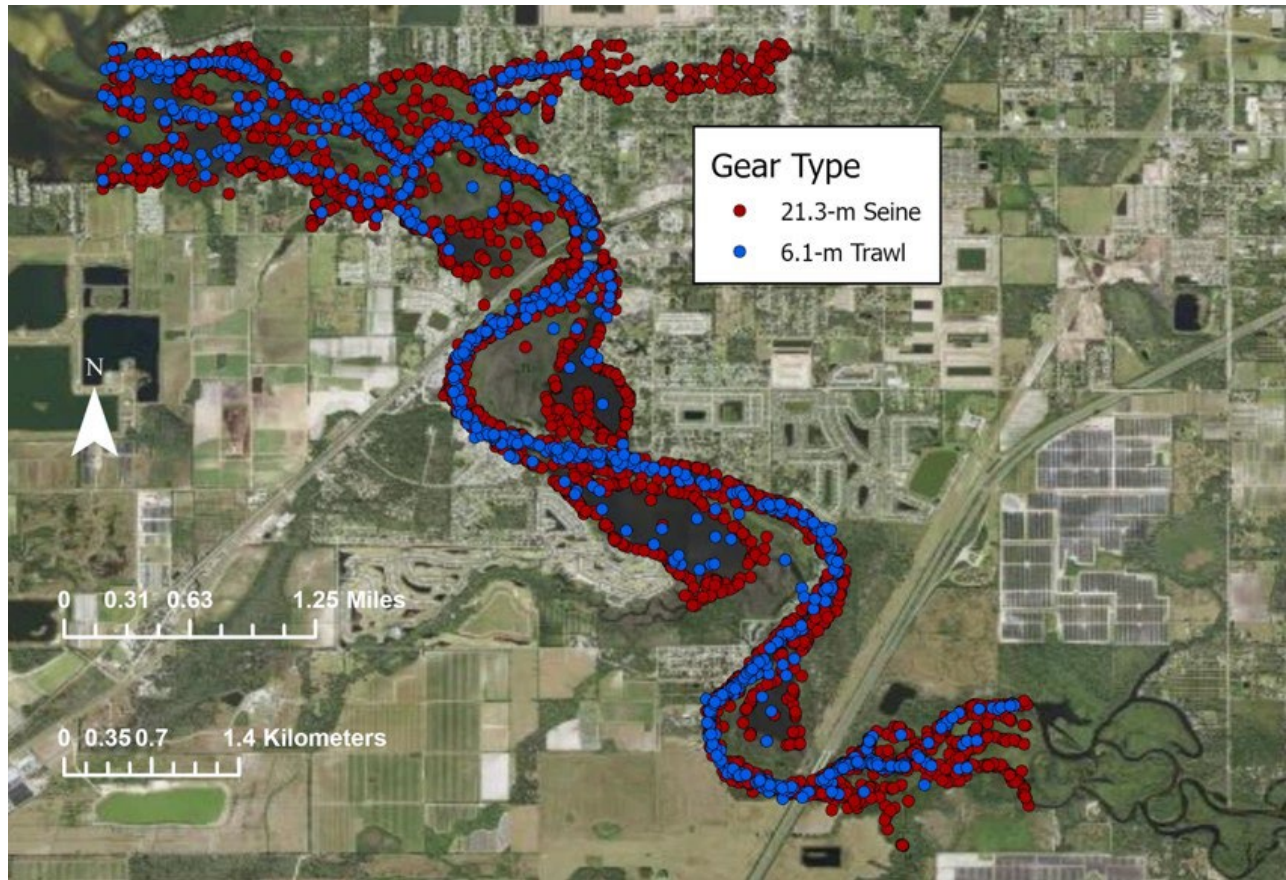
Figure 4-9. All evaluated Fisheries-Independent Monitoring program stratified-random sampling sites by gear type in the Lower Little Manatee River from January 1996 to December 2020.
