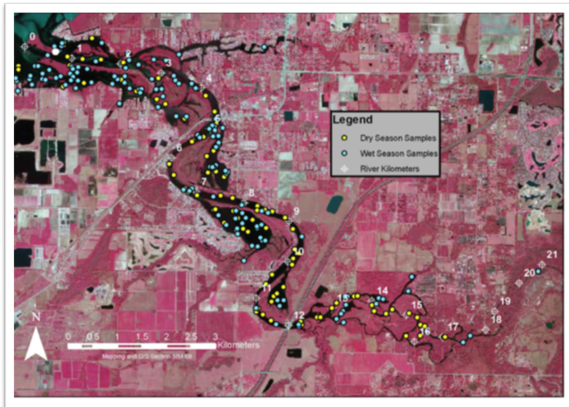
Figure 4-5. Location of benthic macroinvertebrate samples collected between 1996-2005 in the Lower Little Manatee River (from Grabe and Janicki 2008 in Appendix K). River kilometer (RKm) system corresponds with distance from the mouth of the river at RKm 0.
