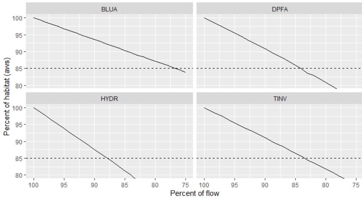
Figure 6-7. Maximum allowable flow reduction for the four most sensitive groups (defined in Table 5-2).
