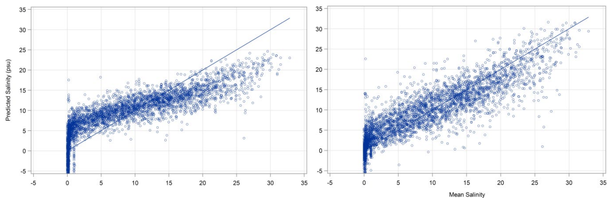
Figure 5-19. Predicted and observed plots for OLS regression (left) and LOESS regression (right) (from JEI 2018b in Appendix E).
