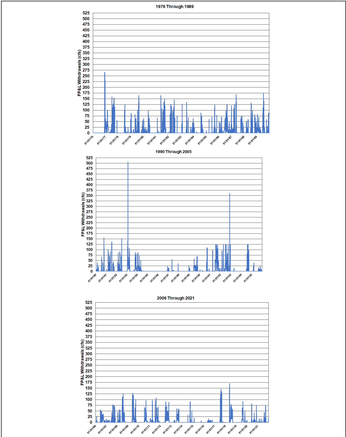
Figure 2-36. Daily surface water withdrawals by the FP&L Company from the Little Manatee River from 1976 through 2021. Top graph: 1976-1989, middle graph: 1990-2005, lower graph: 2006-2021.
