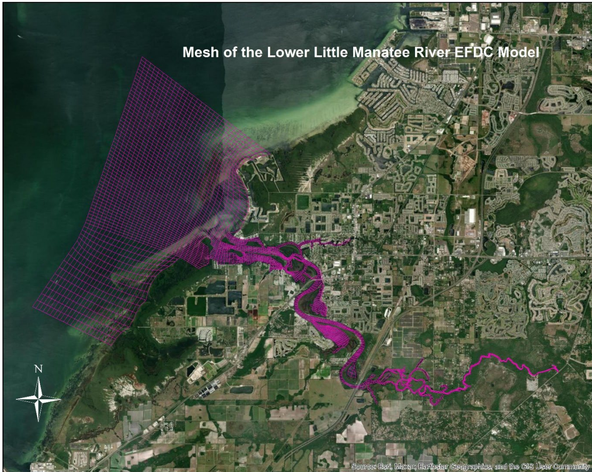
Figure 5-16. The orthogonal grid system (horizontal view) for the EFDC model of the Lower Little Manatee River estuary.
