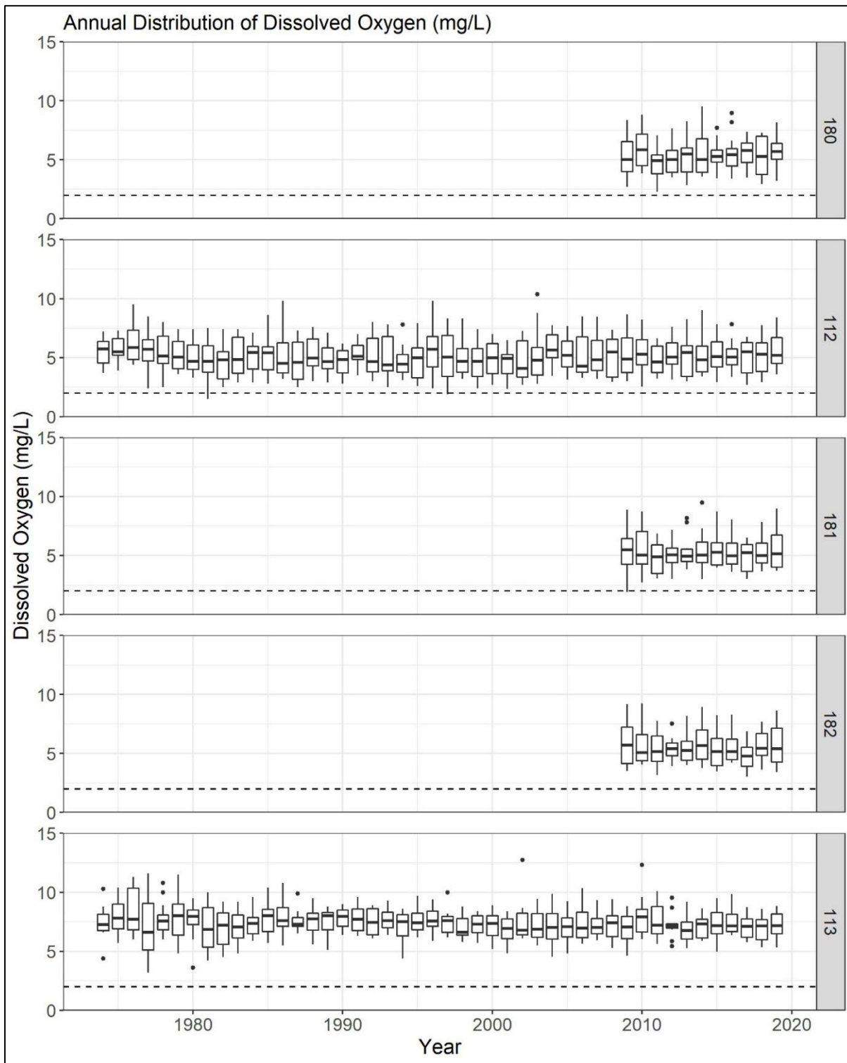
Figure 3-15. Annual distributions of mid-water column dissolved oxygen concentrations (mg/L) for the period of record at five Hillsborough County Environmental Protection Commission stations in the Lower Little Manatee River, with stations listed from downstream (top) to upstream (bottom). The dashed horizontal line represents the 2 mg/L threshold for hypoxic conditions. Boxed values include the 25 th to the 75 th percentiles with the centerline reflecting the 50 th percentile value. Outliers are indicated by dots, representing values outside of the 1.5*Interquartile Range.
