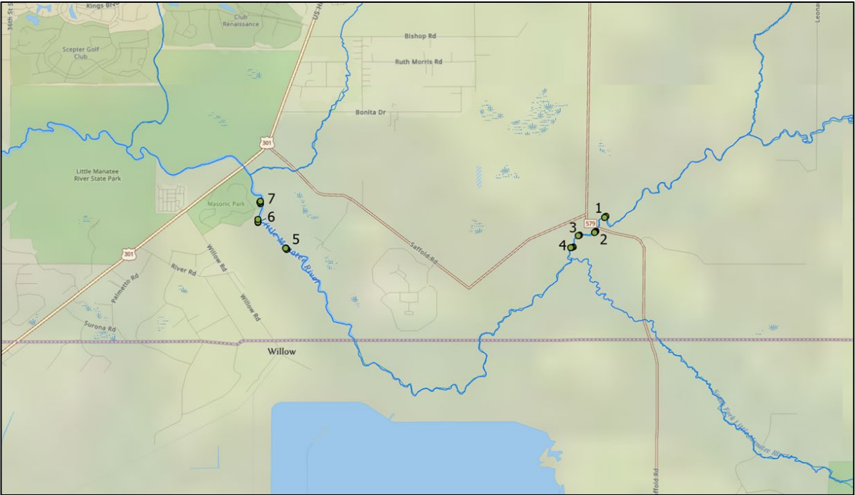
Figure 5-13. The location of the seven sites where substrate/cover was characterized in July 2020 for the SEFA at a total of 21 cross sections along the Upper Little Manatee River.
