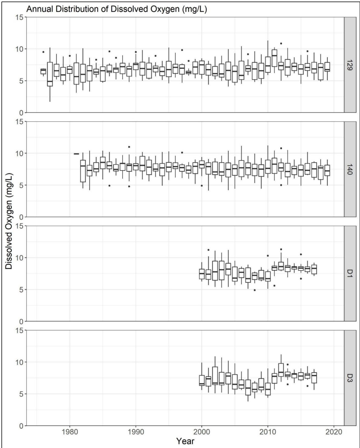
Figure 3-4. Annual distribution of mid-water dissolved oxygen concentrations (mg/L) at two Hillsborough County Environmental Protection Commission stations (129 and 140) and two Manatee County stations (D1 and D3). Boxed values include the 25 th to the 75 th percentiles with the centerline reflecting the 50 th percentile value. Outliers are indicated by dots, representing values outside of the 1.5*Interquartile Range.
