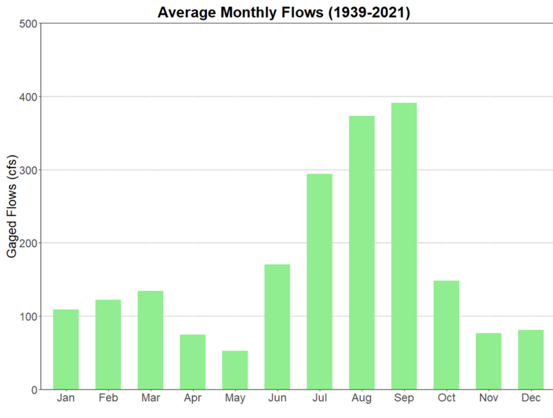
Figure 2-28. Average monthly rates of flow measured at the USGS Little Manatee River at US 301 near Wimauma, FL (No. 02300500) gage from 1939 through 2021.
