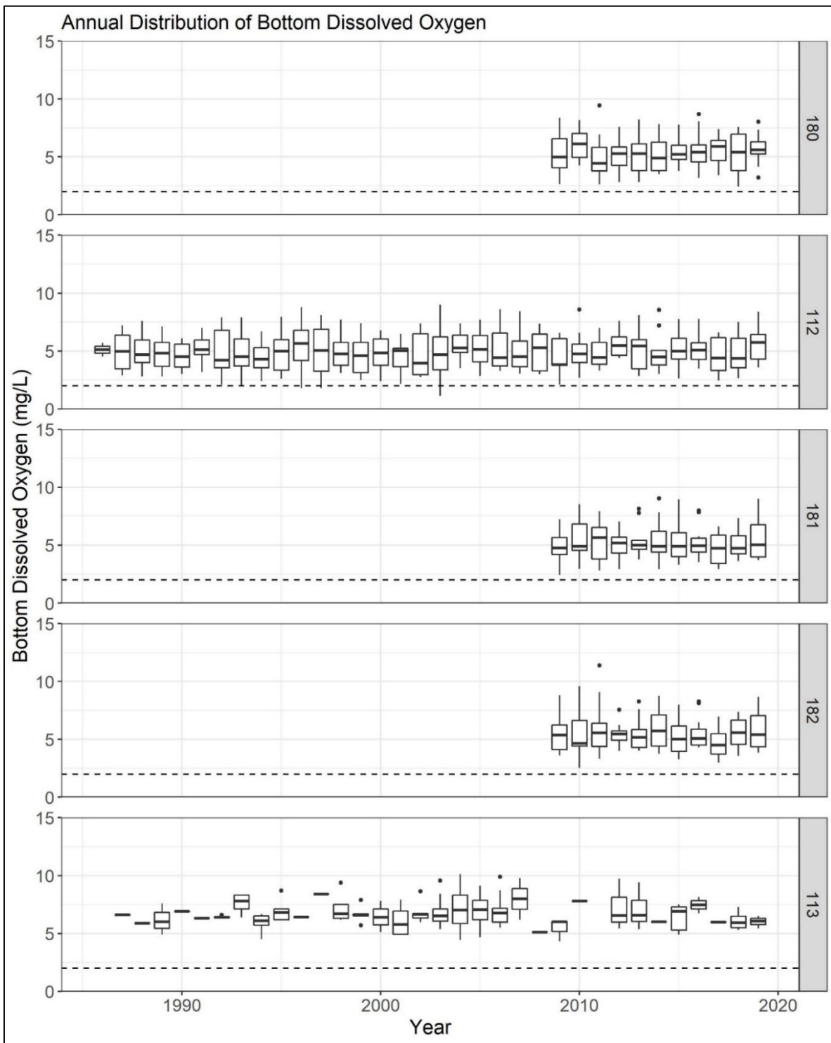
Figure 3-16. Annual distributions of bottom-water column dissolved oxygen concentrations (mg/L) for the period of record at five Hillsborough County Environmental Protection Commission stations in the Lower Little Manatee River, with stations listed from downstream (top) to upstream (bottom). The dashed horizontal line represents the 2 mg/L threshold for hypoxic conditions. Boxed values include the 25 th to the 75 th percentiles with the centerline reflecting the 50 th percentile value. Outliers are indicated by dots, representing values outside of the 1.5*Interquartile Range.
