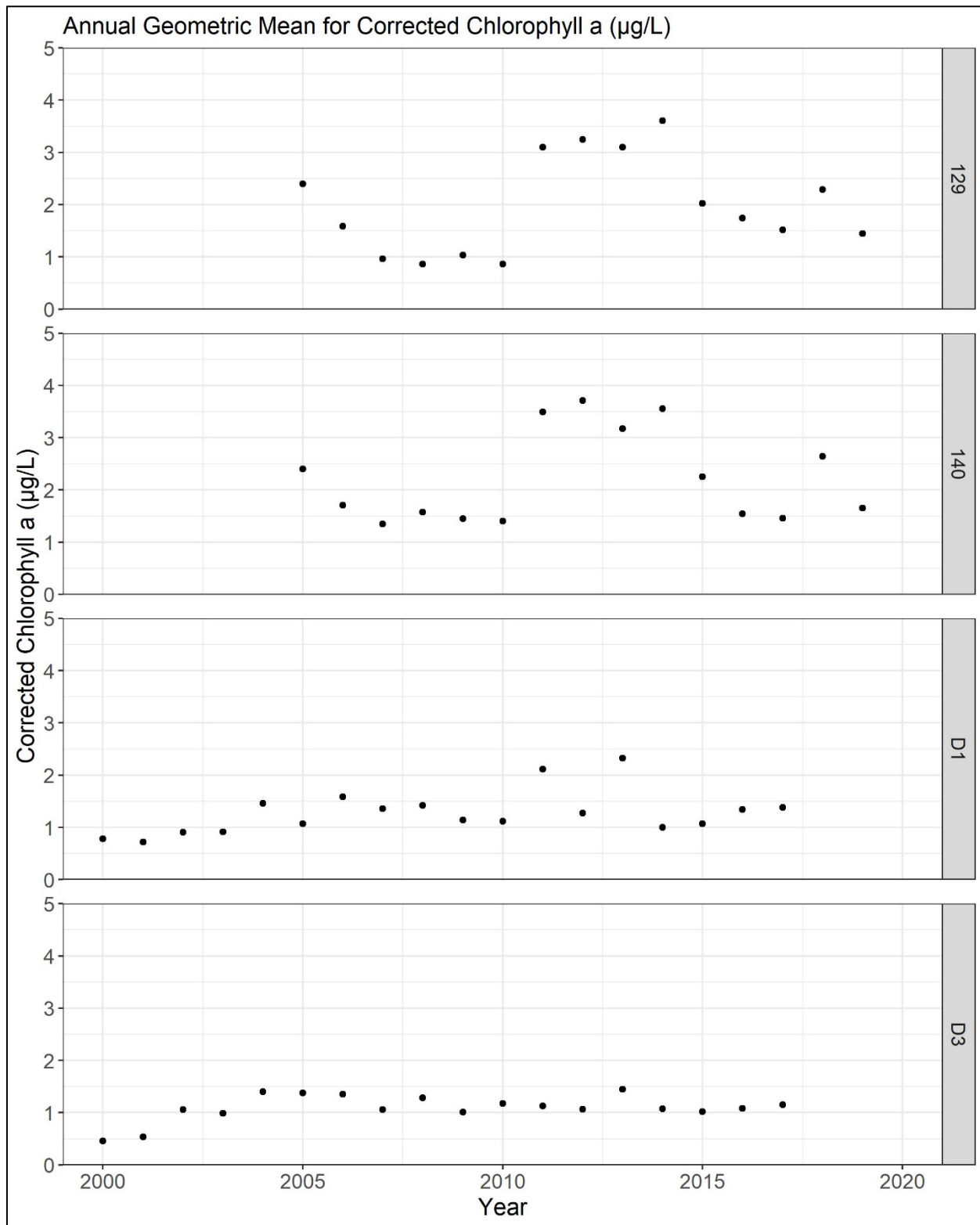
Figure 3-4. Annual geometric mean corrected chlorophyll a concentrations ( \mu\text{g/L} ) for the period of record at Hillsborough County Environmental Protection Commission Stations 129 and 140 and Manatee County Stations D1 and D3 in the Upper Little Manatee River.
