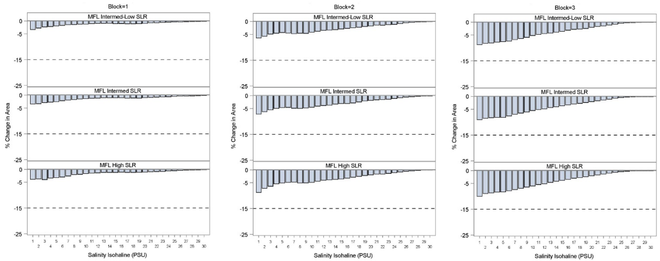
Figure 7-2. Percentage changes of simulated bottom areas of isohalines 1, 2, ... 30 psu under the minimum flow condition with the intermediate-low, intermediate, and high sea level rise (SLR) projections relative to those under the baseline flow condition with the three SLR projections.
