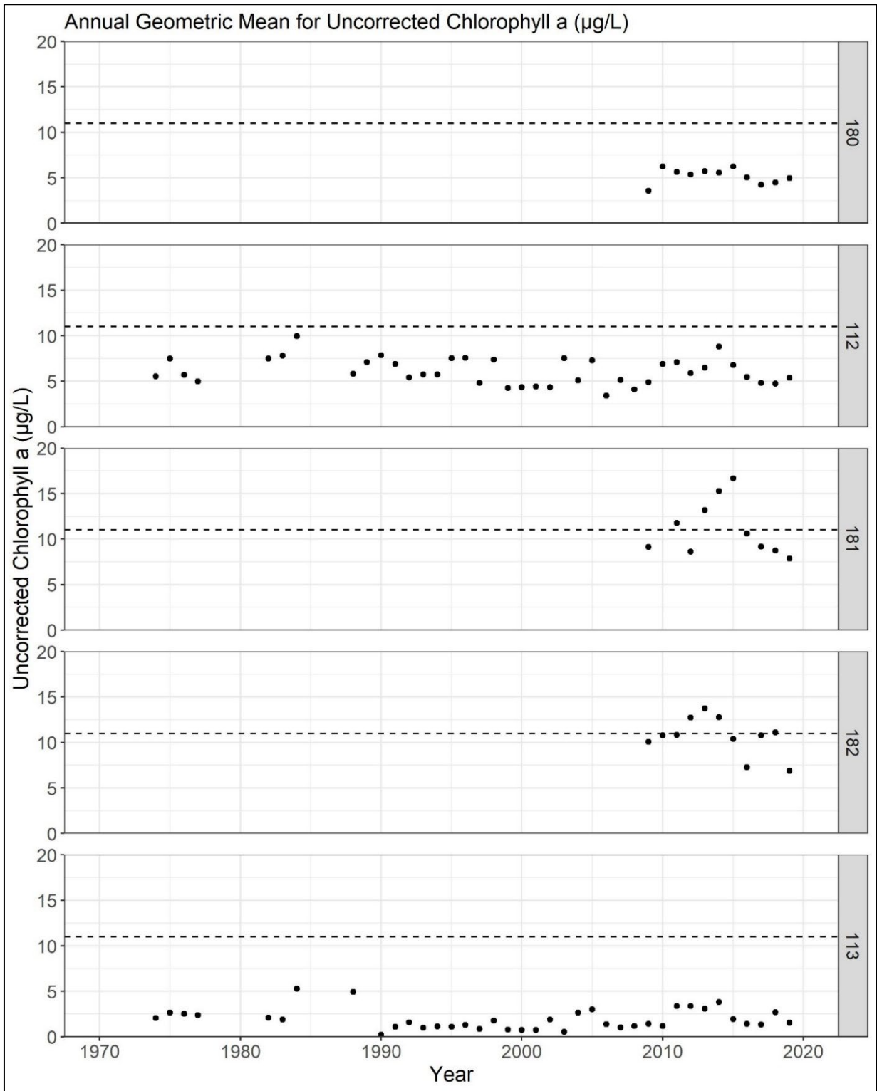
Figure 3-13. Annual geometric mean uncorrected chlorophyll a concentrations ( \mu\text{g/L} ) for the period of record at five Hillsborough County Environmental Protection Commission stations in the Lower Little Manatee River, with stations listed from downstream (top) to upstream (bottom). The dashed horizontal lines represent the 11 \mu\text{g/L} Florida Department of Environmental Protection chlorophyll a threshold.
