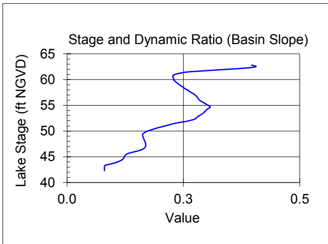
Figure 13. Surface area, maximum depth, mean depth, volume, dynamic ratio (basin slope) in feet above NGVD 29 for Lake Keene.
