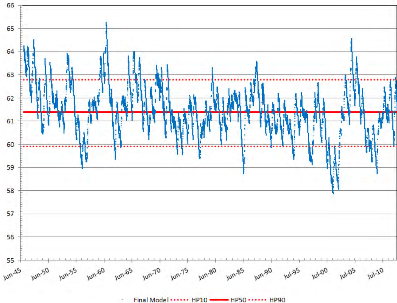
Figure 10. Modeled long term Historic lake stage and measured lake stage (both as daily) used to calculate the Historic P10, P50, and P90 lake stage percentile elevations for Lake Keene from January 1946 through July 2013. The long term Historic P10, P50, and P90 are depicted as horizontal solid and dotted lines.
