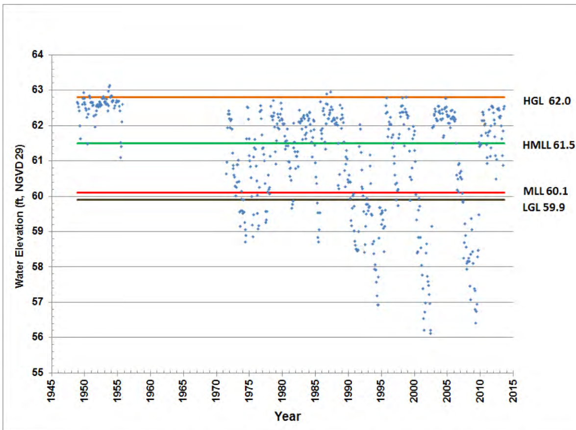
Figure 11. Mean monthly lake stage for Lake Keene of the period of record; and Minimum and Guidance Levels for Lake Keene (as NGVD 29). Levels shown include the High Guidance Level (HGL), High Minimum Lake Level (HMLL), Minimum Lake Level (MLL), and the Low Guidance Level (LGL).
