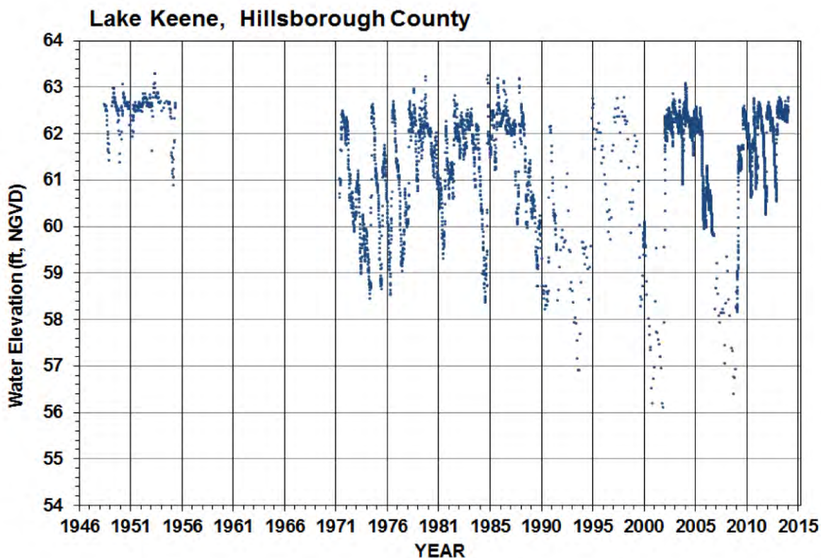
Figure 8. Daily surface water elevations (NGVD 29) through July 2014 for Lake Keene, SWFWMD WMIS site ID's 19189.
