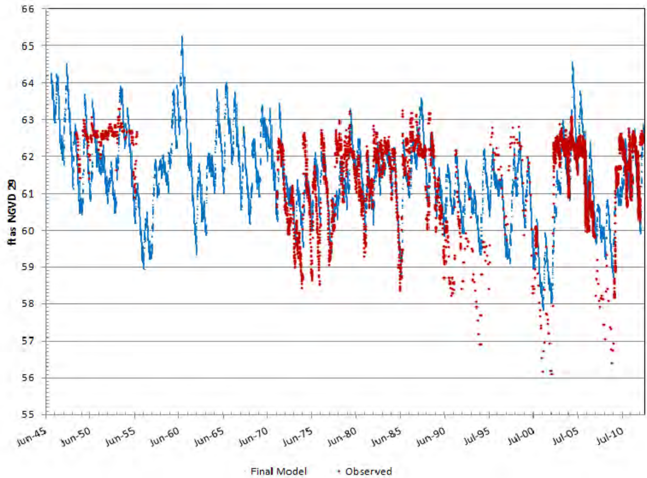
Figure 9. Modeled long term Historic lake stage (as daily, see blue line) from 1946 to 2013 and observed lake stage (as daily, see red points) for Lake Keene.
