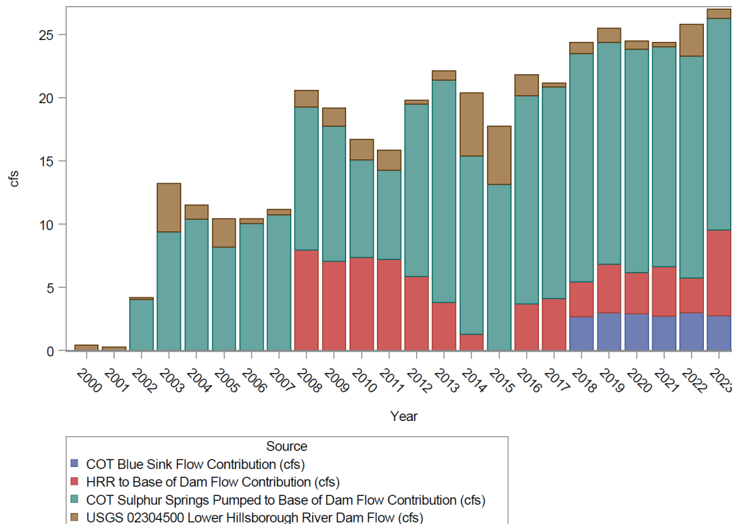
Figure 5.1-3: Stacked bar plot of recovery source contributions and dam flows (USGS 02304500) to the total LHR flow
