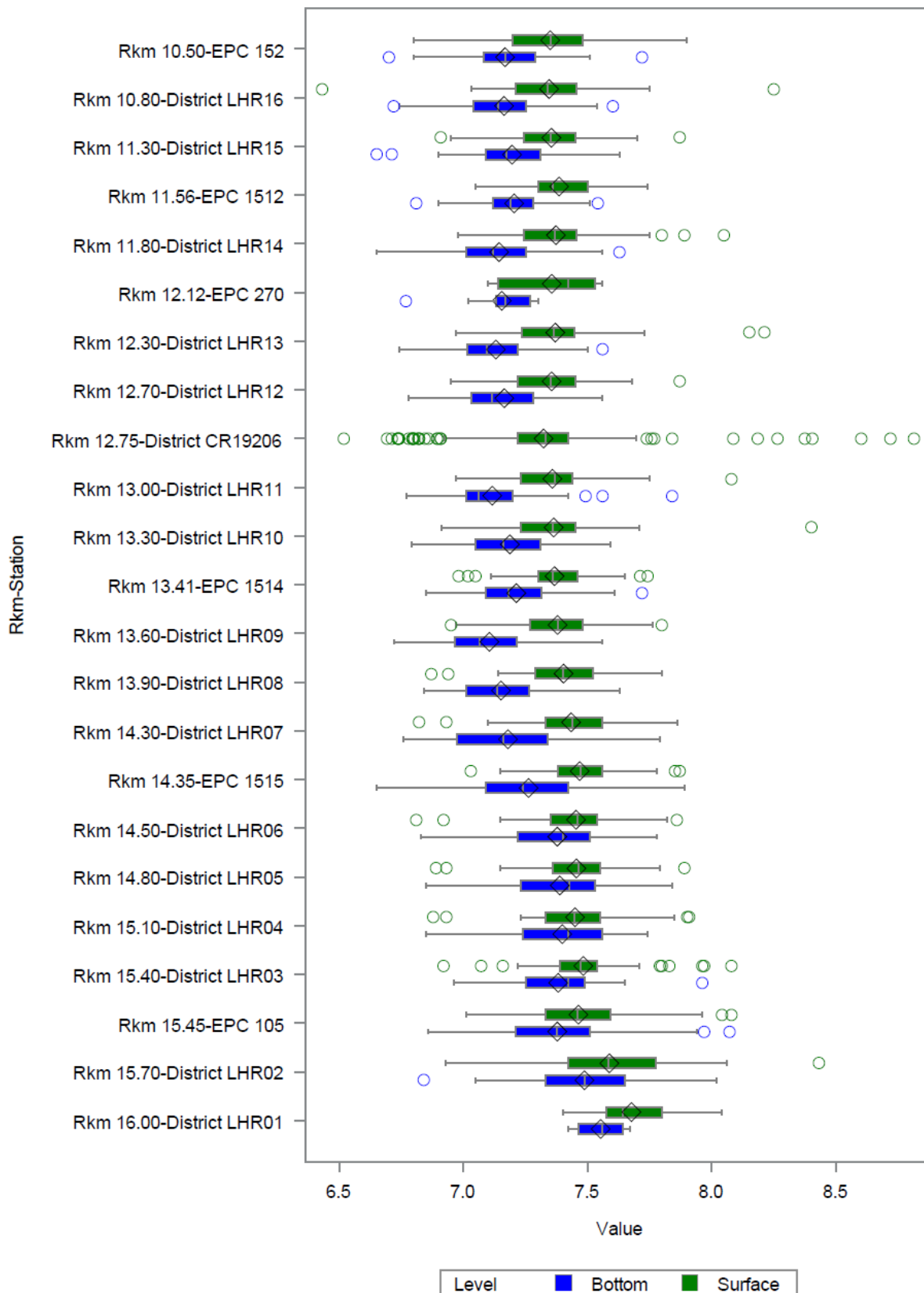
Figure 5.2-63: Distribution for pH (SU) within the LHR target zone by fixed-location stations for specified water column strata (Analysis Days)
