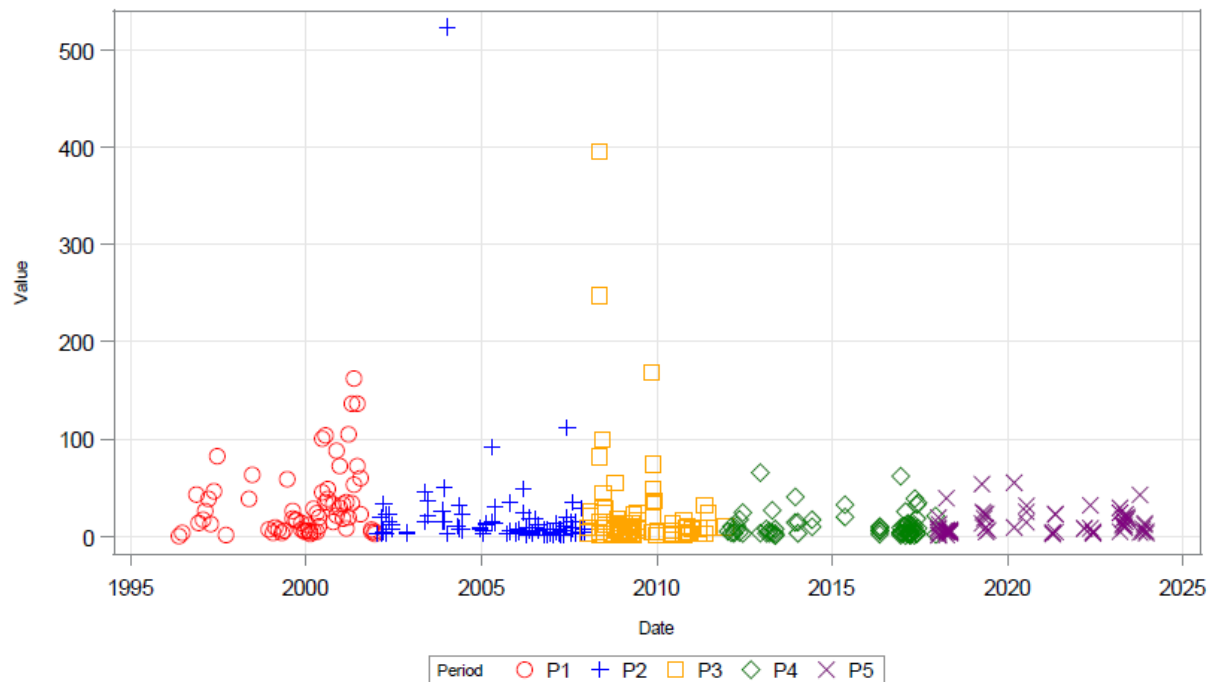
Figure 5.2-84: Time series for surface chlorophyll (µg/L) within the LHR target zone (Analysis Days)
