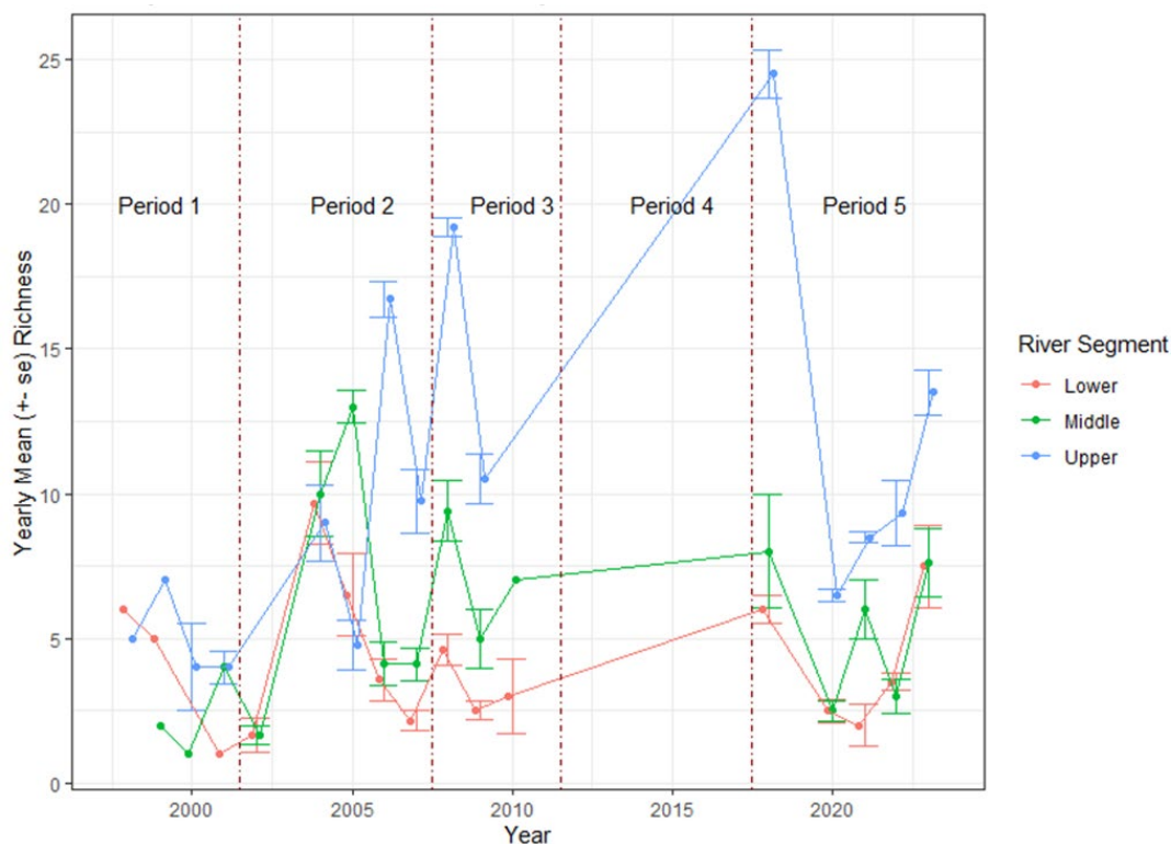
Figure 6.2-39: Salinity-sensitive benthic macroinvertebrate taxa richness over time
