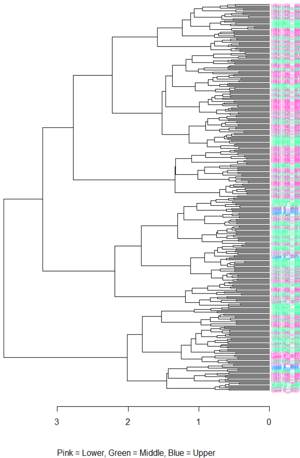
Figure 6.2-1: Hierarchical clustering of zooplankton data
