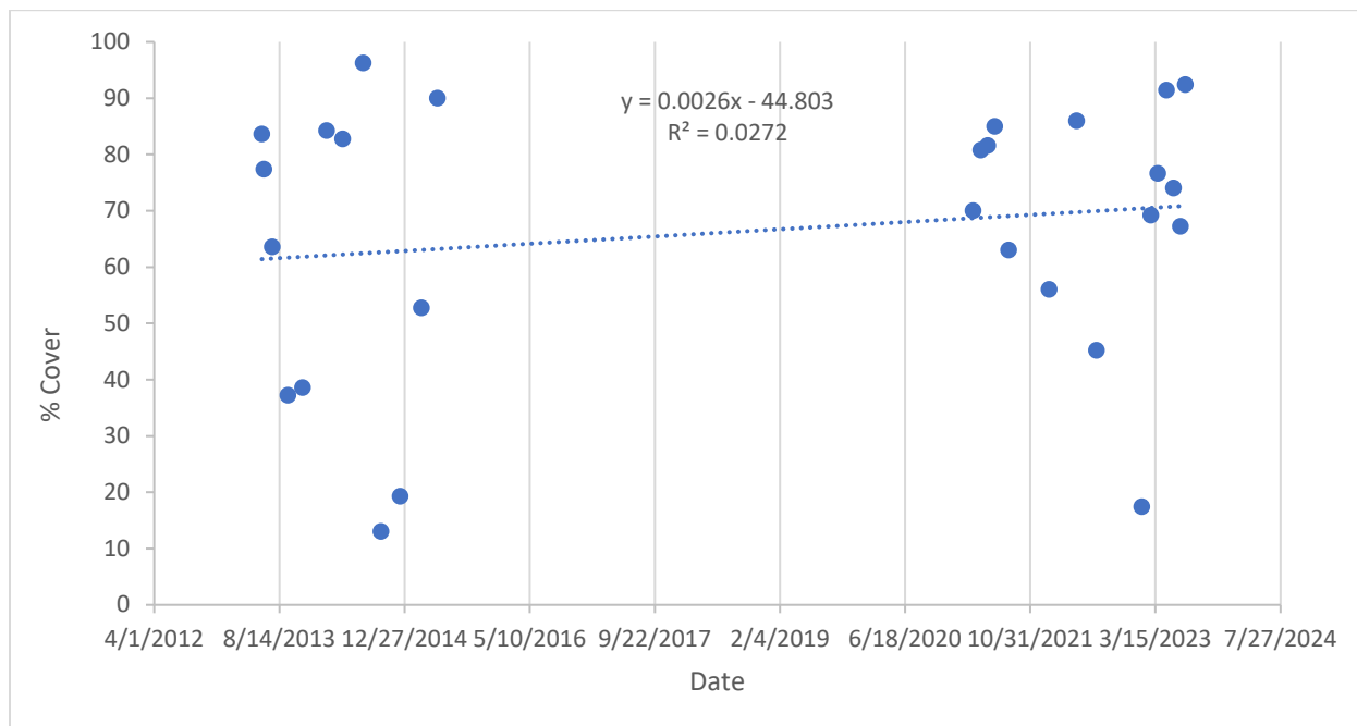
Figure 4.3-1: Sulphur Springs Run mean macroalgae and SAV percent coverage over time
