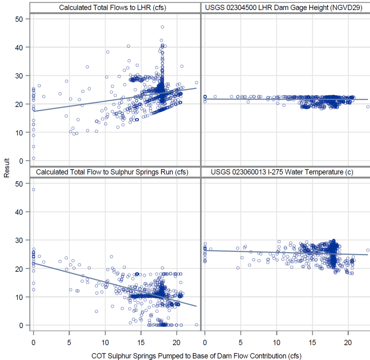
Figure 4.1-3: Scatter plot with regression line depicting relationship between flows pumped to the base of the Hillsborough Dam to meet the LHR minimum flow and other parameters related to the Sulphur Springs minimum flow. Implementation Days only
