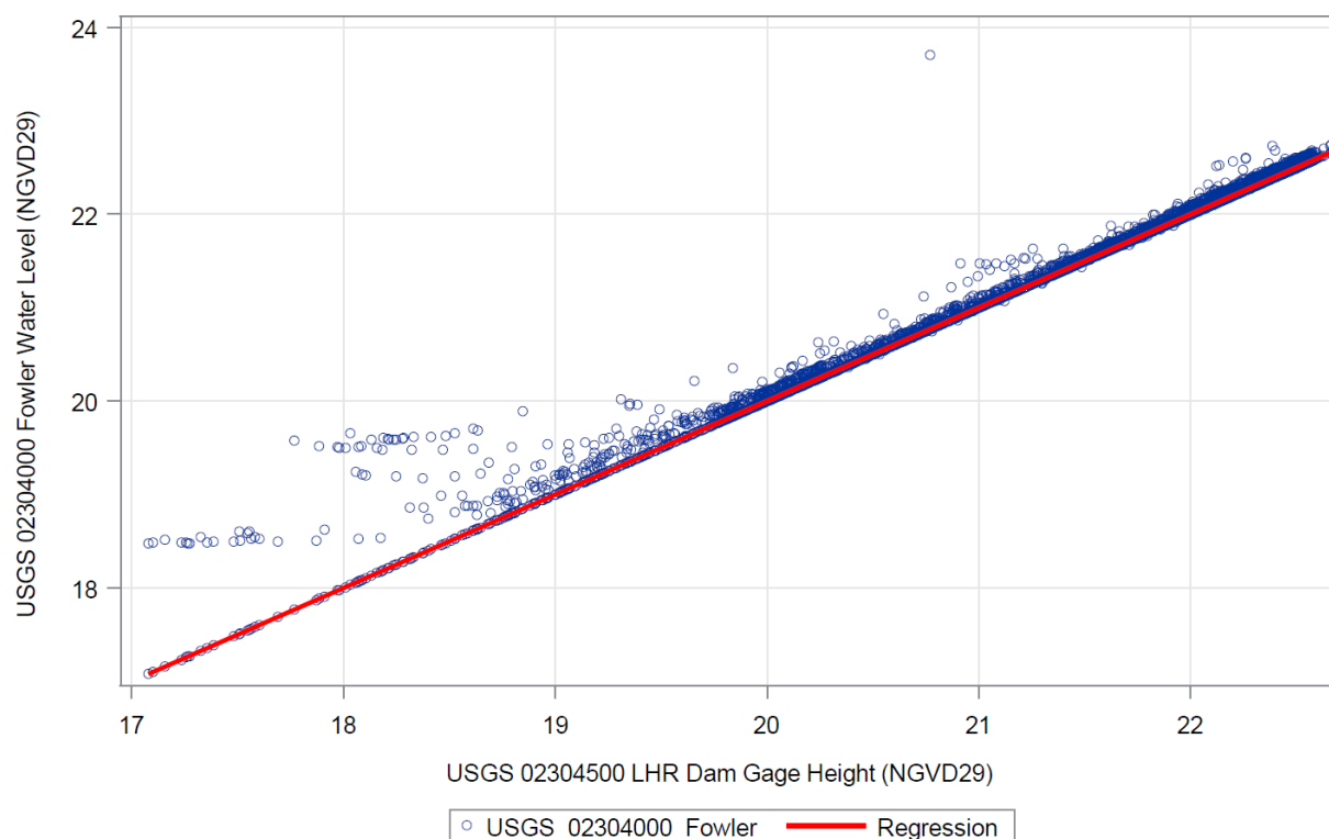
Figure 4.1-6: Comparison of water levels at the Hillsborough River Dam (x axis) and water levels at USGS 02304000 Fowler (y axis) filtered to Implementation Days only with a 1:1 regression line for reference (red solid line)
