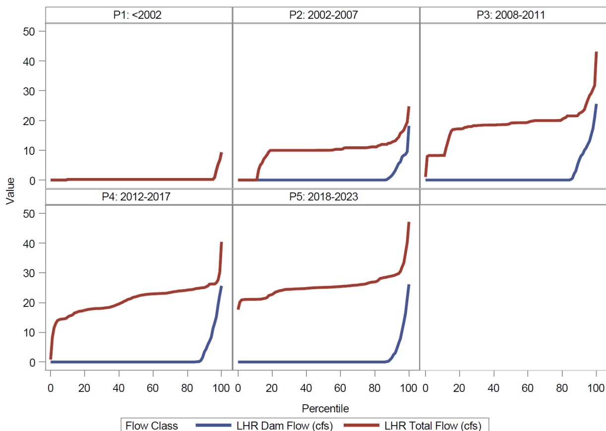
Figure 5.1-4: Cumulative distribution function plots comparing dam flows and calculated total flows for each period when implementation was required under the minimum flow (Implementation Days).
