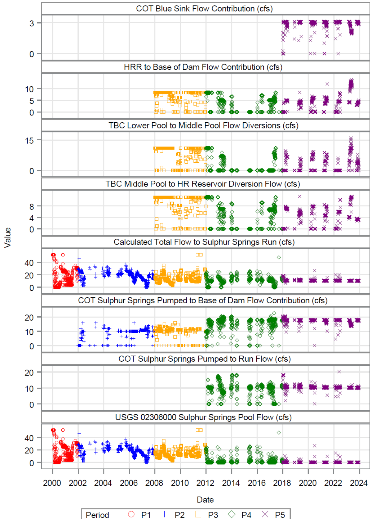
Figure 4.1-1: Time series of recovery source water daily average flow (Implementation Days Only) during the five minimum flow implementation periods
