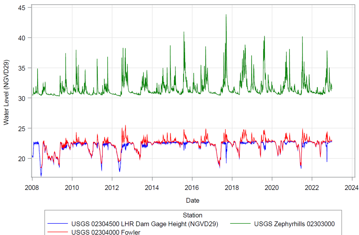
Figure 4.1-7: Water levels at the Hillsborough River Dam, USGS 02304000 Fowler, and USGS 02303000 Zephyrhills
