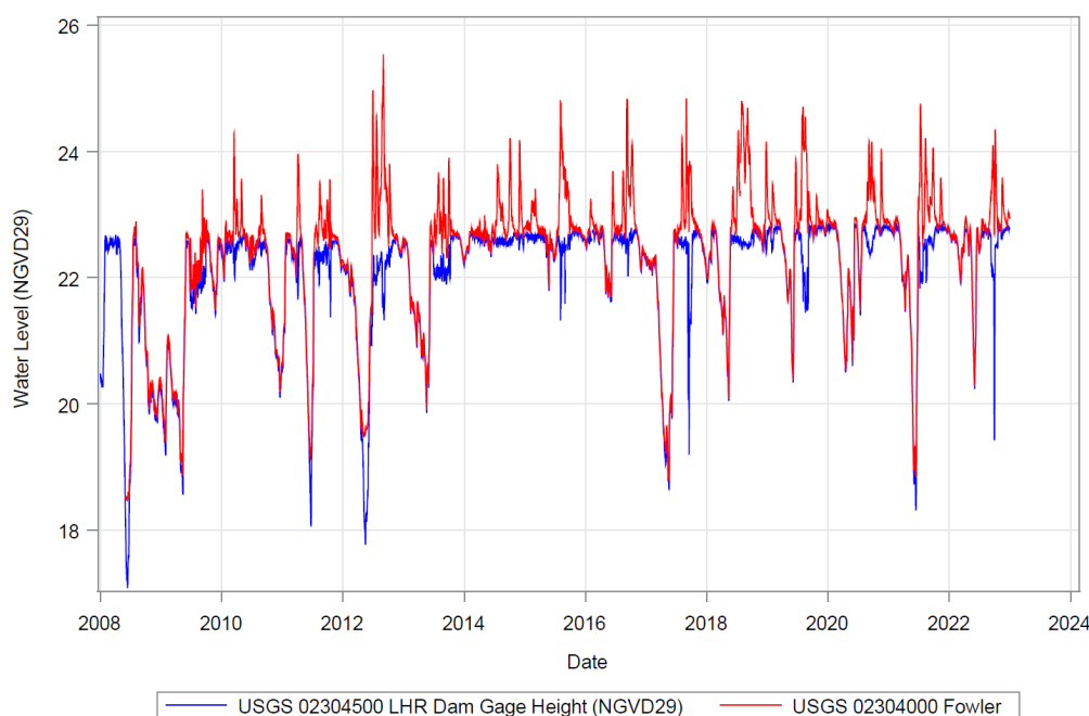
Figure 4.1-5: Extension of data through 2023 comparing the water levels at the Hillsborough River Dam and at USGS 02304000 Fowler
