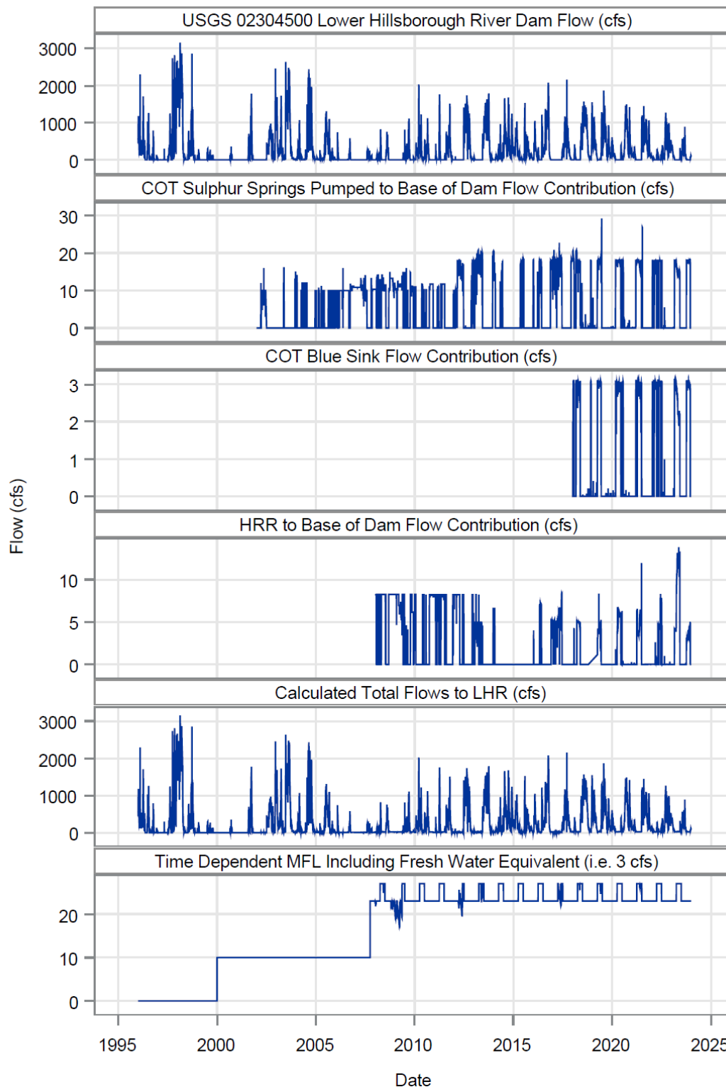
Figure 3.2-1: Time series plot of flow contributions and contributing terms to the calculation of the total flow to the LHR and selection criteria used for analysis using all days in the POR 1996–2023
