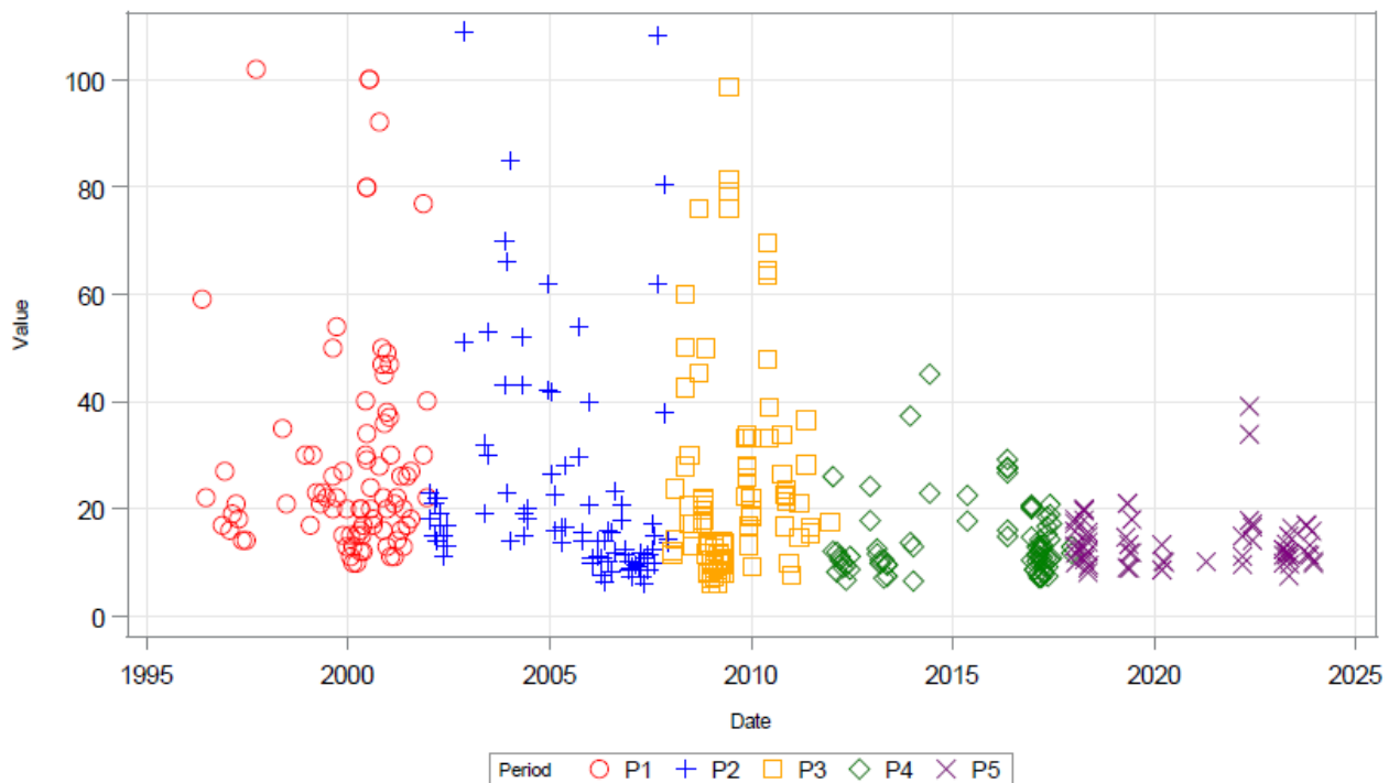
Figure 5.2-64: Time series of surface color (PCU) within the LHR target zone (Analysis Days)
