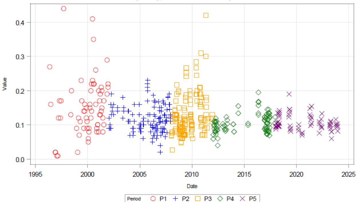
Figure 5.2-80: Time series for surface orthophosphate (mg/L) within the LHR target zone (Analysis Days)
