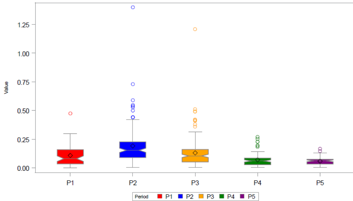
Figure 5.2-73: Distribution for surface nitrate + nitrite (mg/L) within the LHR target zone by period (Analysis Days)
