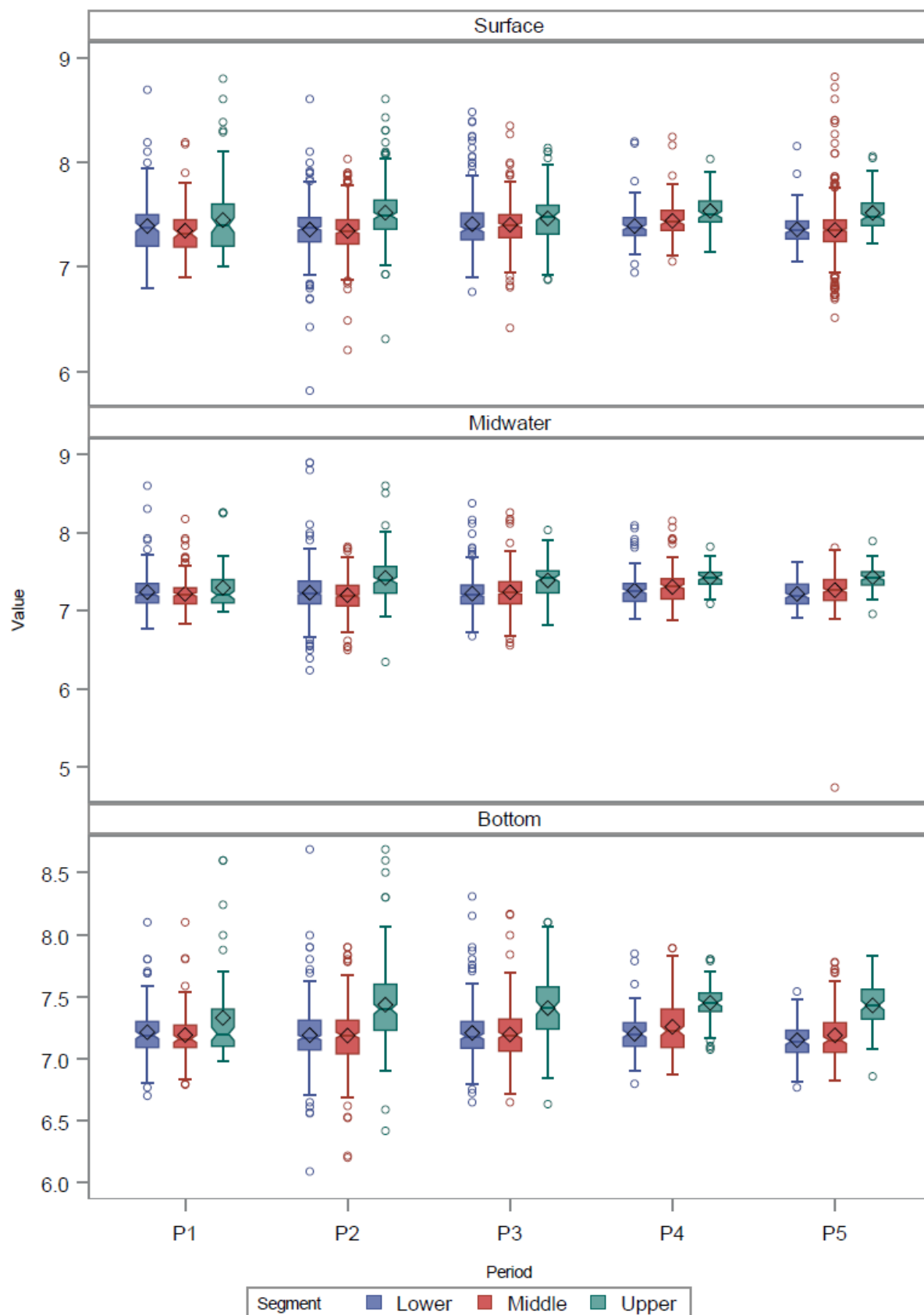
Figure 5.2-61: Distribution of pH (SU) within the LHR target zone by period and river segment for specified water column strata (Analysis Days)
