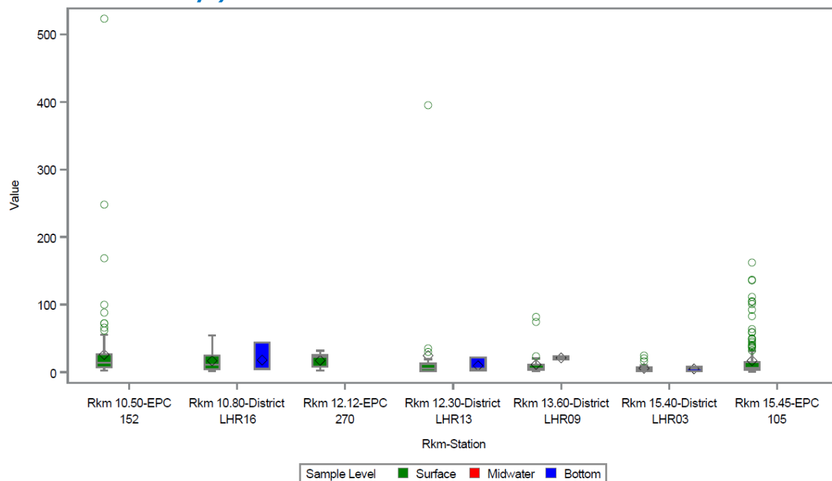
Figure 5.2-87: Distribution for chlorophyll ( \mu\text{g/L} ) within the LHR target zone by fixed-location stations for specified water column strata (Analysis Days)
