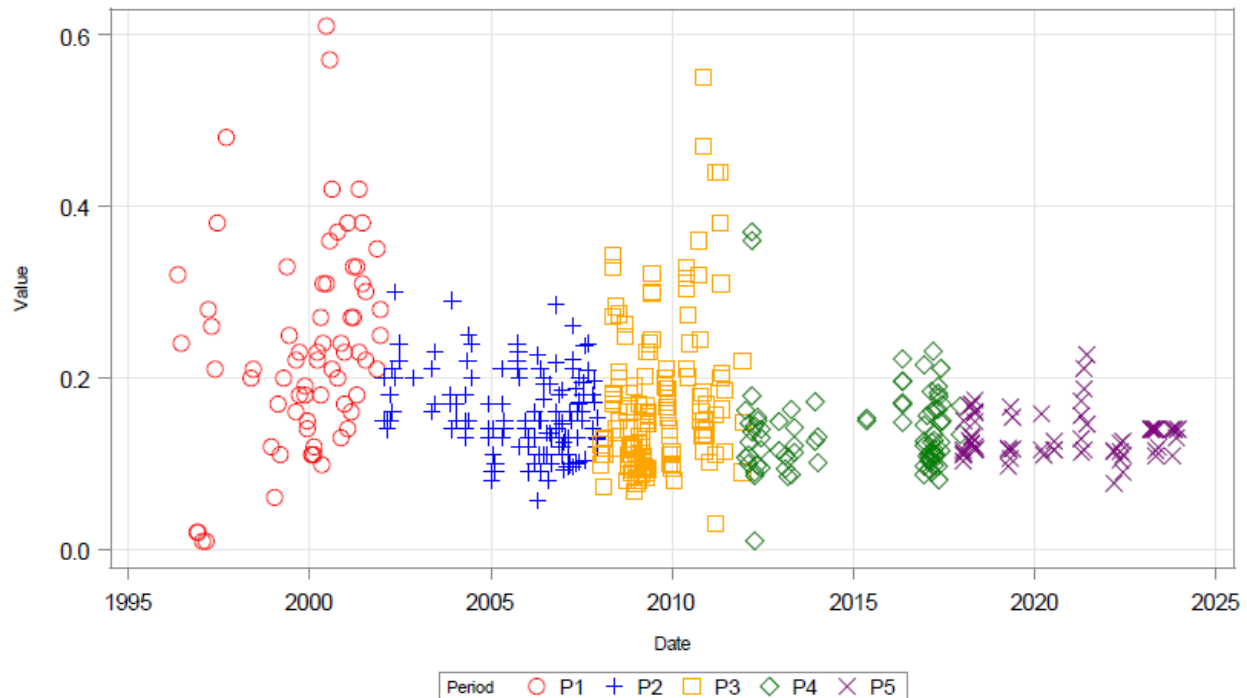
Figure 5.2-76: Time series for surface total phosphorus (mg/L) within the LHR target zone (Analysis Days)
