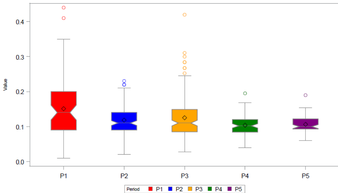
Figure 5.2-81: Distribution for surface orthophosphate (mg/L) within the LHR target zone by period (Analysis Days)
