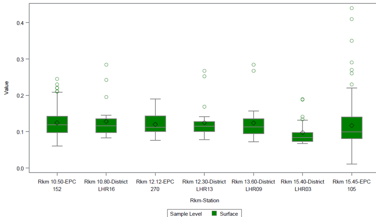
Figure 5.2-83: Distribution for orthophosphate (mg/L) within the LHR target zone by fixed-location stations (Analysis Days)
