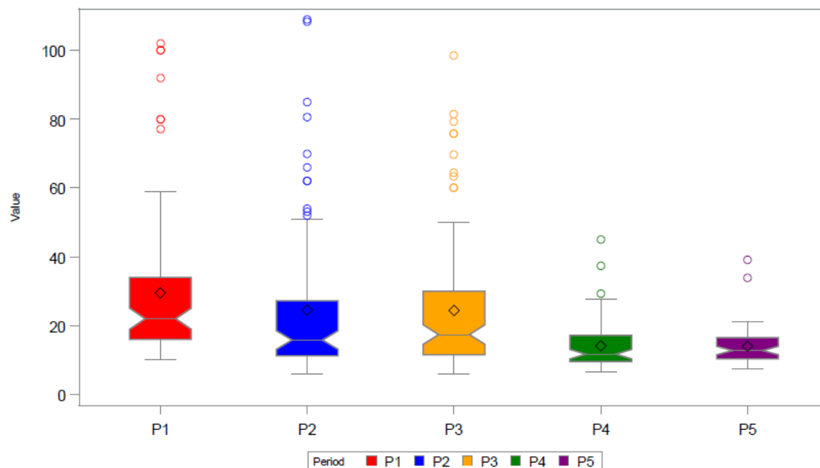
Figure 5.2-65: Distribution for surface color (PCU) within the LHR target zone by period (Analysis Days)
