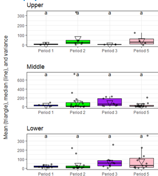
Figure 6.2-81: Boxplots of abundance of Stenoninereis martini by period and segment with Dunn's test comparisons represented by compact letter display
