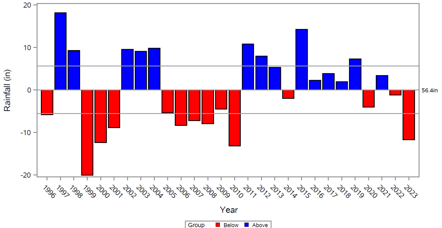
Figure 5.1-2: Deviation of annual rainfall (Hillsborough River at Sulphur Springs station (District 19436) from the POR average (56.4 inches) between 1996–2023. Bar plots identify annual deviations below (red) or above (blue) the POR average. Horizontal reference lines indicate a 10% departure from the long term average
