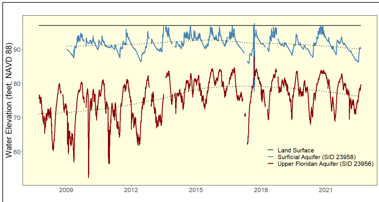
Figure 2-18. Water levels (feet) from monitor wells installed into the surficial and Upper Floridan aquifers at the District Regional Observation and Monitor-Well Program 43 site from 2007 through August 2022. The dashed lines indicate the overall trend using LOESS.
