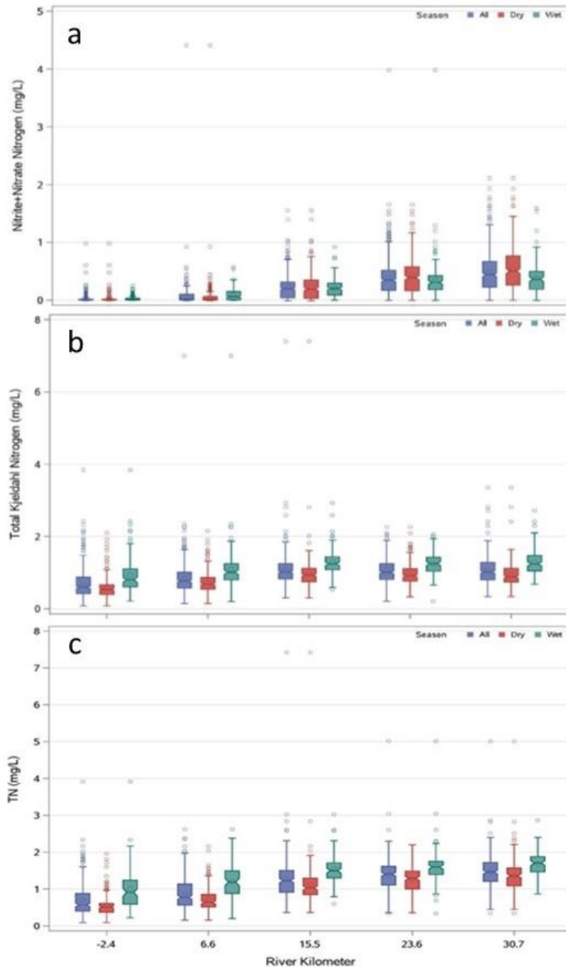
Figure 3-7. Box and whisker plots of a) Nitrate+Nitrite ( \text{NO}_x ), b) Total Kjeldahl Nitrogen (TKN), and c) Total Nitrogen (TN) concentrations measured at selected HBMP fixed-stations in the Lower Peace River and near the river mouth (sampling station identifiers correspond to river kilometer (Rkm) location; see Figure 3-2) between 1996 and 2016, including Dry and Wet seasons, respectively from January through March and July through September (reproduced from Janicki Environmental, Inc. 2017).
