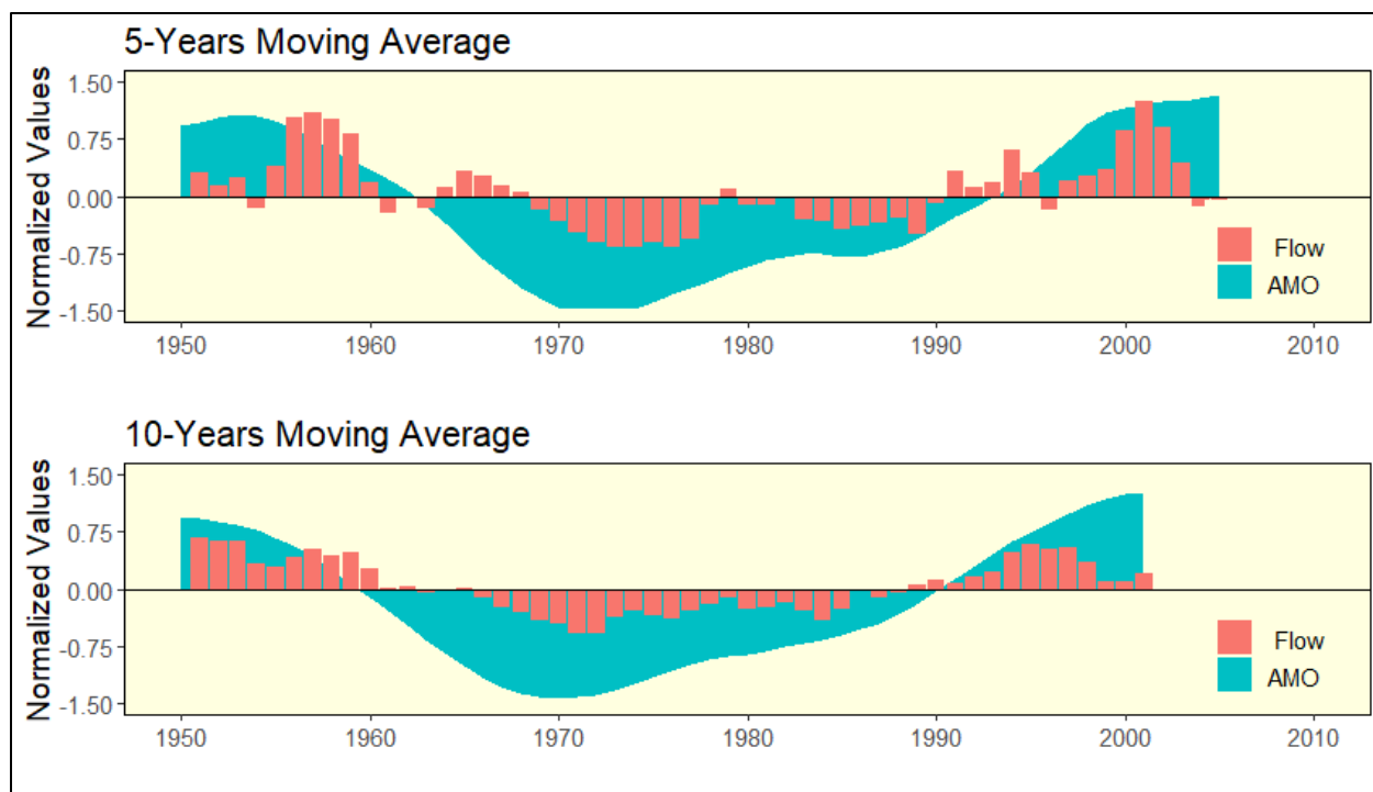
Figure 2-14. Normalized values of 5- and 10-year moving averages of annual AMO anomalies and flows at the USGS Horse Creek at SR 72 near Arcadia, FL (No. 022973100) gage for the period from 1951 through 2008.
