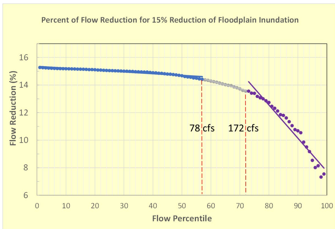
Figure 6-4. The sensitivity between the percent-of-flow reductions that would result in a 15% decrease in the amount of total inundated wetlands and river flow percentiles in Horse Creek. Note the fitting of 3 lines for low, mid and high flow percentile portions of the sensitivity curve.
