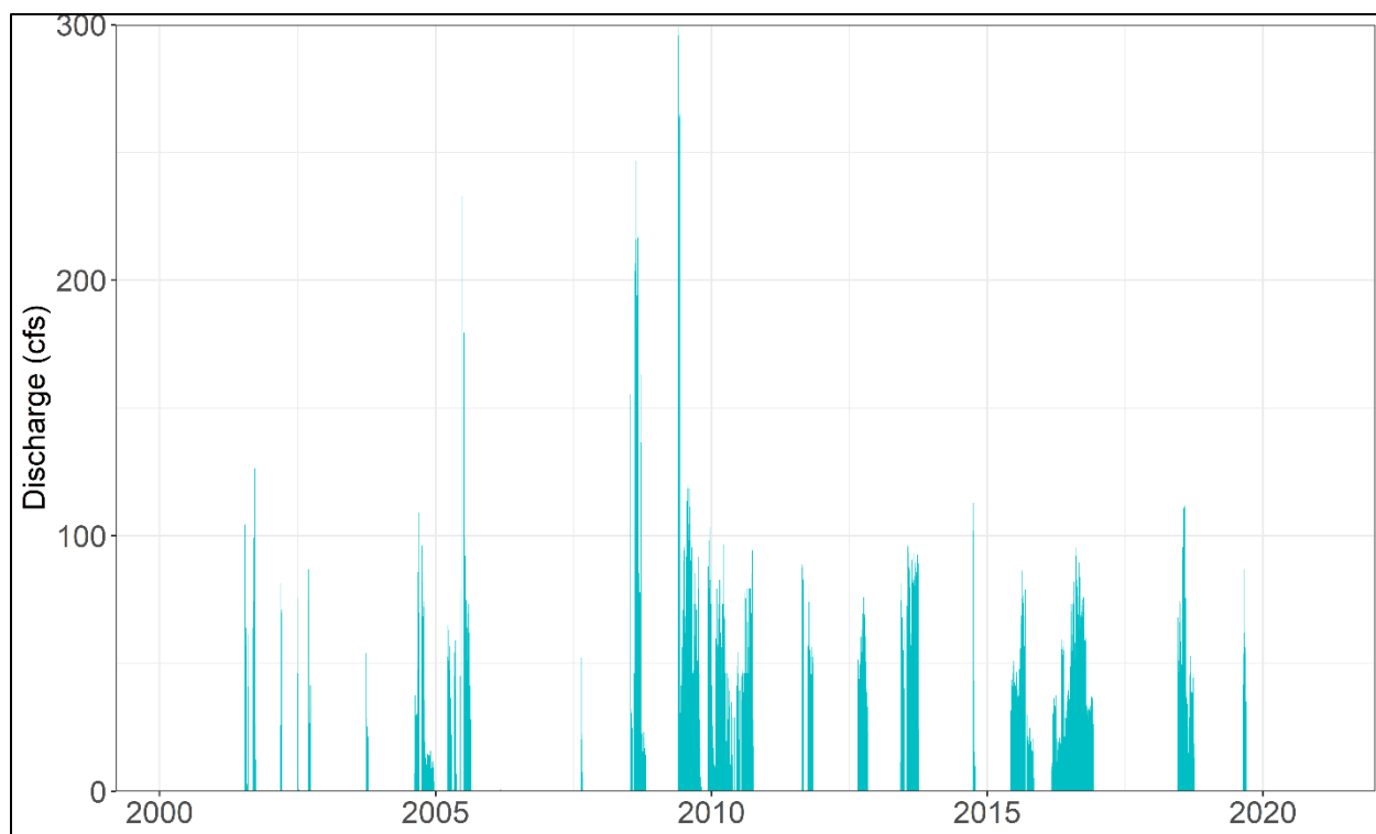
Figure 2-18. Combined daily National Pollutant Discharge Elimination System (NPDES) effluent discharges to Horse Creek from the Fort Green Mine (FTG-003) and Wingate (WIN-004) from 2000 through 2020.
