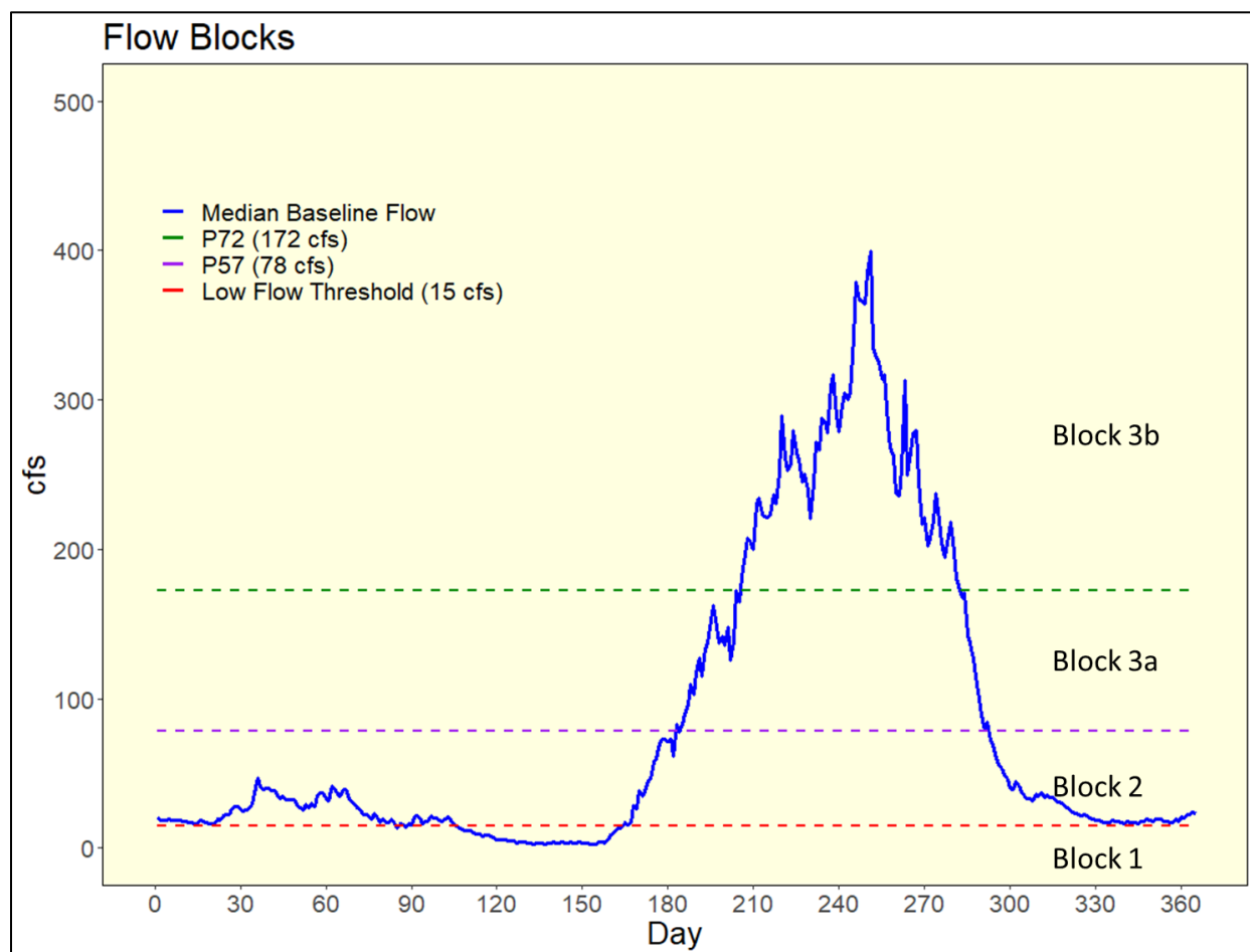
Figure 5-2. Flow blocks superimposed on a hydrograph of median observed daily, i.e., day of the calendar year, flows (solid blue line) at the USGS Horse Creek at SR 72 near Arcadia, FL (No. 02297310) gage. The high flow Block 3 is divided into two sub-blocks as shown by dashed green horizontal line. The boundary between the high-flow Block 3 and medium-flow Block 2 is shown as a purple dashed horizontal line. The boundary between medium-flow Block 2 and low-flow Block 1 is shown as a red dashed horizontal line. The median hydrograph is shown here for reference; blocks were determined based on fish passage and floodplain inundation criteria, not on the median flows.
