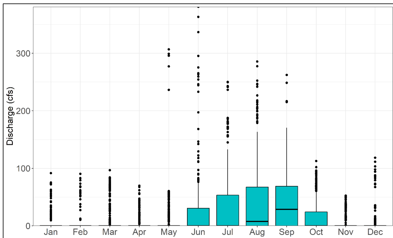
Figure 2-19. Monthly National Pollutant Discharge Elimination System (NPDES) effluent discharge from the Fort Green Mine (FTG-003) and Wingate (WIN-004) from 2000 through 2020. Boxed values indicate the 25 th to 75 th percentiles with the centerline reflecting the 50 th percentile value. Dots represent outliers, indicative of values outside of the 1.5*interquartile range.
