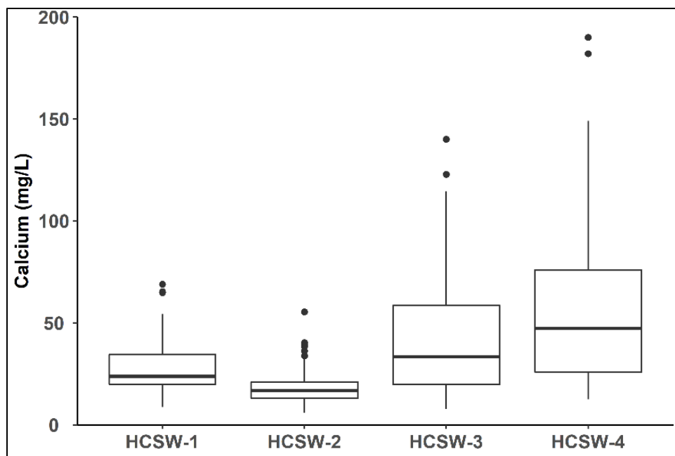
Figure 3-23. Dissolved calcium at HCSW stations from 2003-2018. Boxed values indicate the 25 th to 75 th percentiles with centerline reflecting the 50 th percentile value. Dots represent outliers, indicative of values outside of the 1.5*interquartile range.
