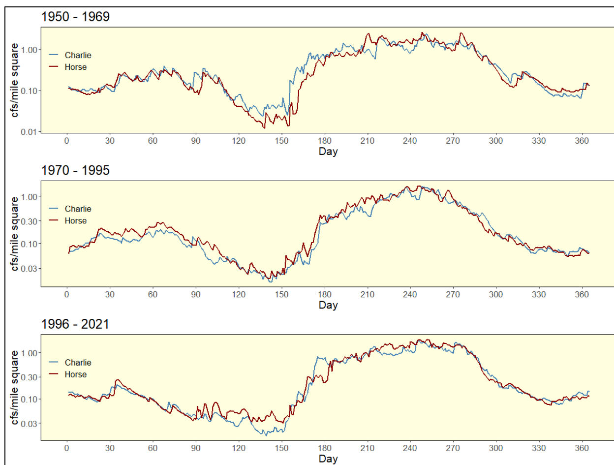
Figure 2-20. Comparison of median daily flows (logarithmic scale) for three time periods at the USGS Charlie Creek near Gardner, FL (No. 02296500) and USGS Horse Creek at SR 72 near Arcadia, FL (No. 02297310) gages. Data from 1950 begin on May 1 st .
