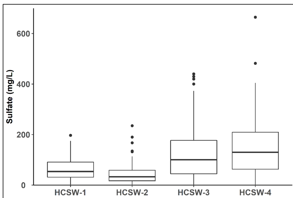
Figure 3-24. Total sulfate at HCSW stations from 2003-2018. Boxed values indicate the 25 th to 75 th percentiles with centerline reflecting the 50 th percentile value. Dots represent outliers, indicative of values outside of the 1.5*interquartile range.
