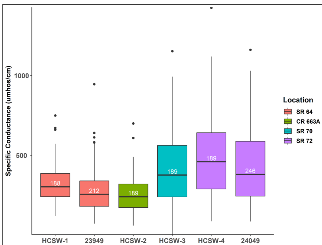
Figure 3-16. Specific conductance at stations with a similar period of record (POR). The HCSW stations (HCSW-1, -2, -3, and -4) have a POR of April 2003 through December 2018 and the District stations (23949 and 24049) have a POR from August 1997 through July 2019. The number of samples measured at each station is noted above the mean line. Stations are color-coded by their relative location since some stations are sampled at nearly the same coordinates. Boxed values indicate the 25 th to 75 th percentiles with centerline reflecting the 50 th percentile value. Dots represent outliers, indicative of values outside of the 1.5*interquartile range.
