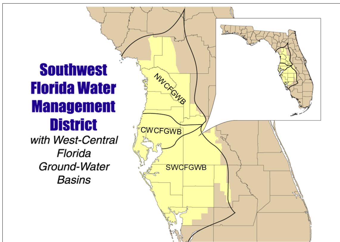
Figure 2-21. Location of regional groundwater basins within the District boundary, including the Northern West-Central Florida Groundwater Basin (NWCFGWB), the
