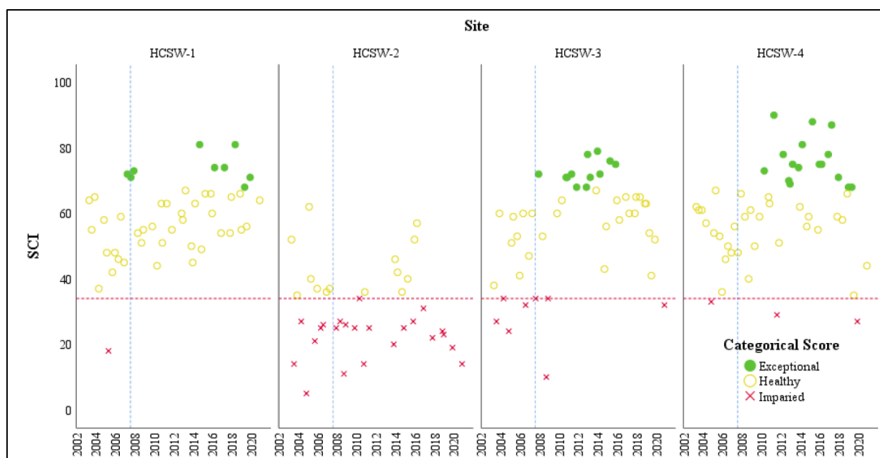
Figure 4-2. Stream Condition Index (SCI) scores for HCSW stations HCSW-1 through HCSW-4 over the period of record. The dashed vertical line designates a methods revision that occurred in 2007. Scores prior to 2007 are not compatible with those occurring later (Figure from Flatwoods 2021).
