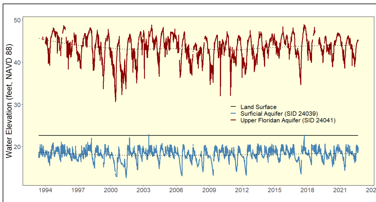
Figure 2-22. Water levels (feet) from monitor wells installed into the surficial and Upper Floridan aquifers at the District Regional Observation and Monitor-Well Program 17 site from 1993 through August 2022. The dashed lines indicate the overall trend using LOESS.
