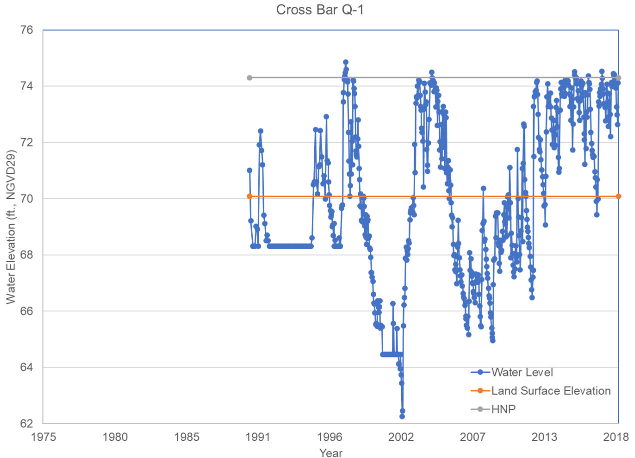
Figure 29: Cross Bar Q-1 water levels
