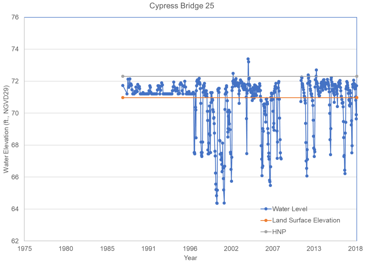
Figure 36: Cypress Bridge 25 water levels
