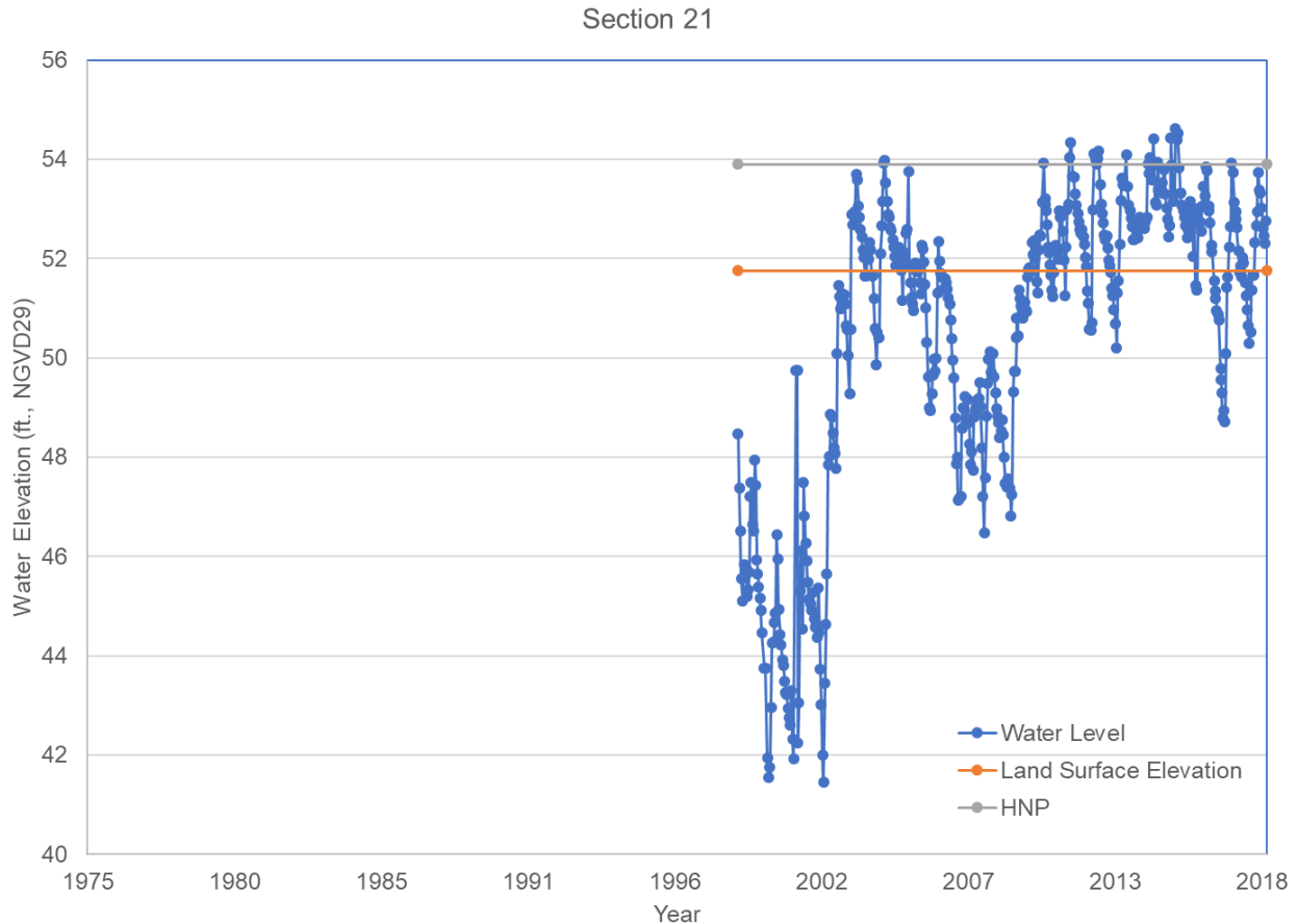
Figure 76: Section 21 WF NW-53 water levels
