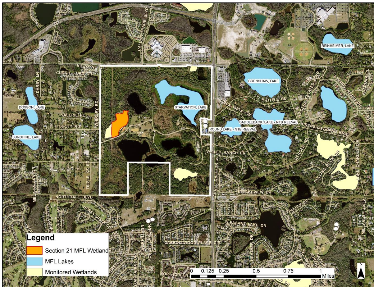
Figure 77: Section 21 WF NW-53 Wetland and surrounding lakes with established minimum levels
