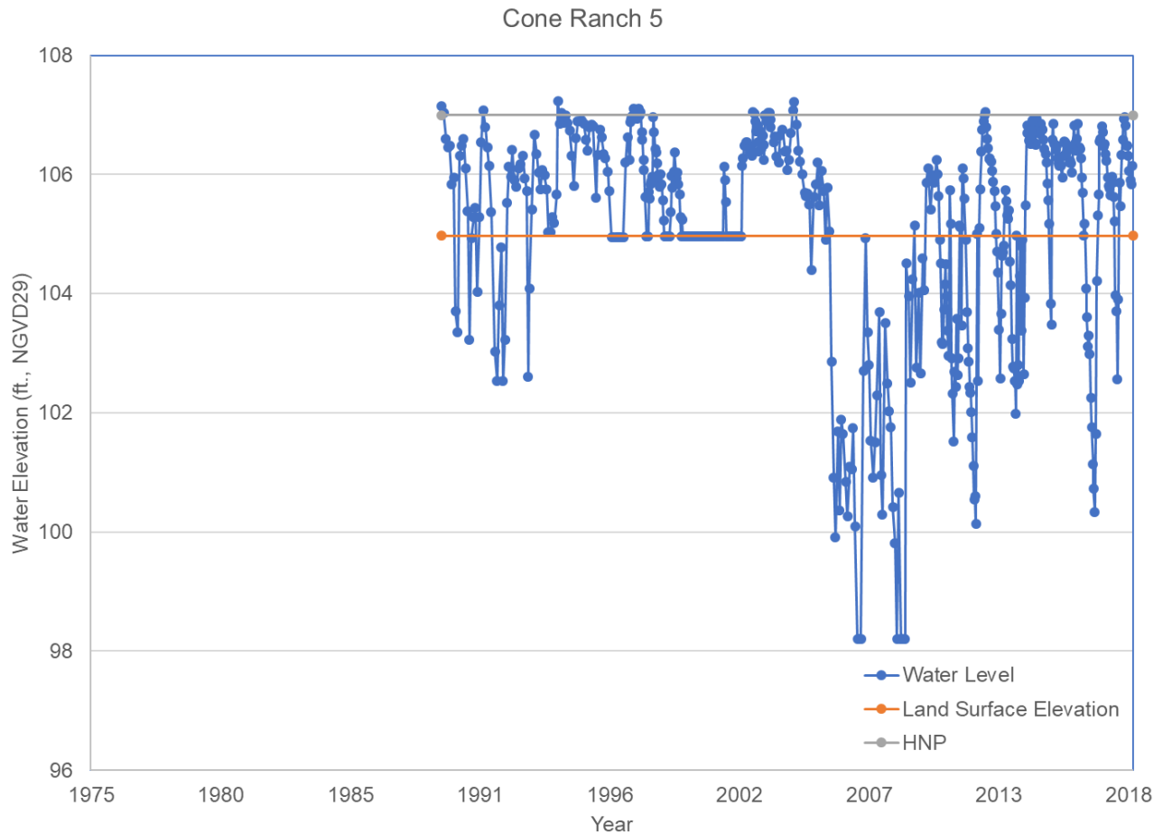
Figure 13: Cone Ranch 5 water levels
