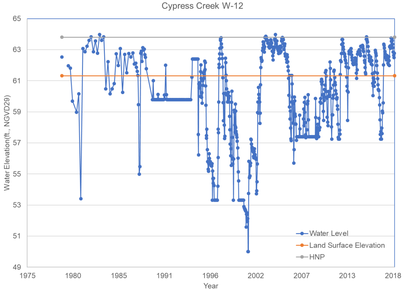
Figure 48: Cypress Creek W-12 water levels
