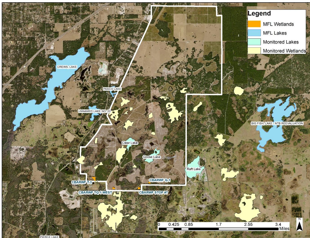
Figure 27: MFL and monitored sites in the Cross Bar wellfield area. Note the Cross Bar TQ-1 West is no longer an adopted MFL, but remains a monitored wetland.
