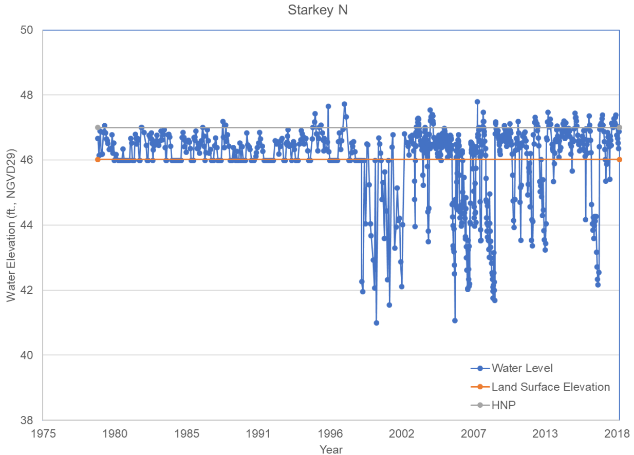
Figure 102: Starkey N water levels
