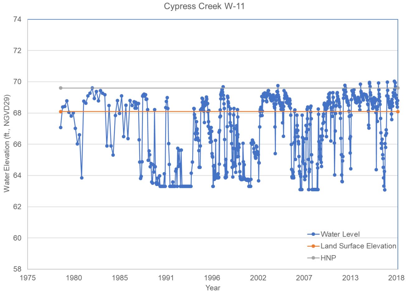
Figure 46: Cypress Creek W-11 water levels
