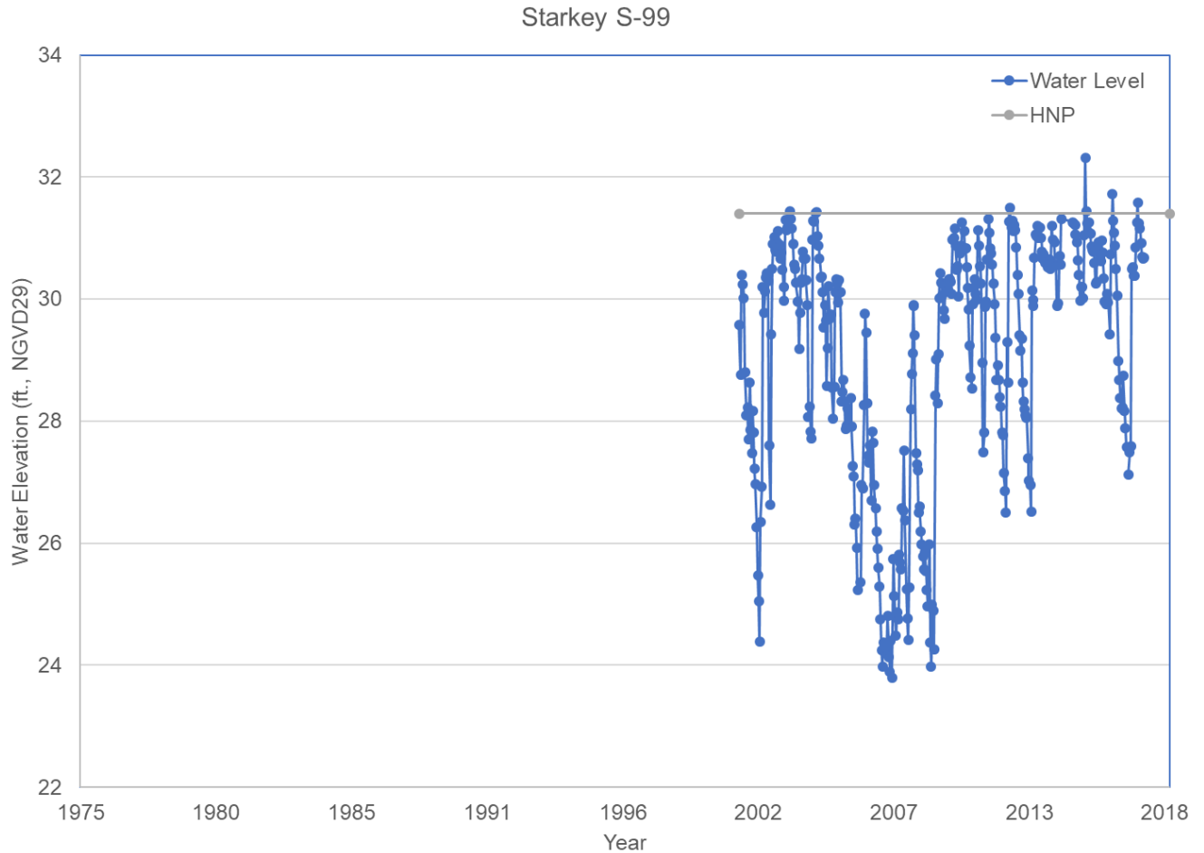
Figure 90: Starkey S-99 water levels
