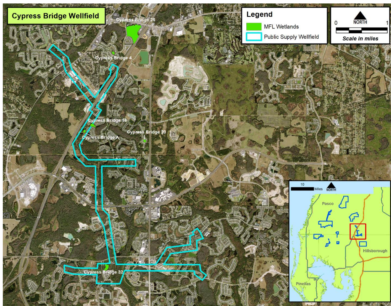
Figure 30: Cypress Bridge wellfield with established minimum level wetlands
