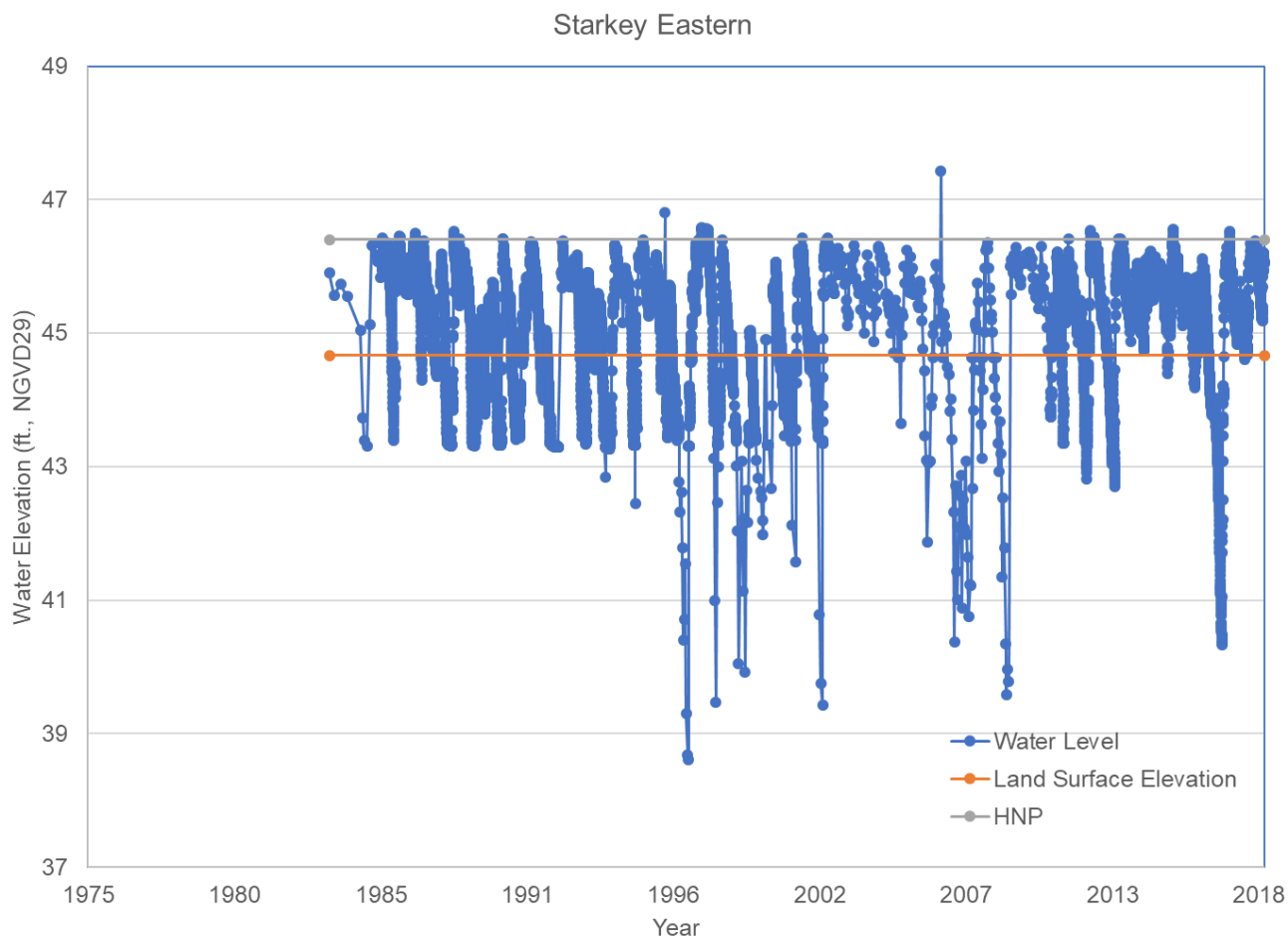
Figure 96: Starkey Eastern water levels
