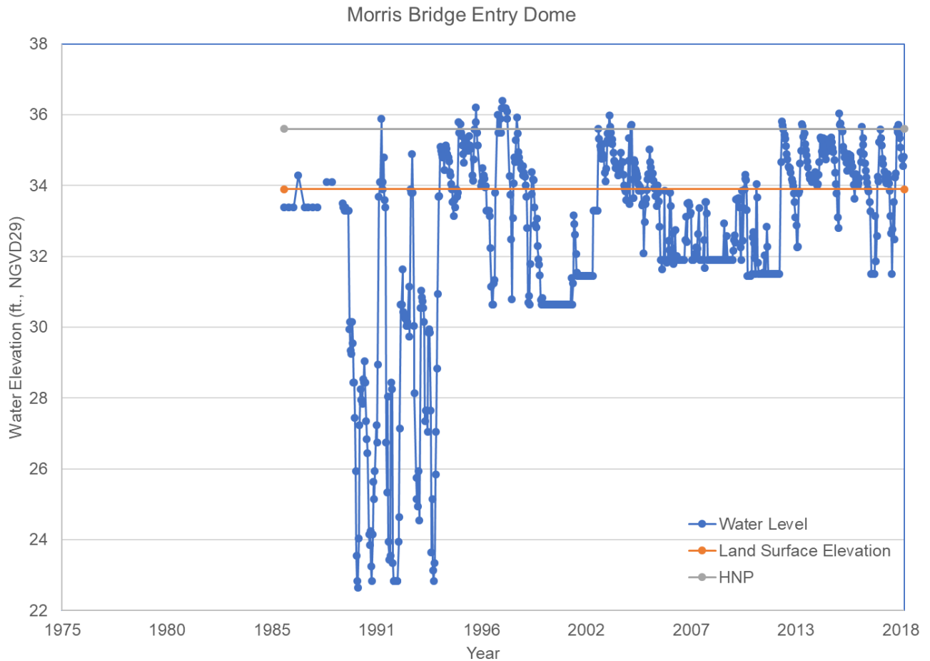
Figure 62: Morris Bridge Entry Dome water levels
