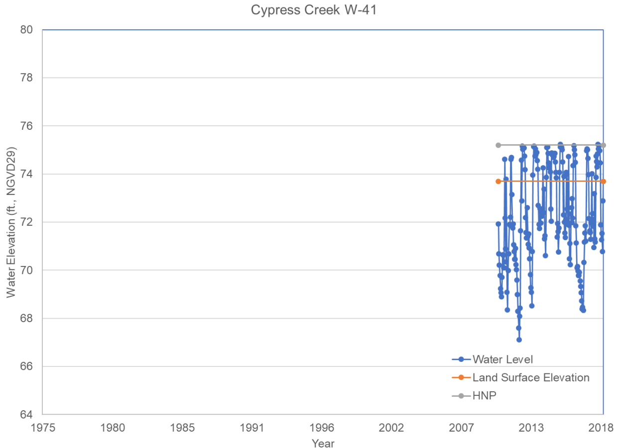
Figure 44: Cypress Creek W-41 water levels. Note: elevation on vertical axis goes higher than on other Cypress Creek hydrographs.
