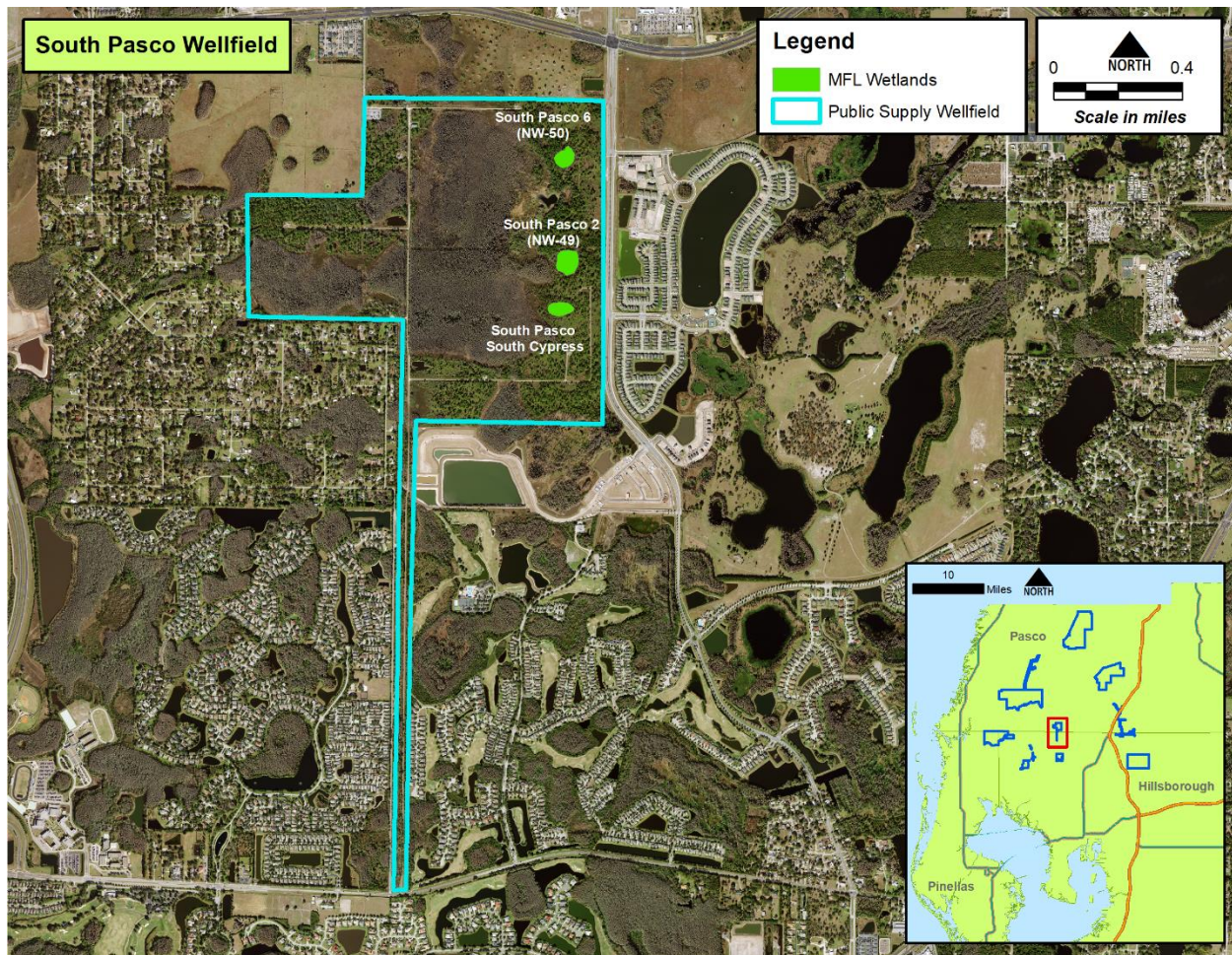
Figure 78: South Pasco Wellfield with established minimum level wetlands
