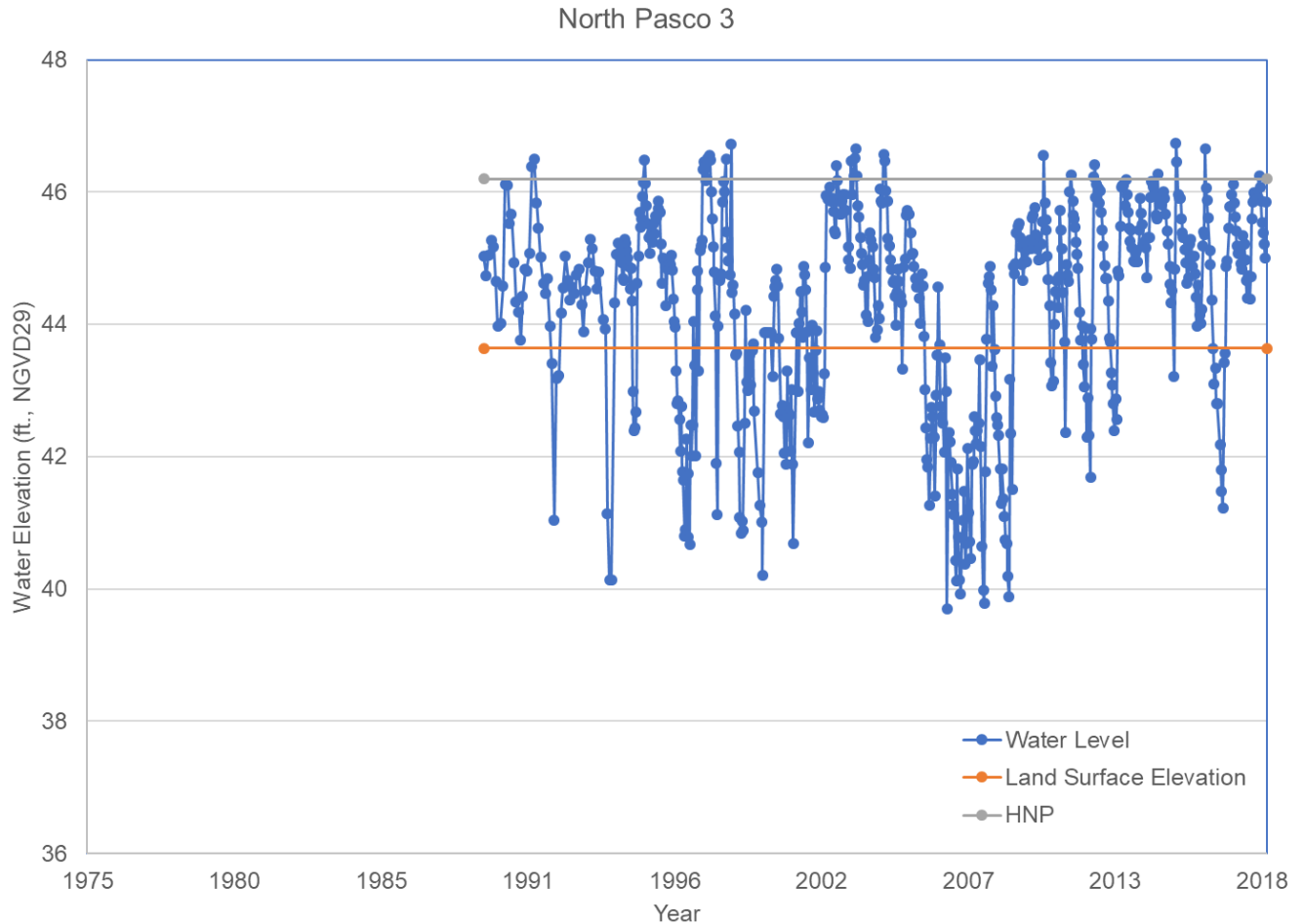
Figure 71: North Pasco 3 water levels
