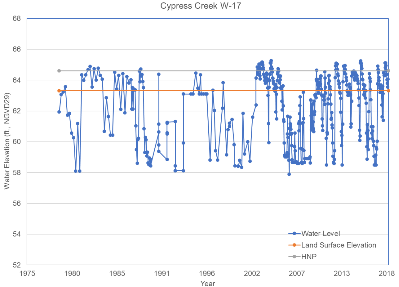
Figure 50: Cypress Creek W-17 water levels
