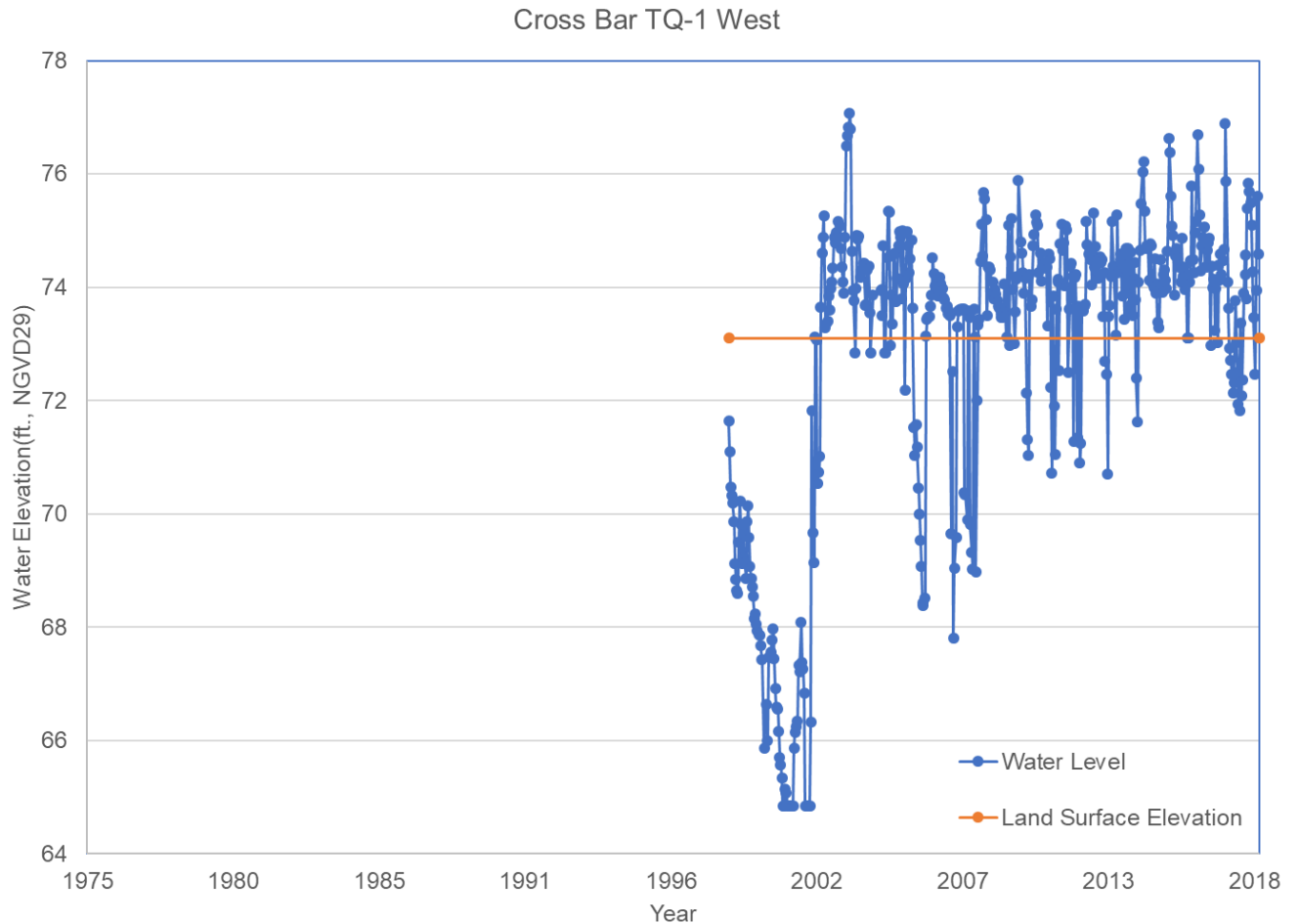
Figure 22: Cross Bar TQ-1 West water levels
