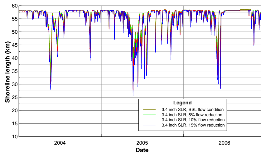
Figure B44 Daily shoreline length of water: salinity range 0-15ppt, 3.4 inch SLR.
