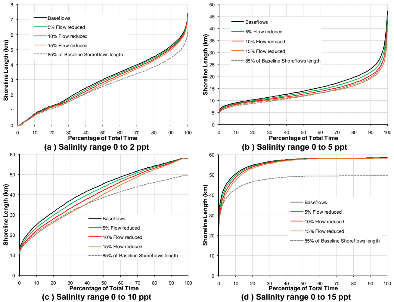
Figure 11 Shoreline length analysis CDF's: SLR 3.4 inches.
