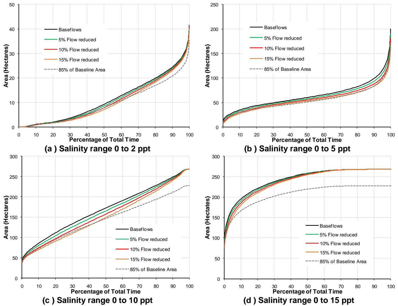
Figure 14 Bottom area analysis CDF's: SLR 7.7 inches.
