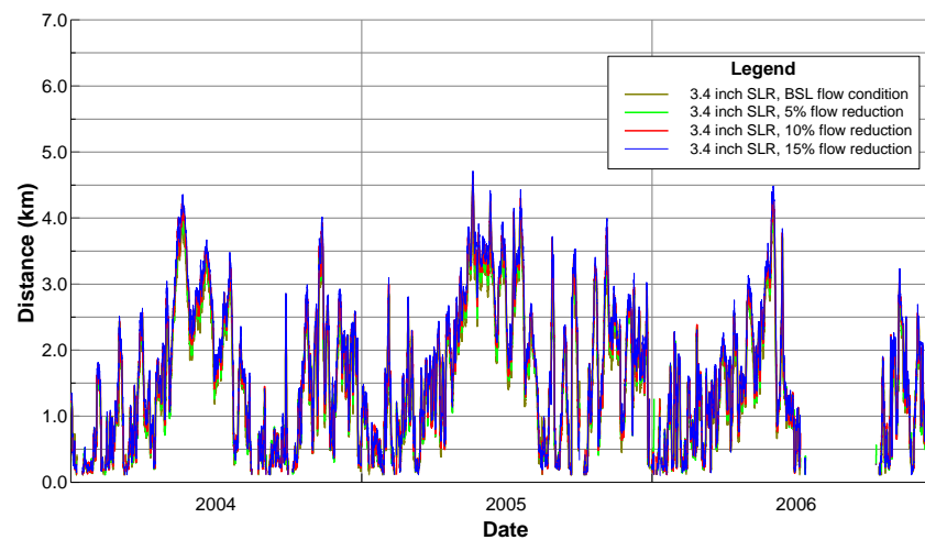
Figure B60 Daily isohaline location of water: salinity range 0-15ppt, 3.4 inch SLR.
