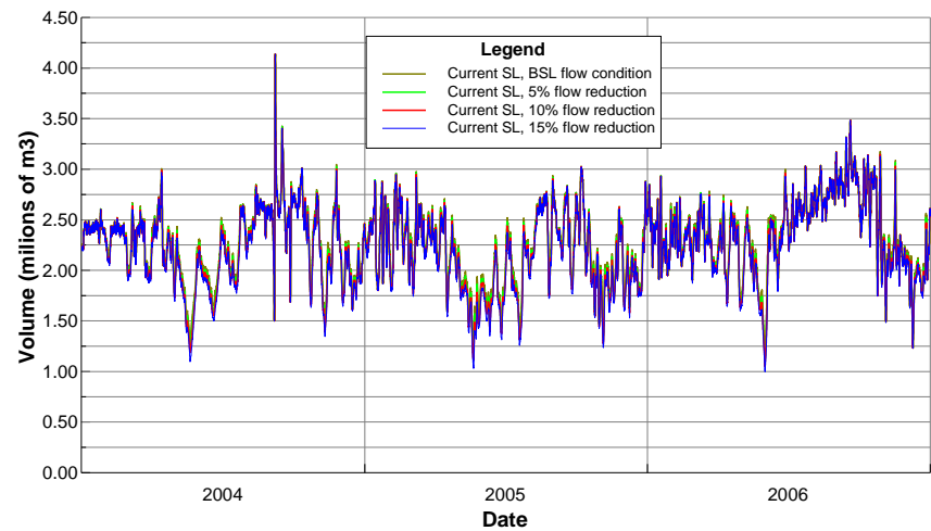
Figure B4 Daily volume of water: salinity range 0-15ppt, current sea level.
