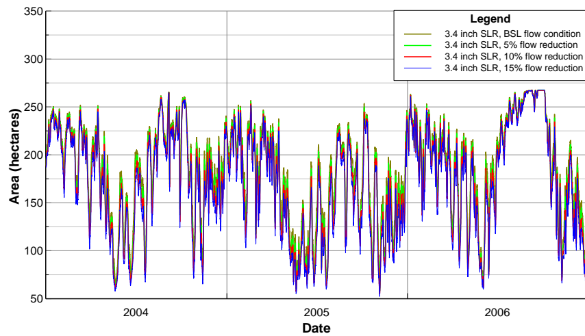
Figure B27 Daily Bottom area of water: salinity range 0-10ppt, 3.4 inch SLR.
