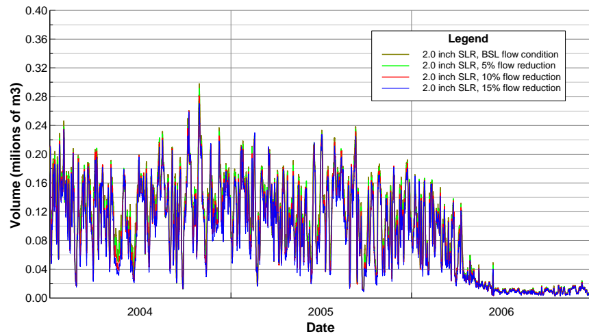
Figure B5 Daily volume of water: salinity range 0-2ppt, 2.0 inch SLR.
