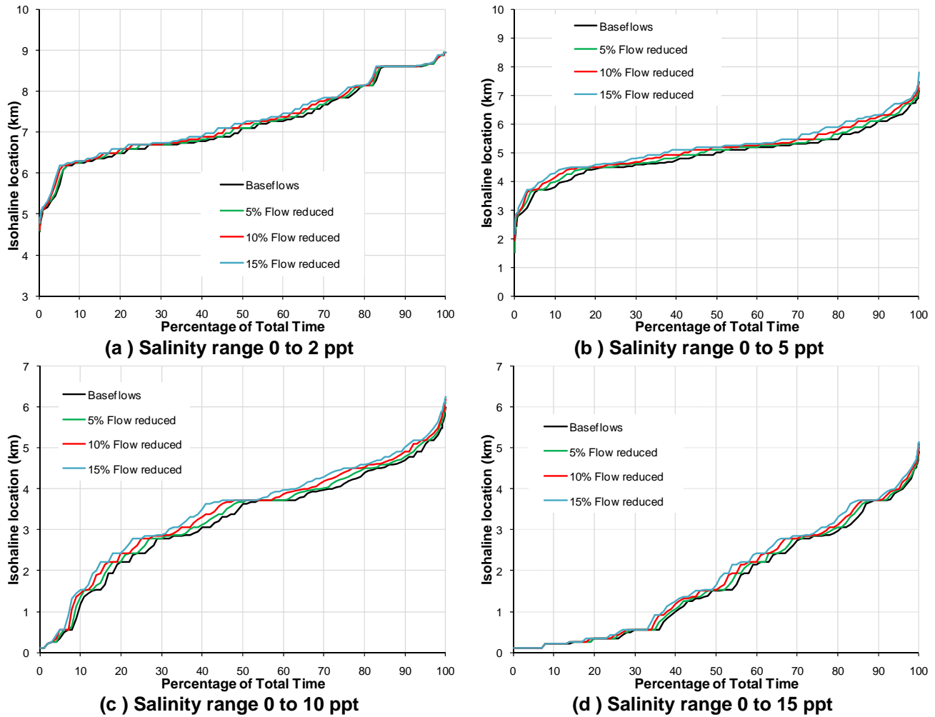
Figure 12 Isohaline location analysis CDF's: SLR 3.4 inches.
