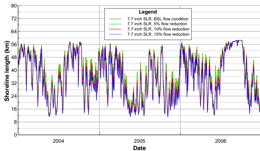
Figure B47 Daily shoreline length of water: salinity range 0-10ppt, 7.7 inch SLR.
