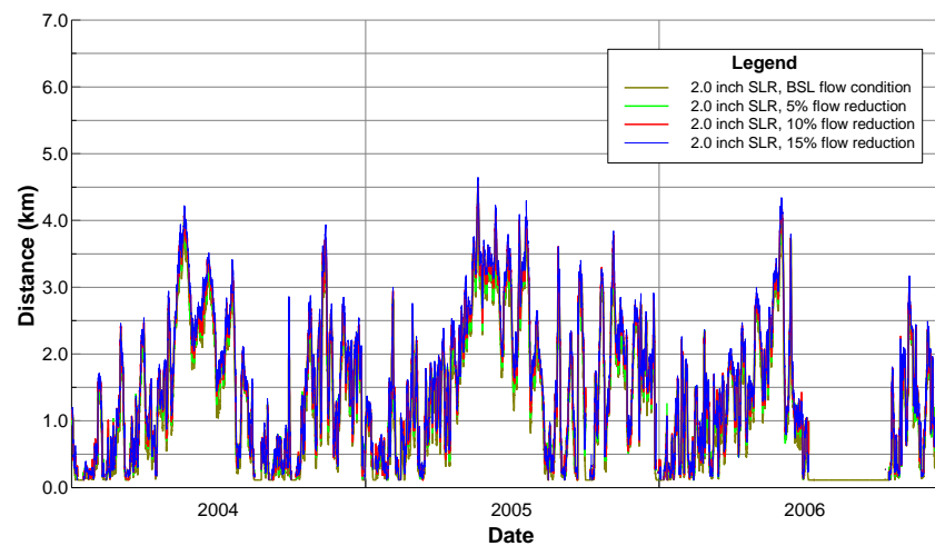
Figure B56 Daily isohaline location of water: salinity range 0-15ppt, 2.0 inch SLR.
