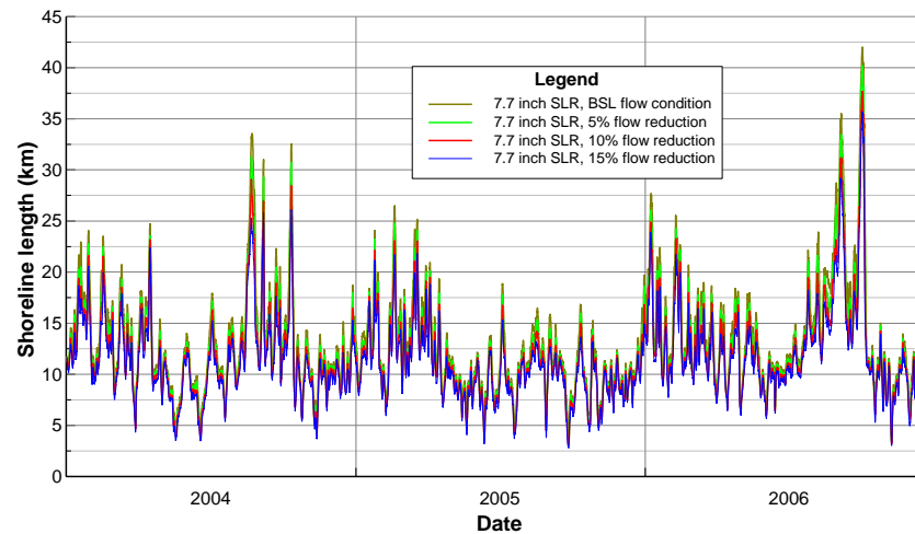
Figure B46 Daily shoreline length of water: salinity range 0-5ppt, 7.7 inch SLR.
