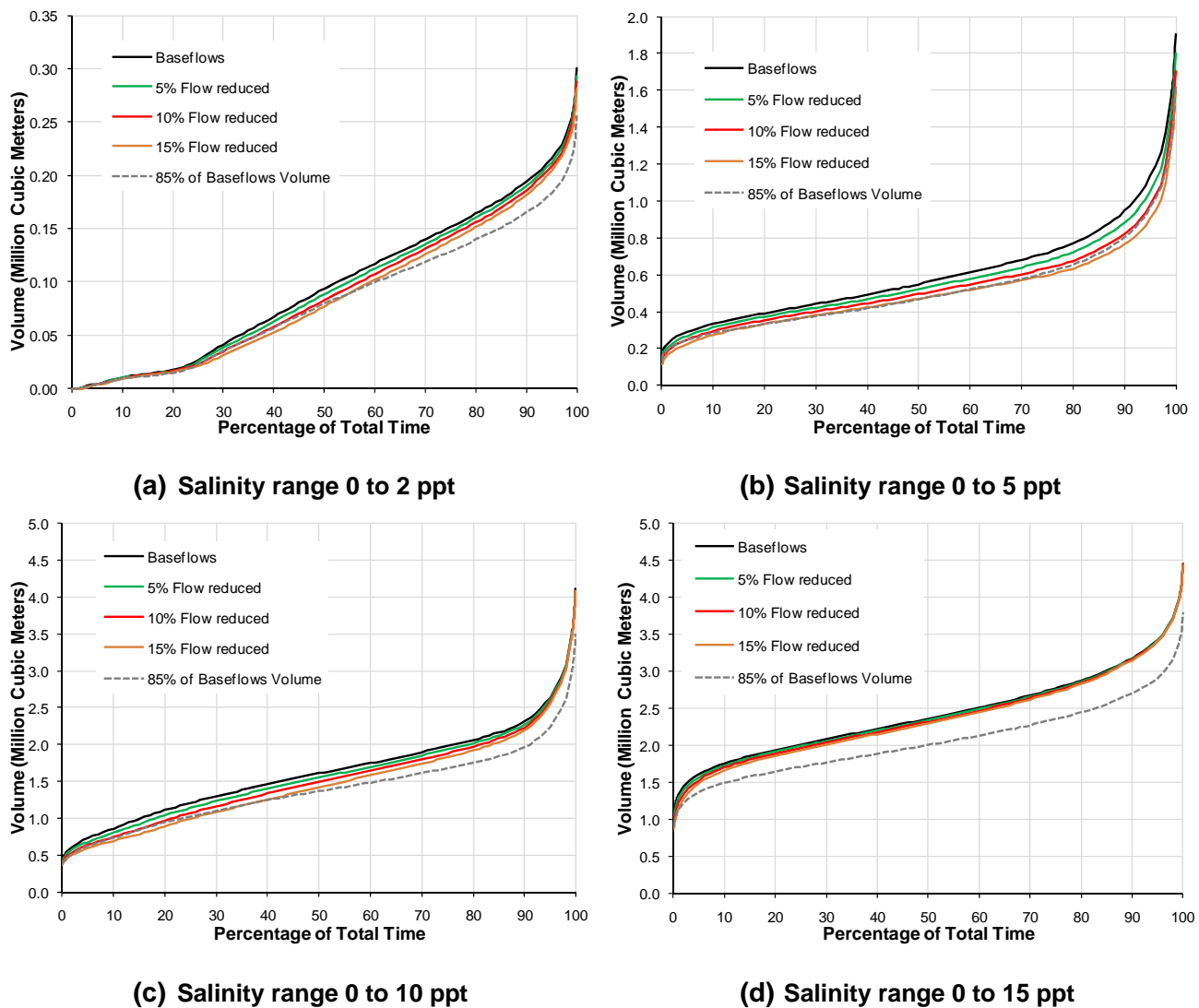
Figure 9 Volumetric analysis CDF's: SLR 3.4 inches
