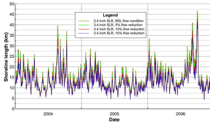
Figure B42 Daily shoreline length of water: salinity range 0-5ppt, 3.4 inch SLR.
