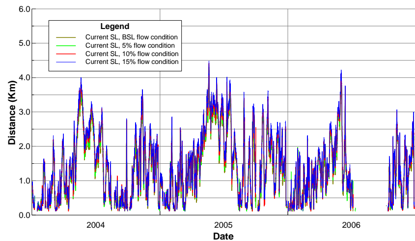
Figure B52 Daily isohaline location of water: salinity range 0-15ppt, current sea level.
