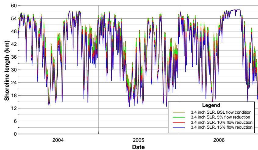
Figure B43 Daily shoreline length of water: salinity range 0-10ppt, 3.4 inch SLR.
