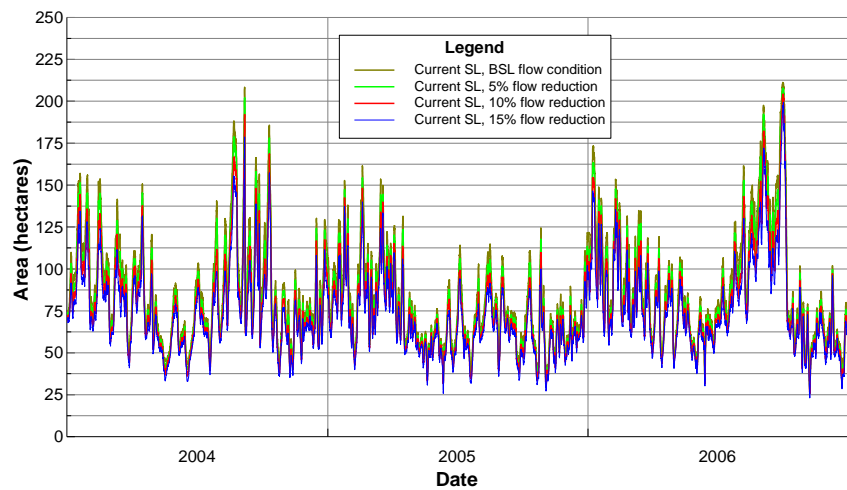
Figure B18 Daily Bottom area of water: salinity range 0-5ppt, current sea level.
