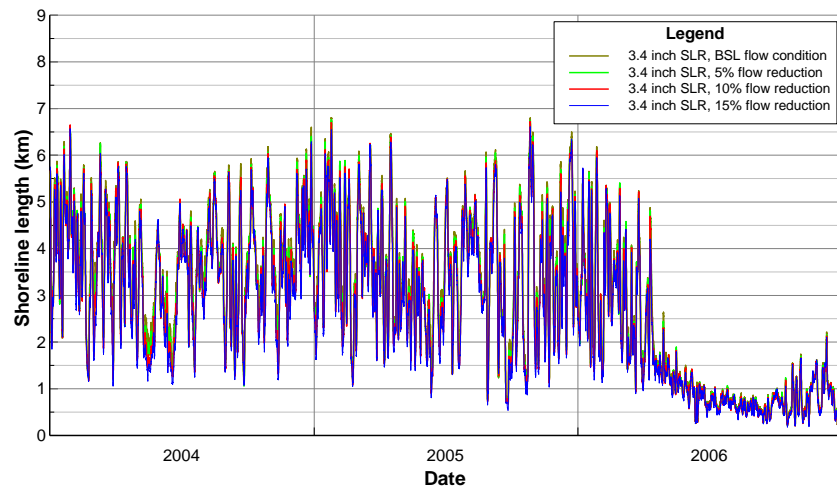
Figure B41 Daily shoreline length of water: salinity range 0-2ppt, 3.4 inch SLR.
