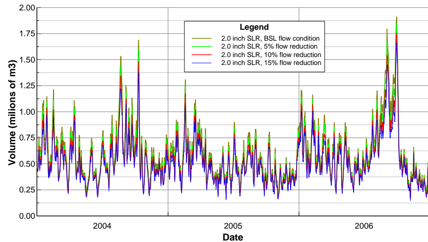
Figure B6 Daily volume of water: salinity range 0-5ppt, 2.0 inch SLR.
