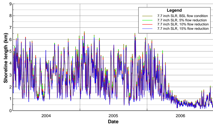
Figure B45 Daily shoreline length of water: salinity range 0-2ppt, 7.7 inch SLR.
