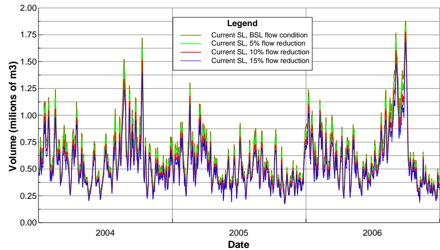
Figure B2 Daily volume of water: salinity range 0-5ppt, current sea level.
