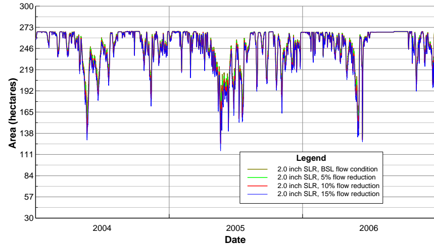
Figure B24 Daily Bottom area of water: salinity range 0-15ppt, 2.0 inch SLR.
