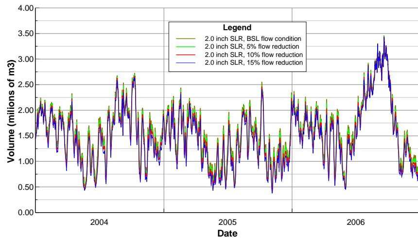
Figure B7 Daily volume of water: salinity range 0-10ppt, 2.0 inch SLR.
