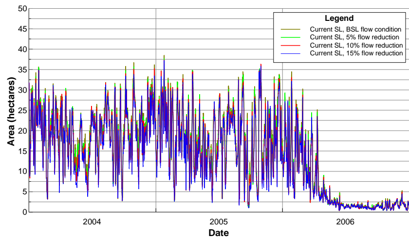
Figure B17 Daily Bottom area of water: salinity range 0-2ppt, current sea level.
