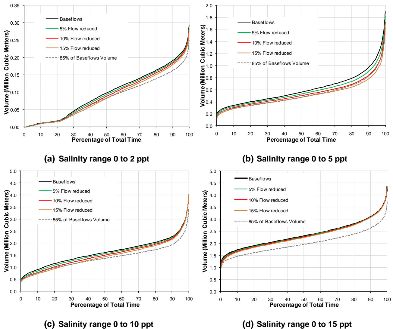
Figure 5 Volumetric analysis CDF's: SLR 2.0 inches
