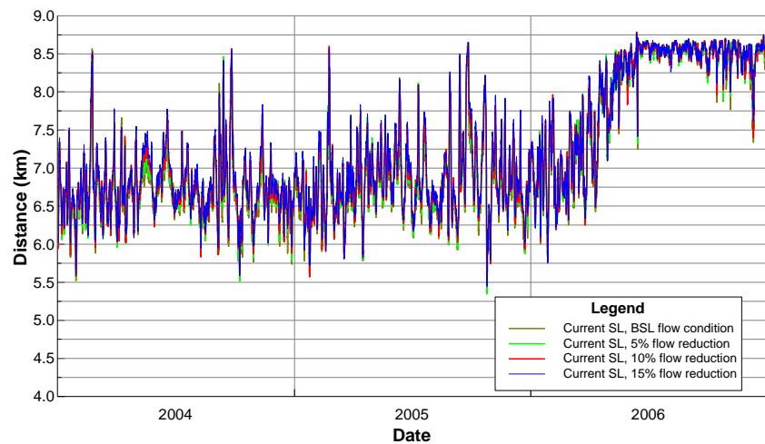
Figure B49 Daily isohaline location of water: salinity range 0-2ppt, current sea level.
