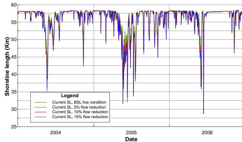
Figure B36 Daily shoreline length of water: salinity range 0-15ppt, current sea level.
