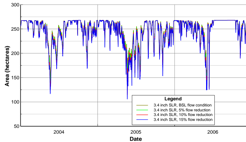
Figure B28 Daily Bottom area of water: salinity range 0-15ppt, 3.4 inch SLR.
