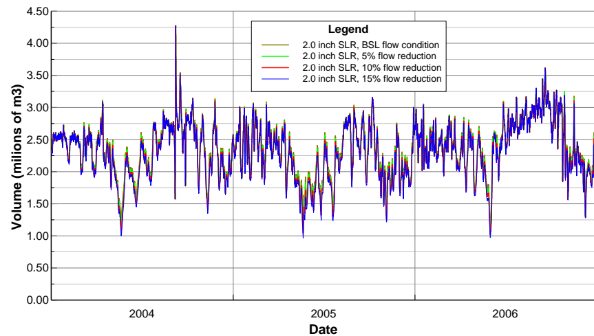
Figure B8 Daily volume of water: salinity range 0-15ppt, 2.0 inch SLR.
