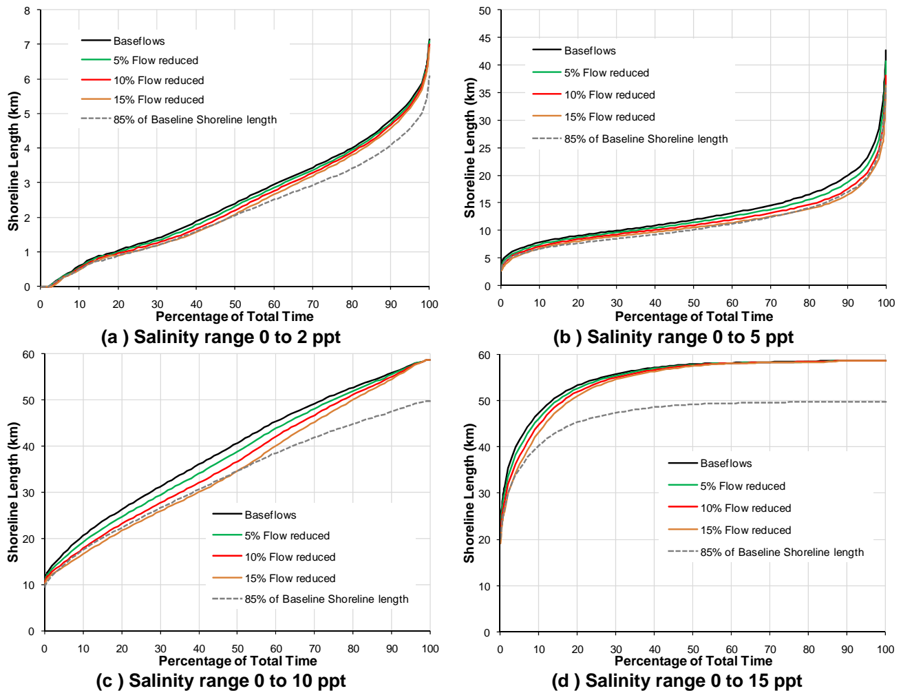
Figure 15 Shoreline length analysis CDF's: SLR 7.7 inches.
