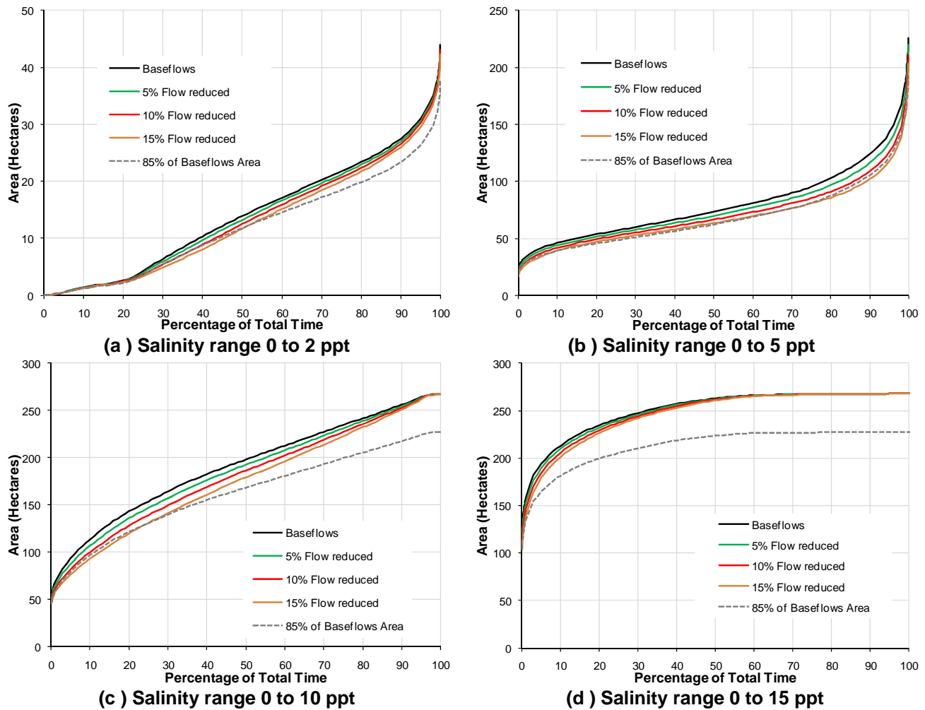
Figure 6 Bottom area analysis CDF's: SLR 2.0 inches.
