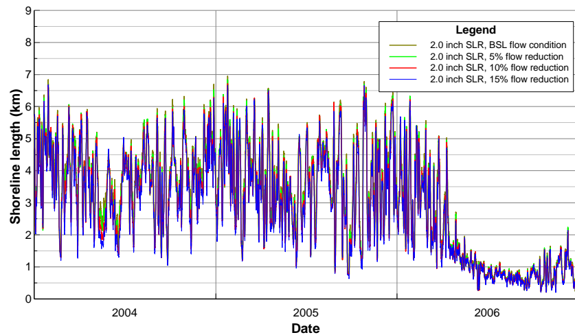
Figure B37 Daily shoreline length of water: salinity range 0-2ppt, 2.0 inch SLR.
