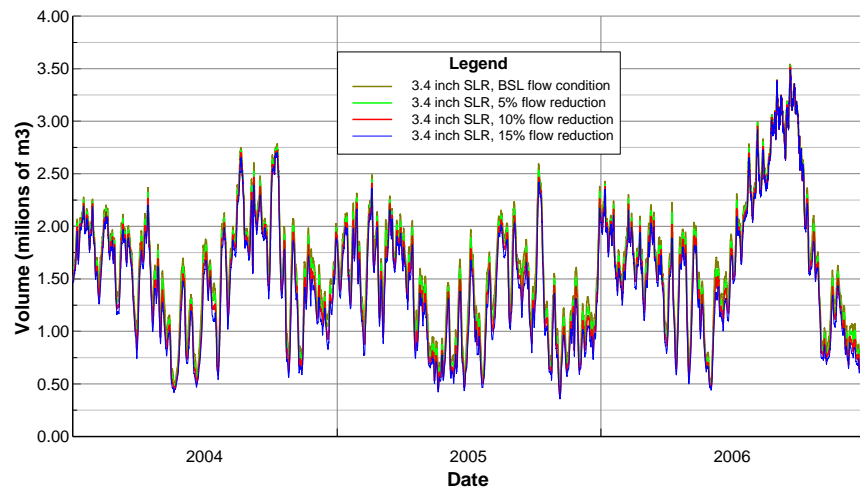
Figure B11 Daily volume of water: salinity range 0-10ppt, 3.4 inch SLR.
