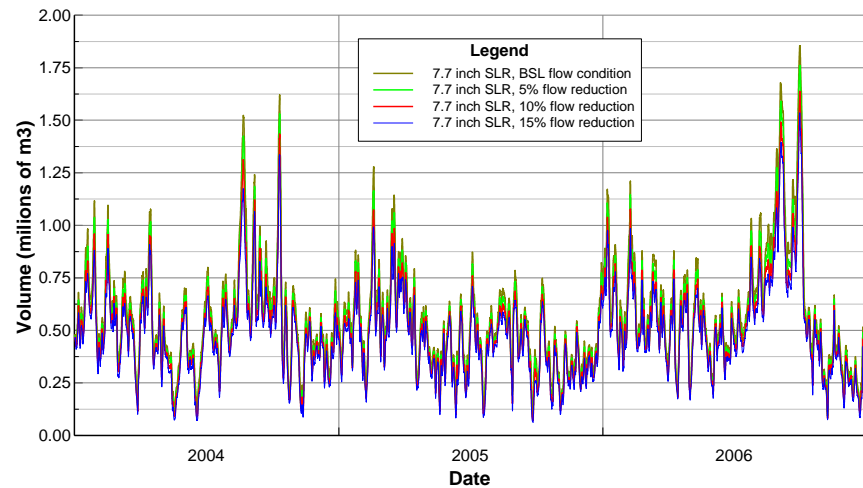
Figure B14 Daily volume of water: salinity range 0-5ppt, 7.7 inch SLR.
