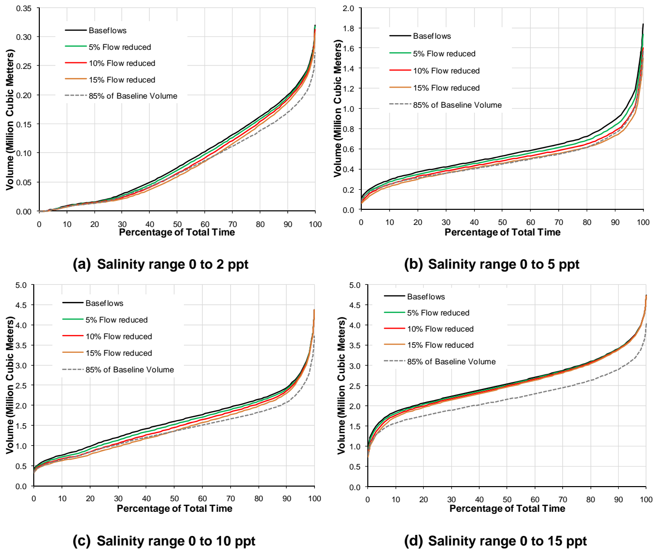
Figure 13 Volumetric analysis CDF's: SLR 7.7 inches
