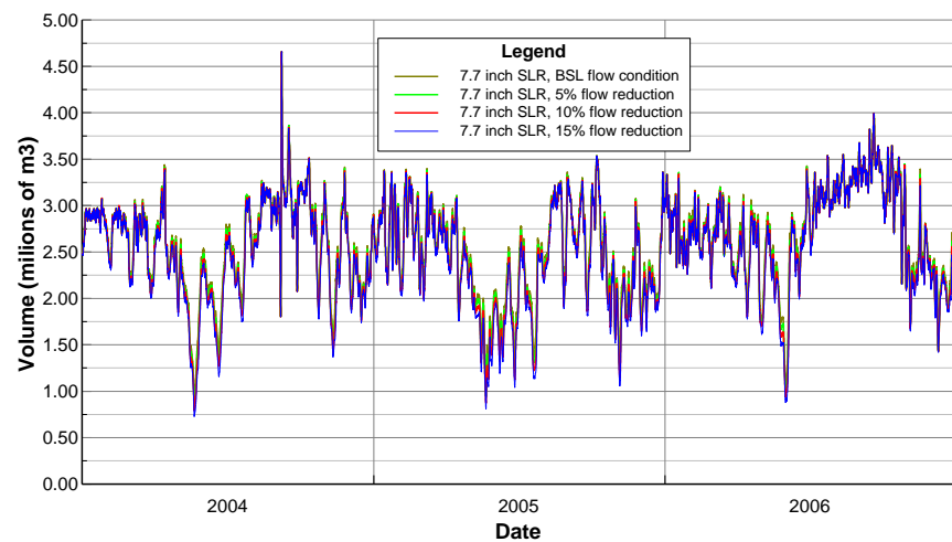
Figure B16 Daily volume of water: salinity range 0-15ppt, 7.7 inch SLR.
