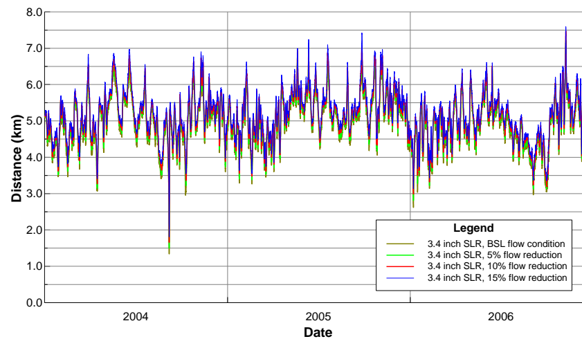
Figure B58 Daily isohaline location of water: salinity range 0-5ppt, 3.4 inch SLR.
