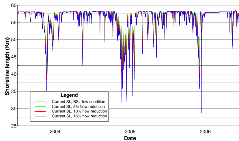
Figure B36 Daily shoreline length of water: salinity range 0-15ppt, current sea level.
