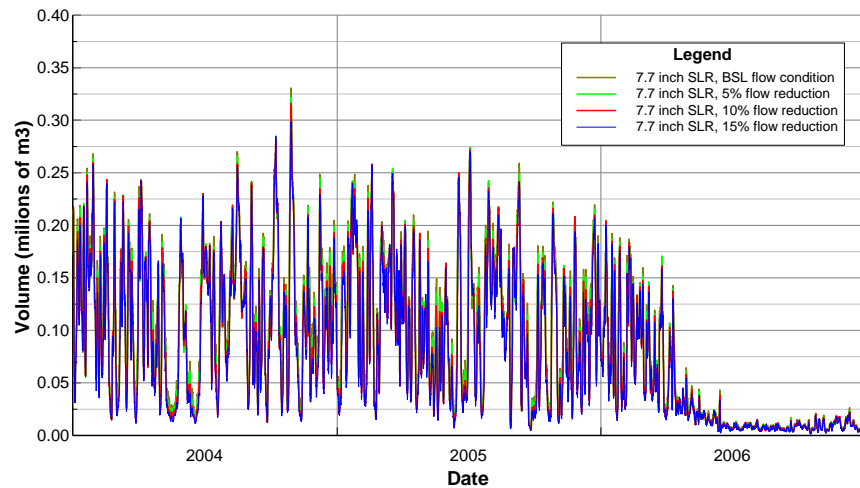
Figure B13 Daily volume of water: salinity range 0-2ppt, 7.7 inch SLR.
