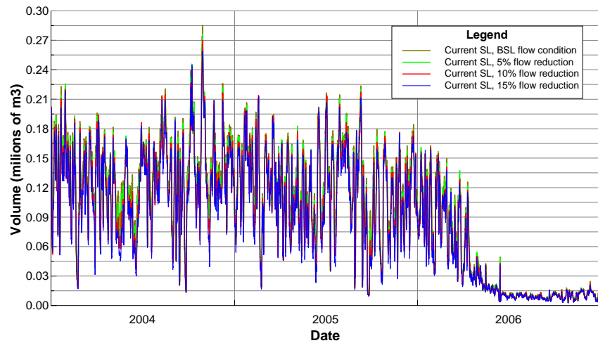
Figure B1 Daily volume of water: salinity range 0-2ppt, current sea level.
