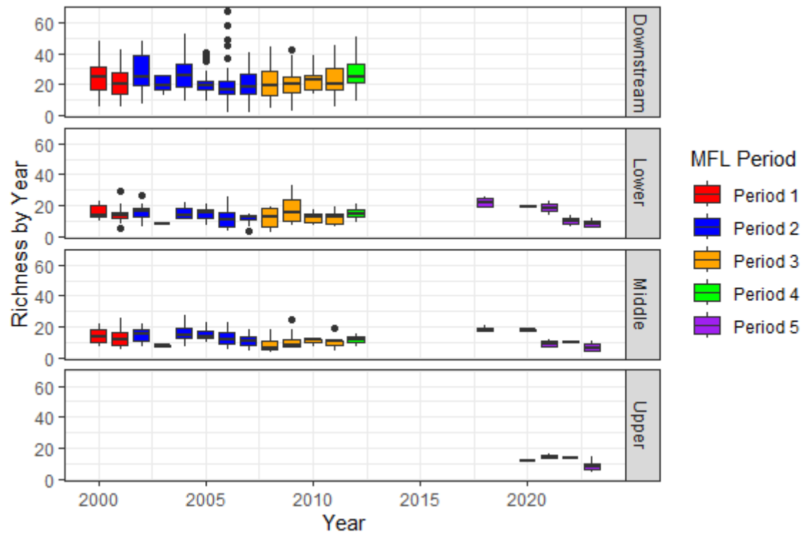
3.4.2.4 Boxplot of site level richness by MFL period and river segment.
