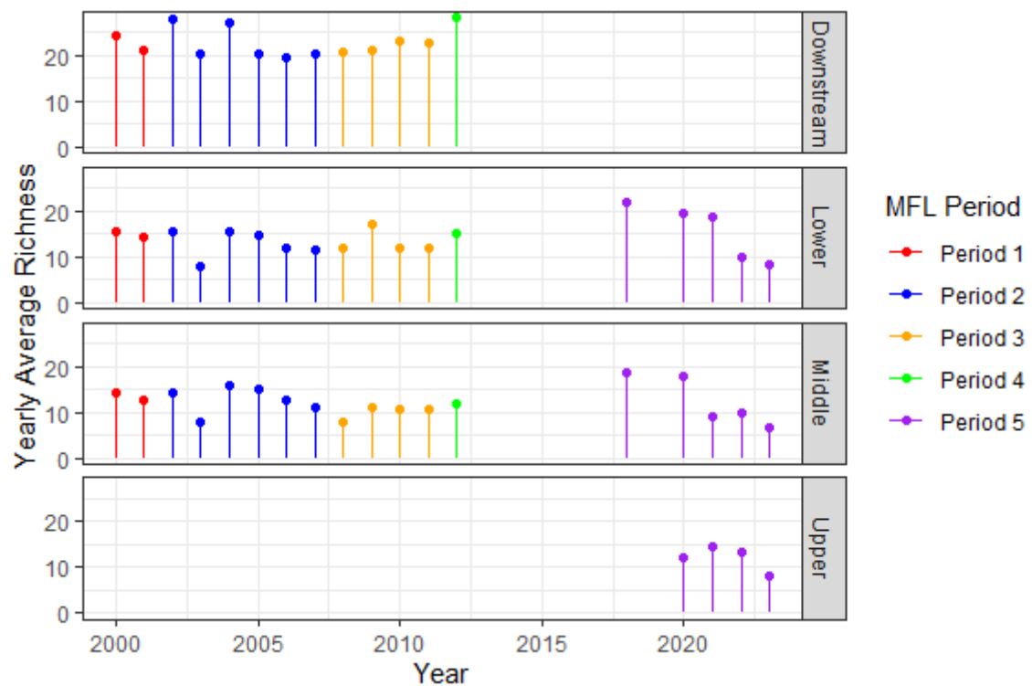
3.4.2.2 Average richness over time, grouped by year of samplin, by MFL period and river segment.
