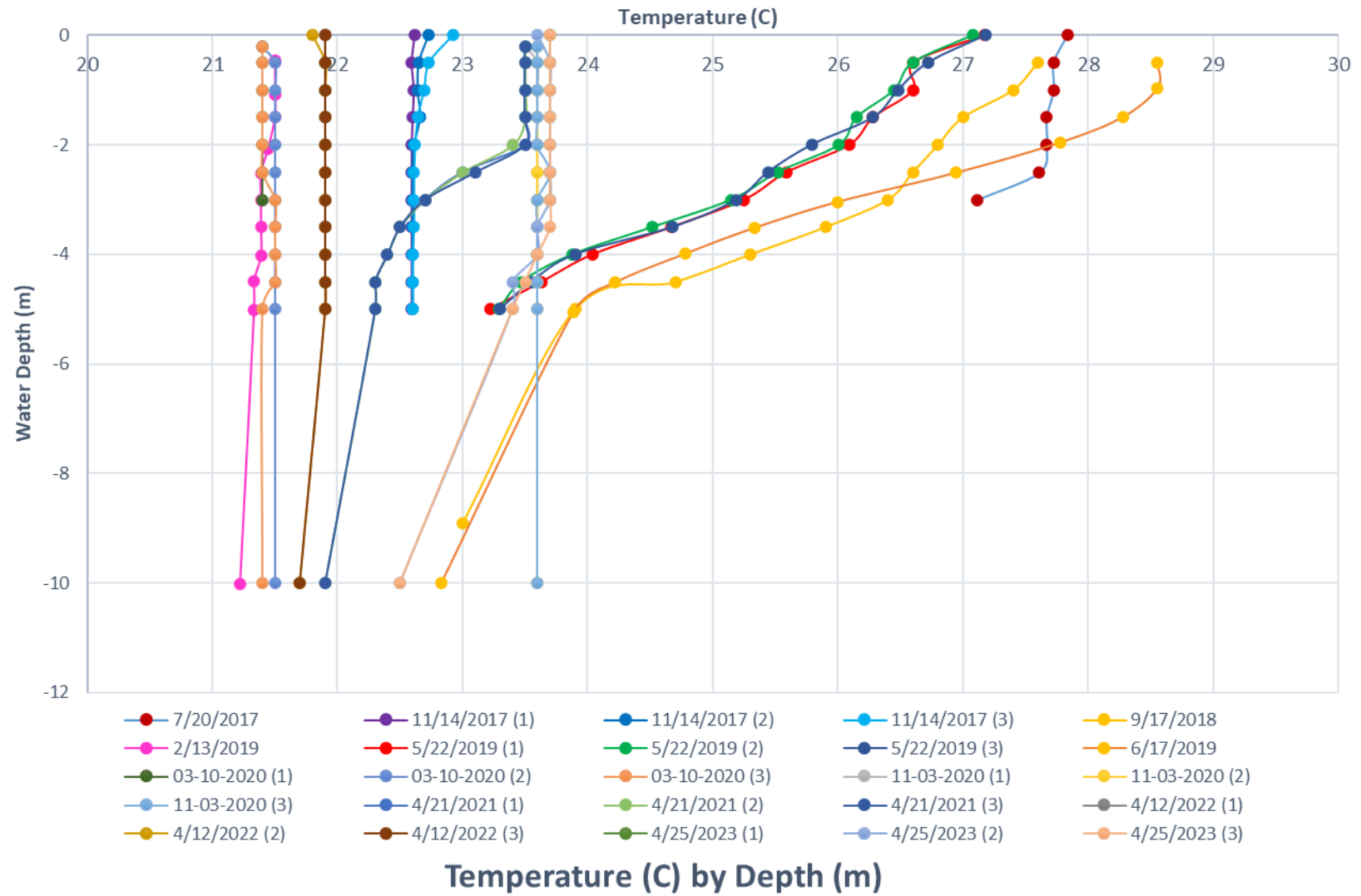
Figure 6-2 Consolidated Water Quality Data Graphs (2017–2023)
