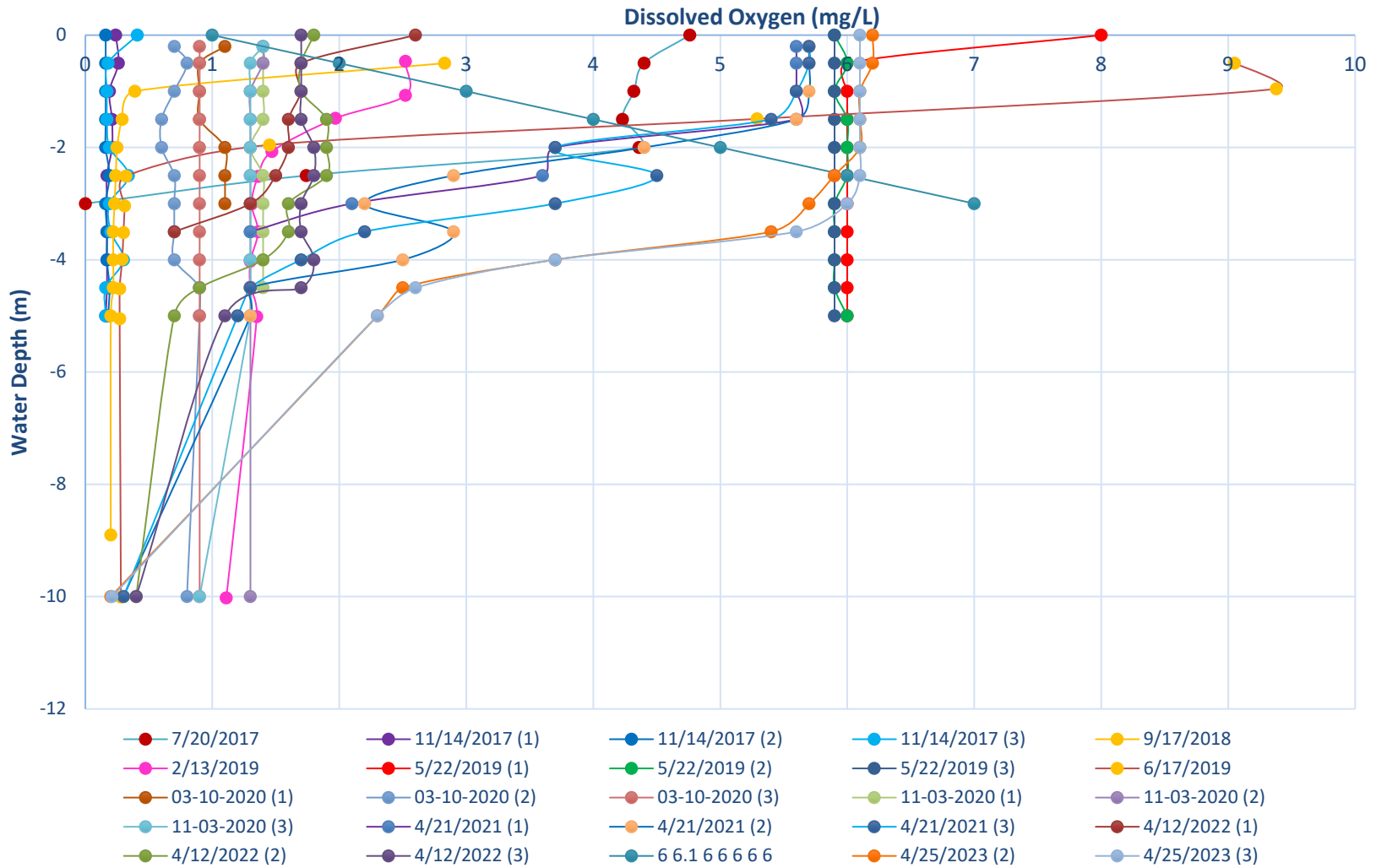
Dissolved Oxygen (mg/L) by Depth (m)
