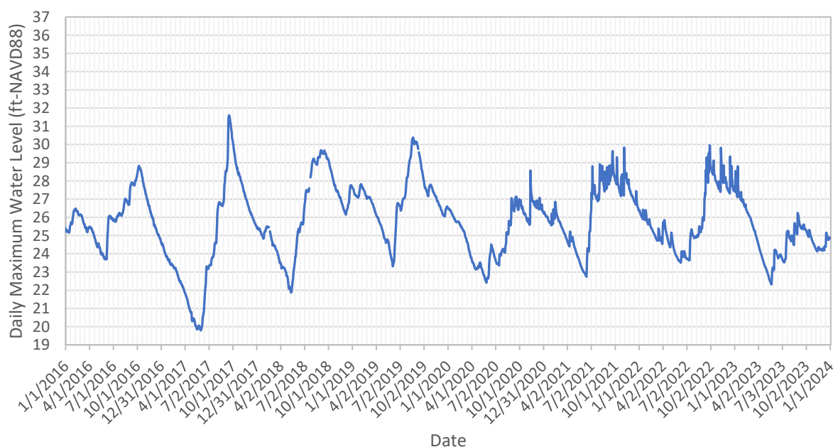
Figure 9 Surficial Aquifer Levels Northwest of Nursery Sink (SID 637851, DID 12)
