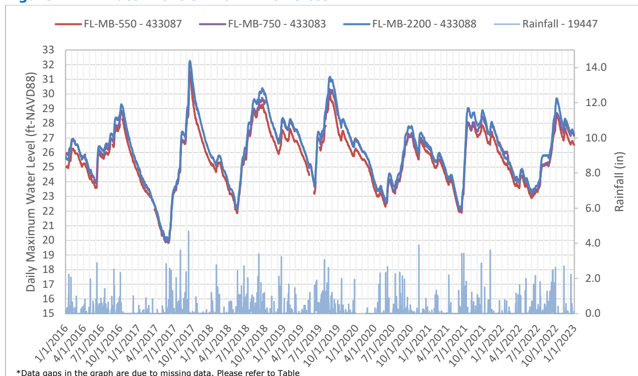
Figure 4-2 Water Levels in UFA Well Sites
