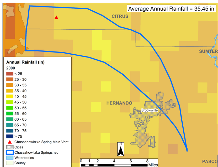
2000 Annual Rainfall Distribution within the Chassahowitzka Springshed
