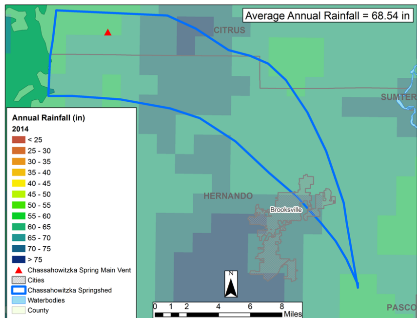
2014 Annual Rainfall Distribution within the Chassahowitzka Springshed
