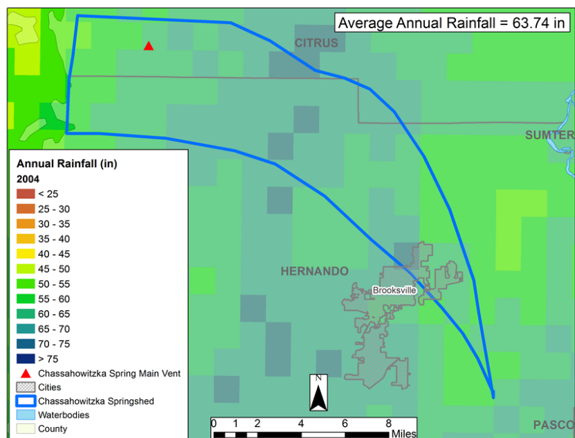
2004 Annual Rainfall Distribution within the Chassahowitzka Springshed
