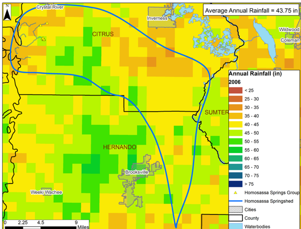
2006 Annual Rainfall Distribution within the Homosassa Springshed
