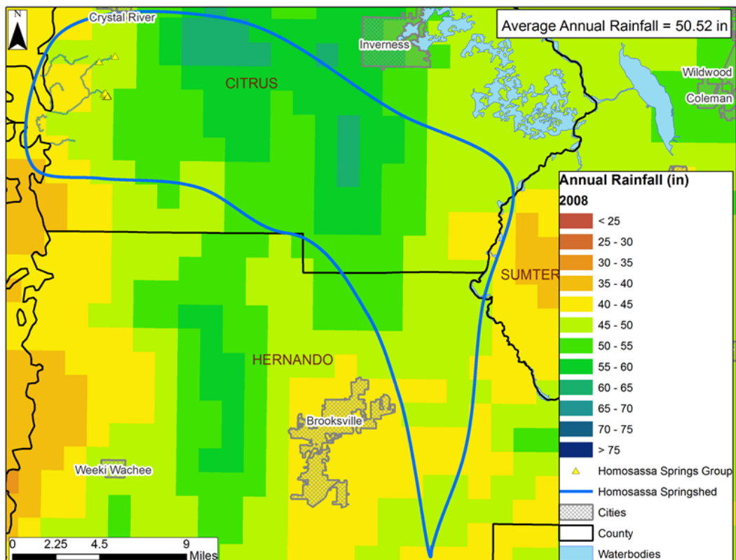
2008 Annual Rainfall Distribution within the Homosassa Springshed
