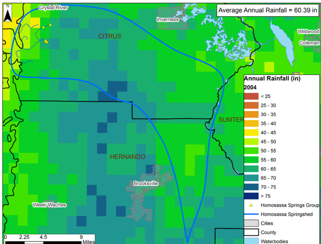
2004 Annual Rainfall Distribution within the Homosassa Springshed
