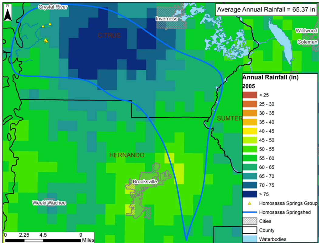
2005 Annual Rainfall Distribution within the Homosassa Springshed
