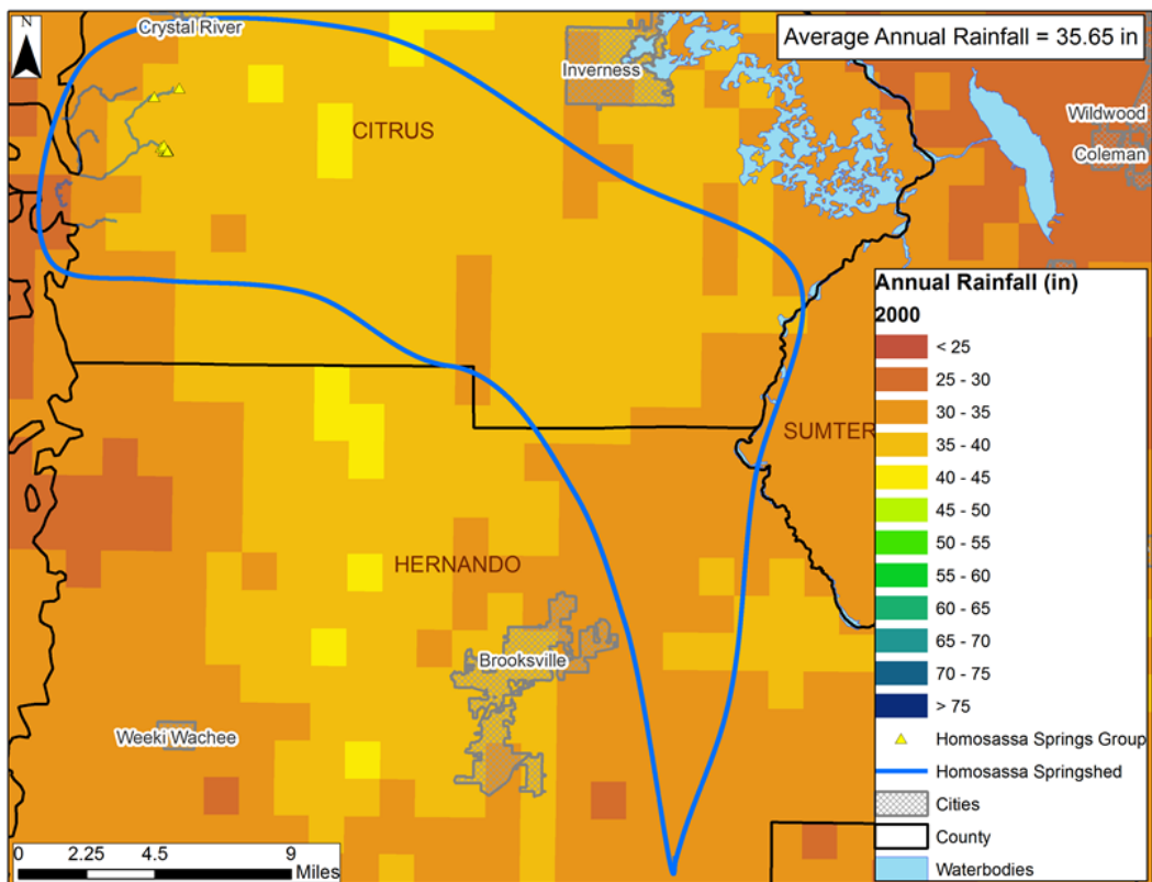
2000 Annual Rainfall Distribution within the Homosassa Springshed
