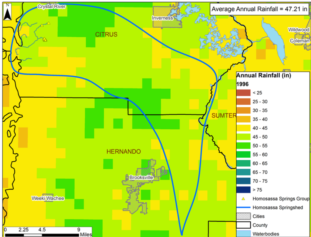
1996 Annual Rainfall Distribution within the Homosassa Springshed
