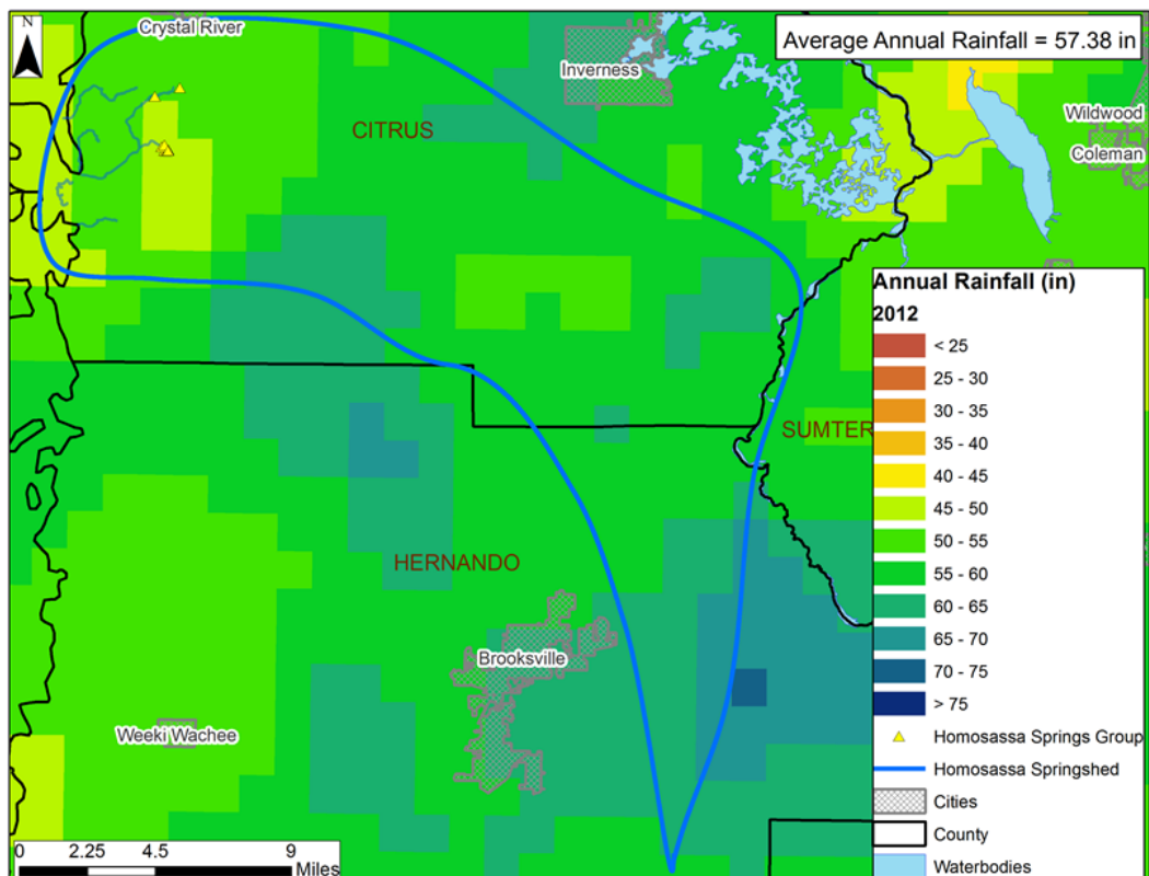
2012 Annual Rainfall Distribution within the Homosassa Springshed
