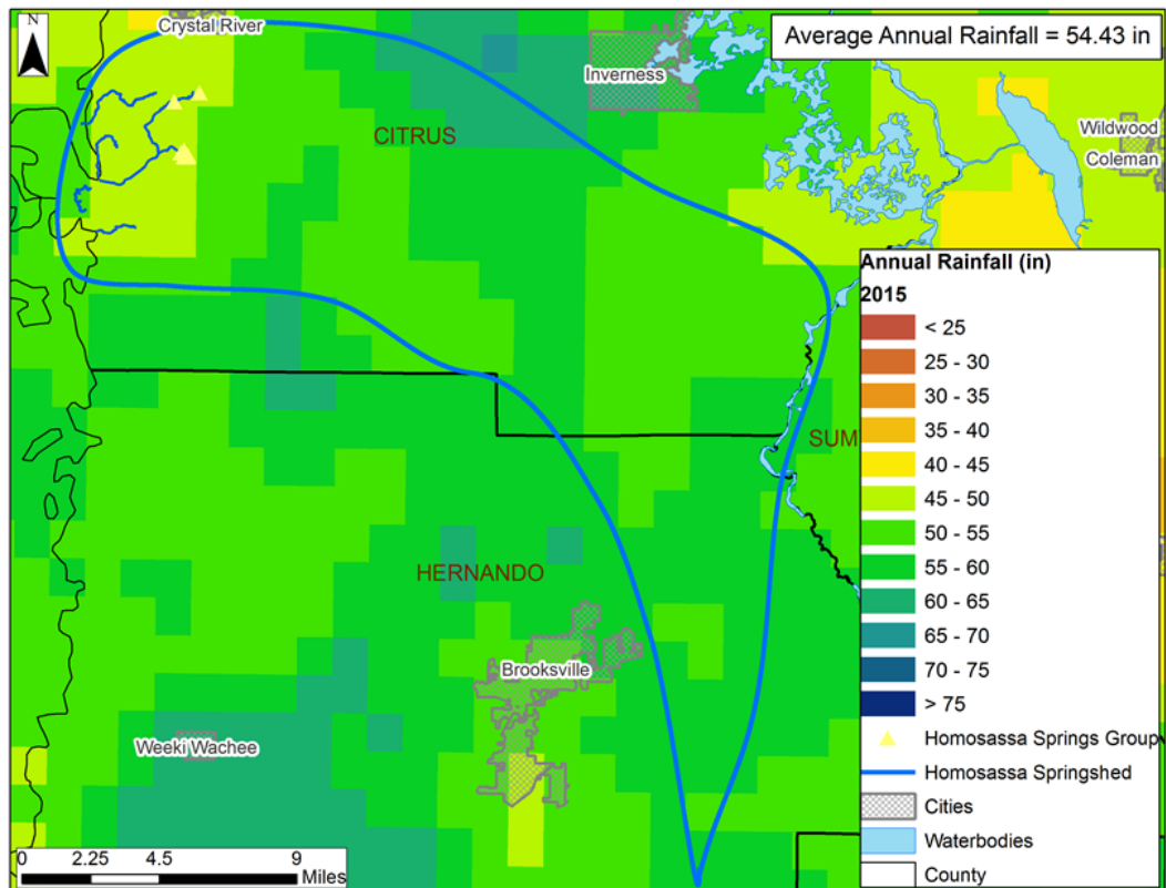
2015 Annual Rainfall Distribution within the Homosassa Springshed
