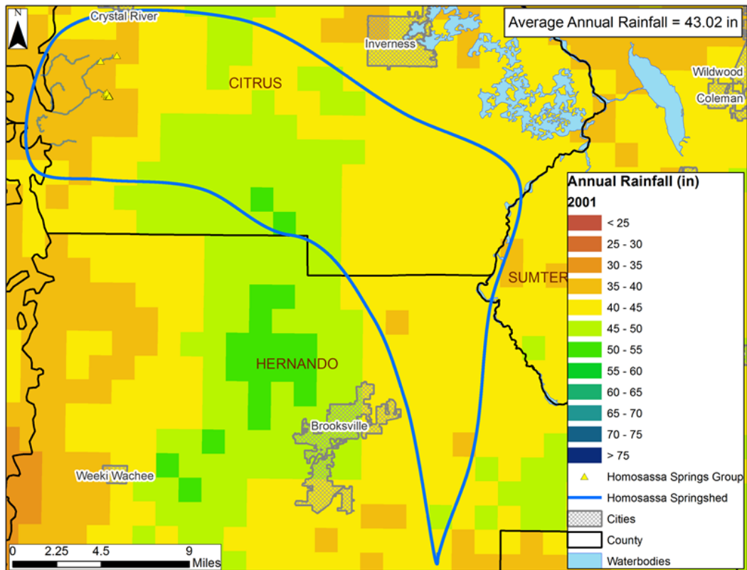
2001 Annual Rainfall Distribution within the Homosassa Springshed
