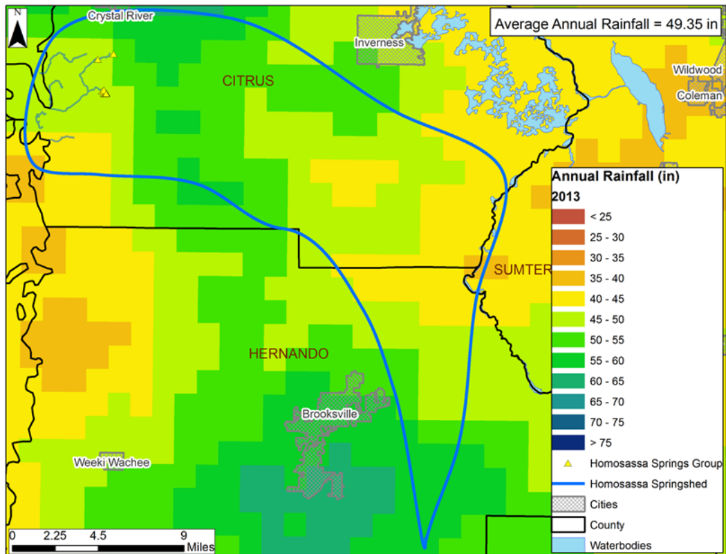
2013 Annual Rainfall Distribution within the Homosassa Springshed
