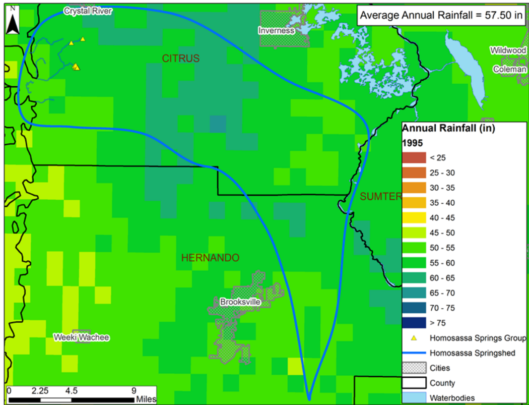
1995 Annual Rainfall Distribution within the Homosassa Springshed
