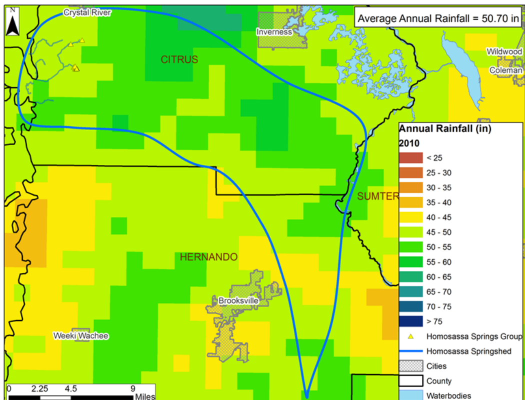
2010 Annual Rainfall Distribution within the Homosassa Springshed
