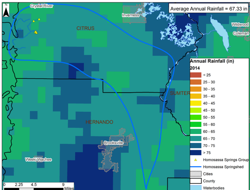
2014 Annual Rainfall Distribution within the Homosassa Springshed
