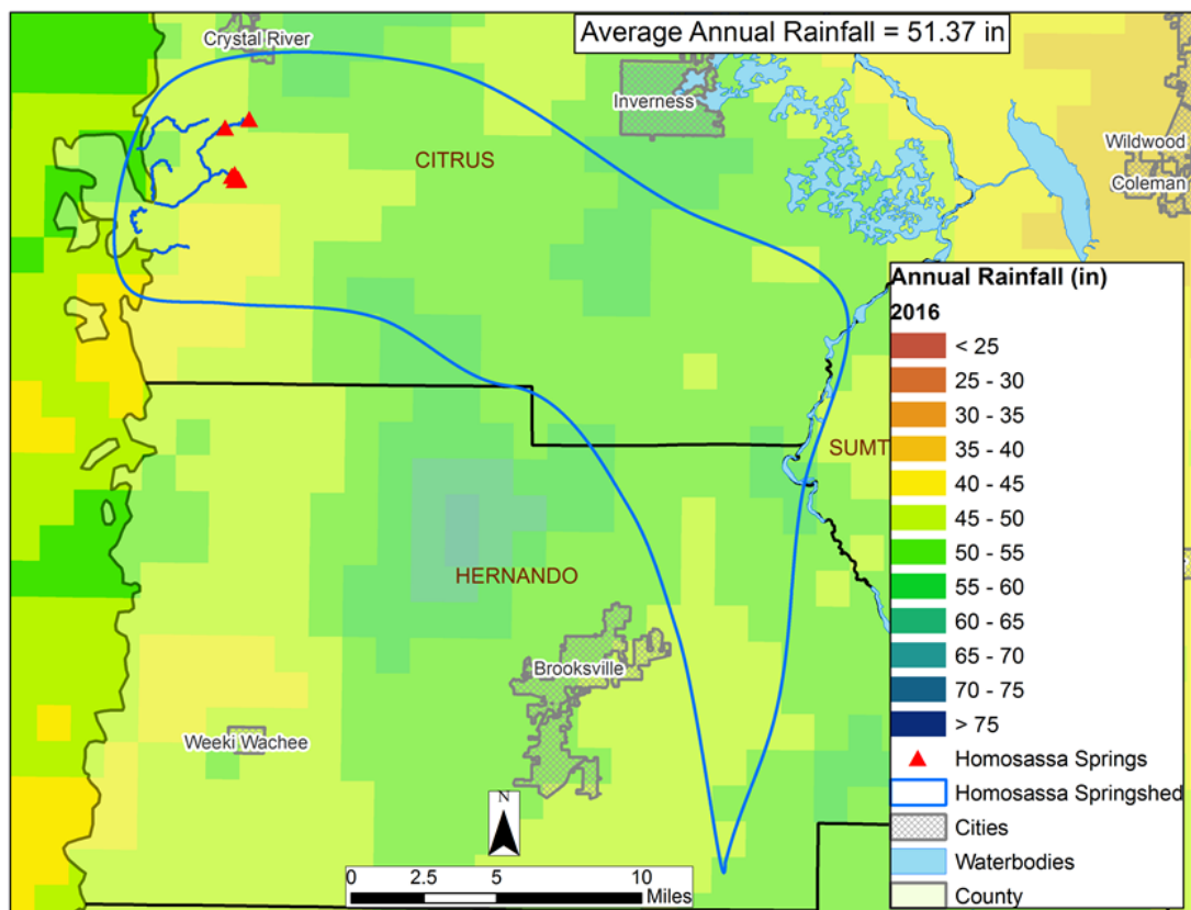
2016 Annual Rainfall Distribution within the Homosassa Springshed
