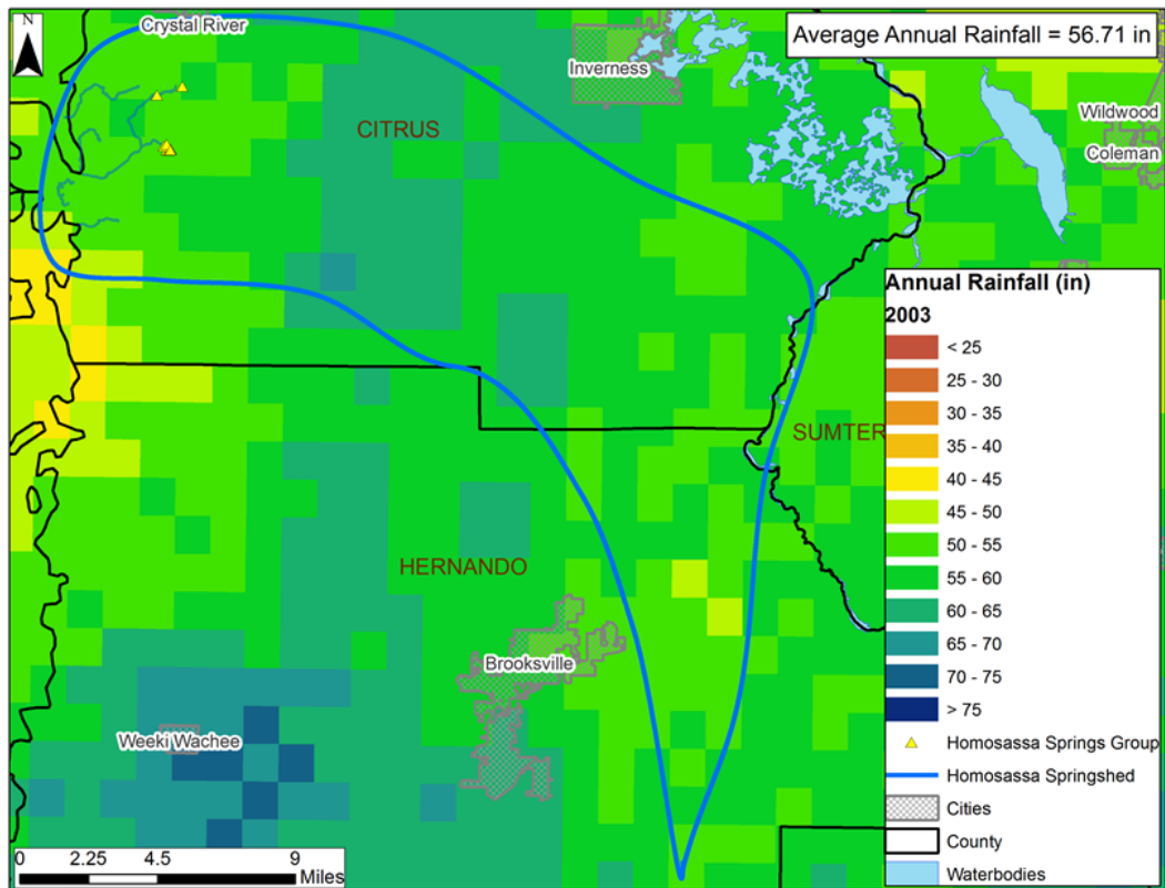
2003 Annual Rainfall Distribution within the Homosassa Springshed
