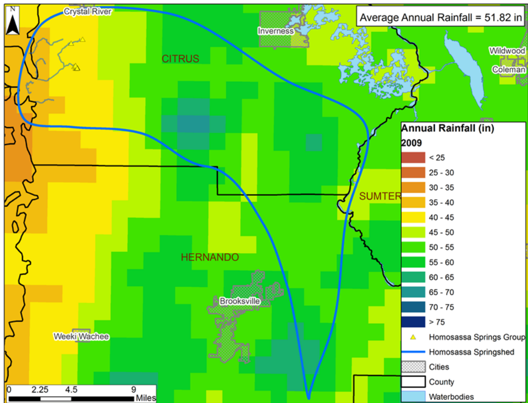
2009 Annual Rainfall Distribution within the Homosassa Springshed
