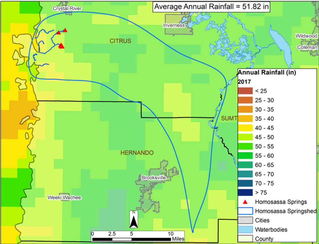
2017 Annual Rainfall Distribution within the Homosassa Springshed
