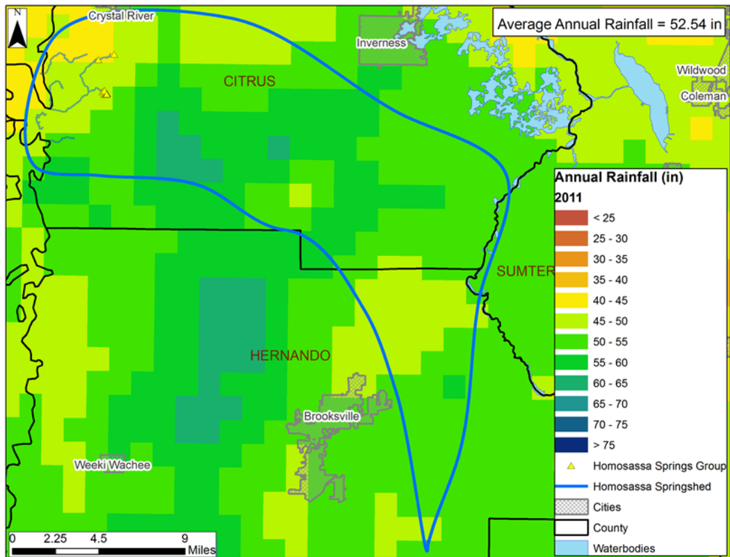
2011 Annual Rainfall Distribution within the Homosassa Springshed
