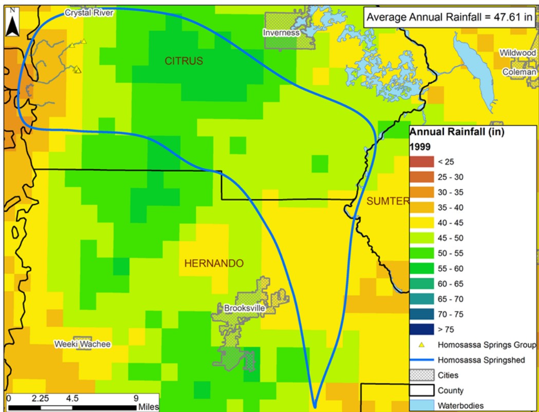
1999 Annual Rainfall Distribution within the Homosassa Springshed
