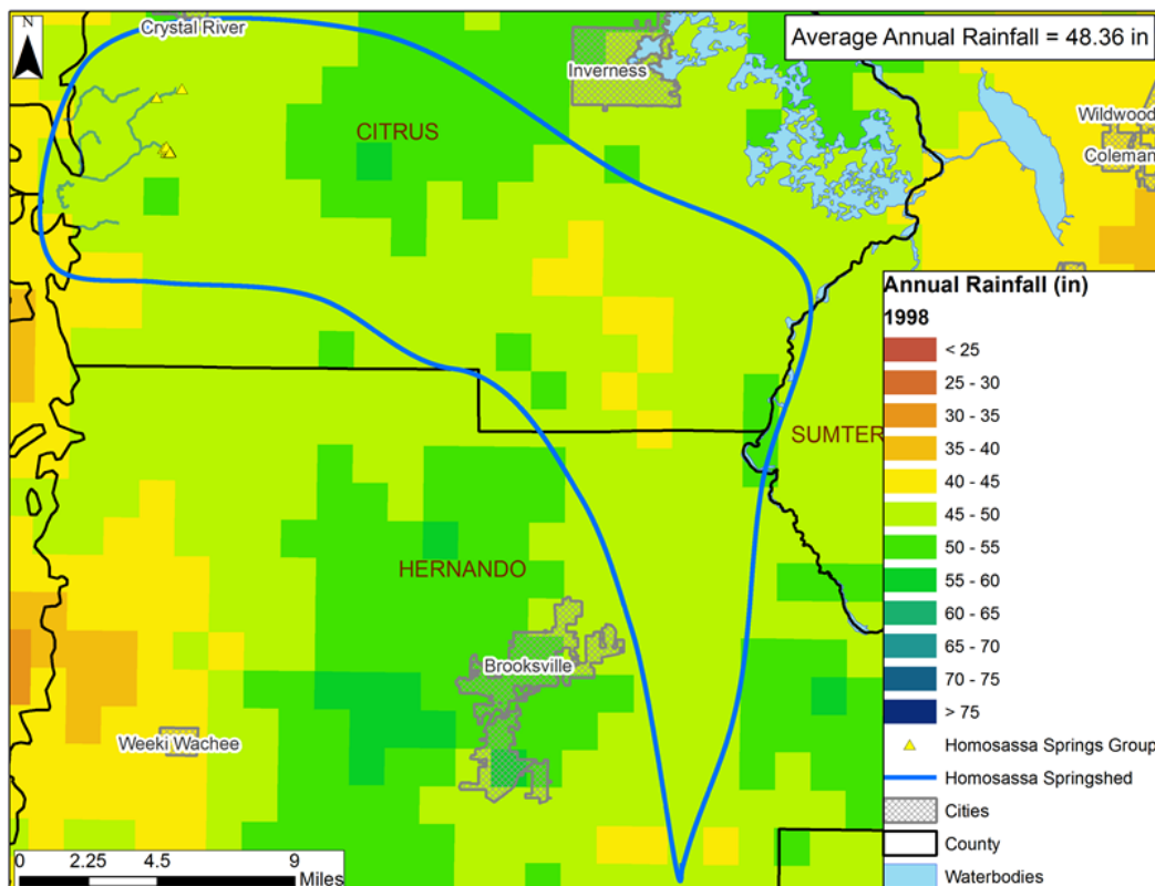
1998 Annual Rainfall Distribution within the Homosassa Springshed
