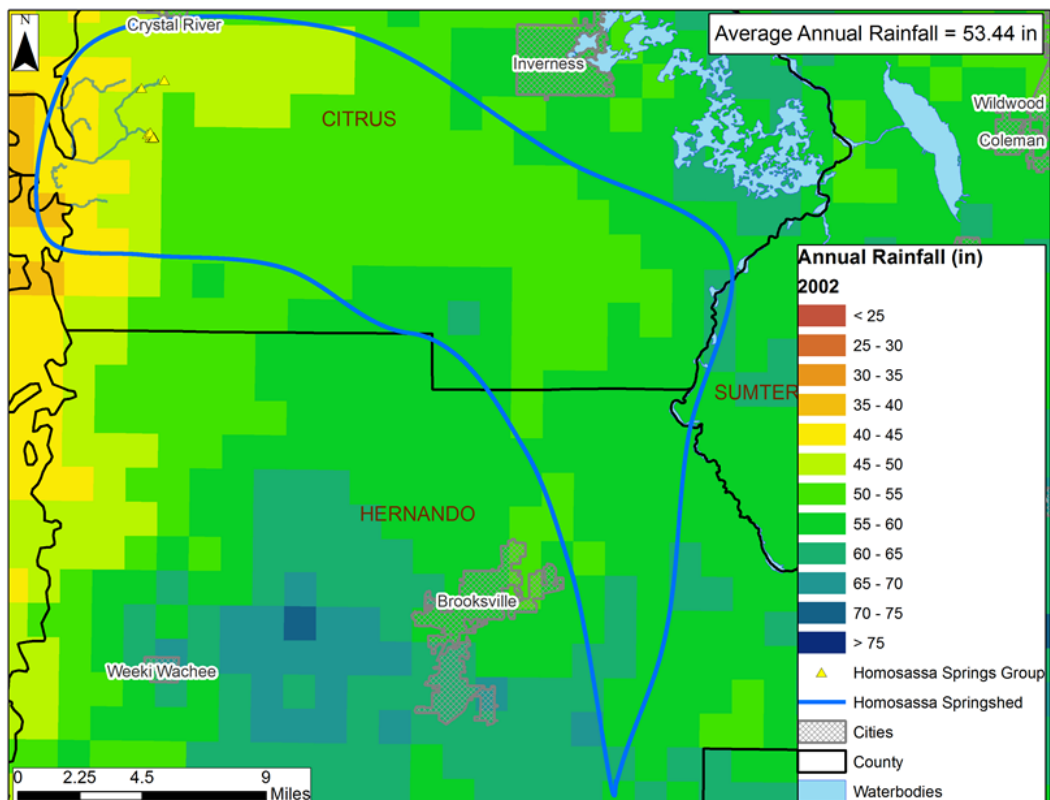
2002 Annual Rainfall Distribution within the Homosassa Springshed
