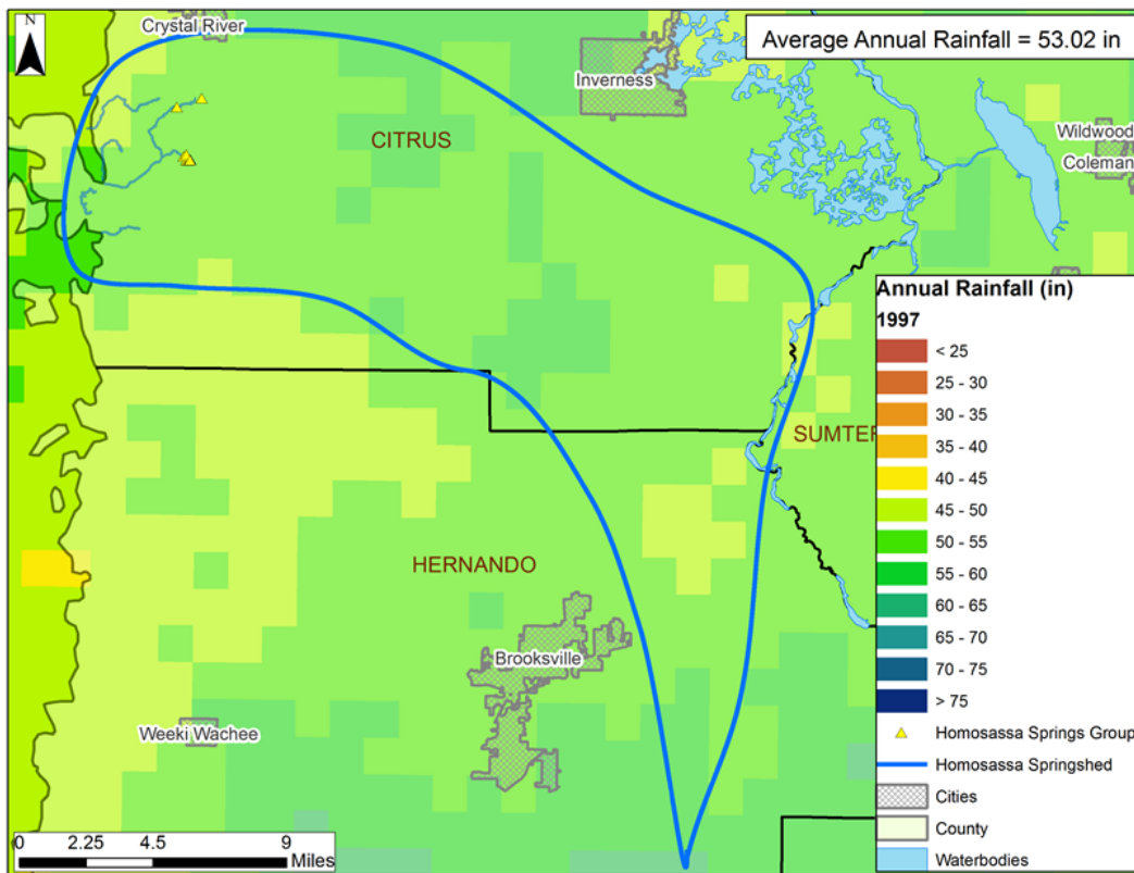
1997 Annual Rainfall Distribution within the Homosassa Springshed
