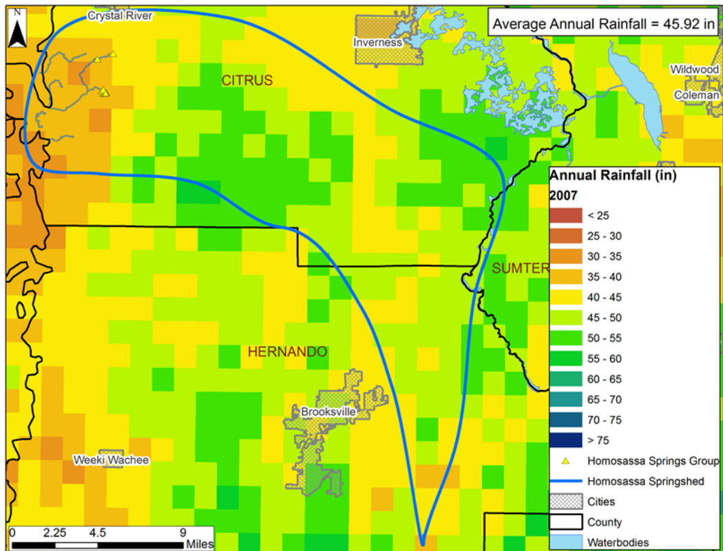
2007 Annual Rainfall Distribution within the Homosassa Springshed
