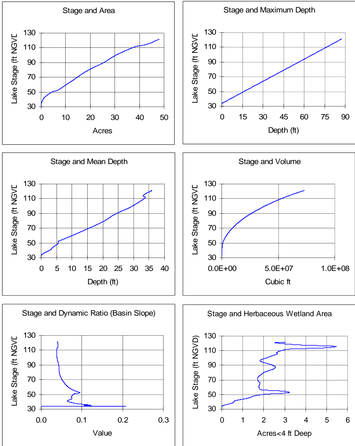
Figure 6. Surface area, maximum depth, mean depth, volume, dynamic ratio (basin slope), and potential herbaceous wetland area versus lake stage in feet above NGVD 29 for Lake Verona.
