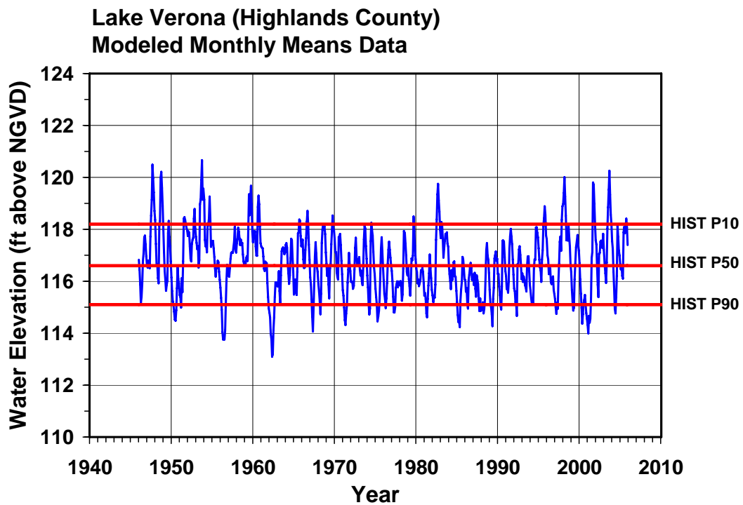
Figure 5. Modeled monthly-means surface water elevations in feet above NGVD 29 for the composite data set from January 1946 through December 2005 for Lake Verona, and the Historic P10, P50, and P90 lake stage percentile elevations.
