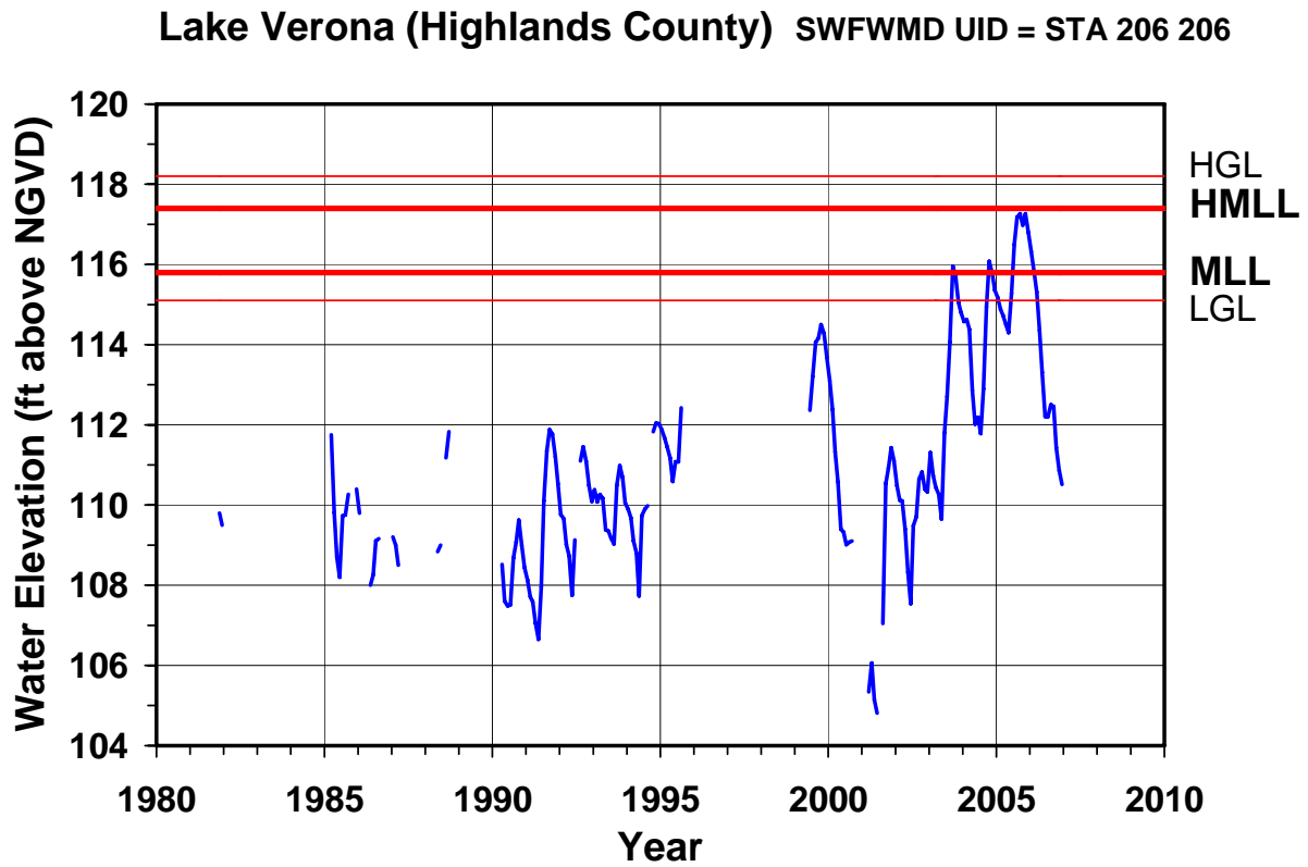
Figure 7. Mean monthly surface water elevations in feet above NGVD 29 through December 2006 based on measured lake stage records, and Minimum and Guidance Levels for Lake Verona. Levels include the High Guidance Level (HGL), Low Guidance Level (LGL), High Minimum Lake Level (HMLL), and Minimum Lake Level (MLL).
