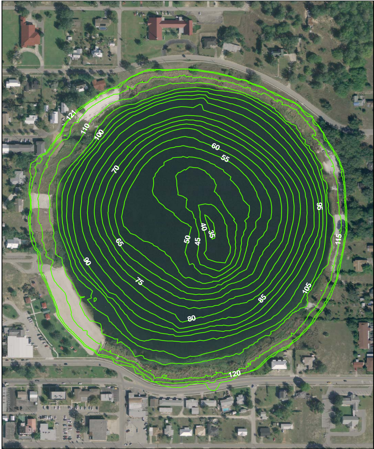
Figure 3. Five-foot contours within the Lake Verona basin. Values shown are elevations in feet above NGVD 29.
