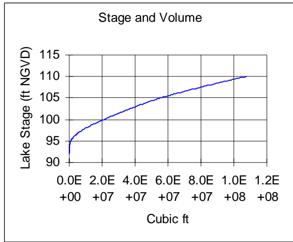
Figure 6. Surface area, volume, mean depth, dynamic ratio (basin slope), and potential herbaceous wetland area versus lake stage for Middle Lake.
