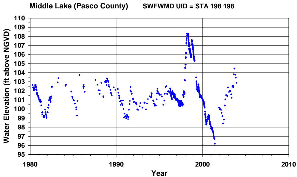
Figure 5. Mean monthly surface water elevations through December 2003, and proposed Guidance and Minimum Levels for Middle Lake. Proposed levels include the Ten-Year Flood Guidance Level (10-YR), High Guidance Level (HGL), Low Guidance Level (LGL), High Minimum Lake Level (HMLL), and Minimum Lake Level (MLL).
