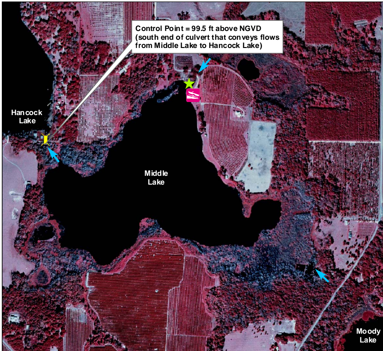
Figure 2. Location of lake water level gauge, boat ramp, inflows, outflow, and control point for Middle Lake.
