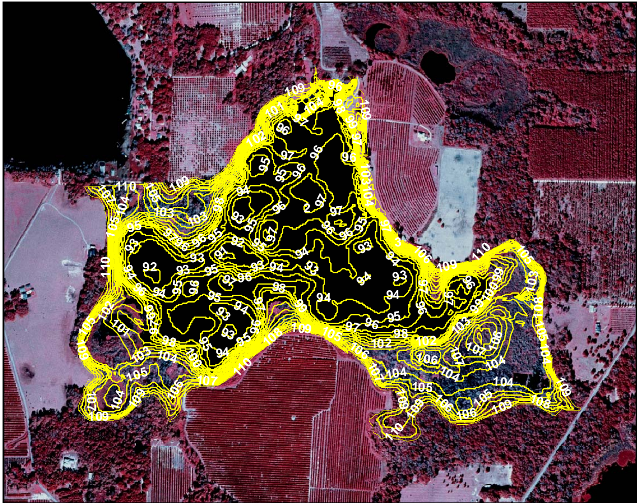
Figure 3. One foot contours within the Middle Lake basin. Values shown are elevations in feet above the National Geodetic Vertical Datum of 1929.
