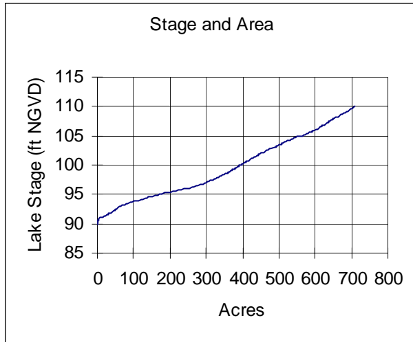
Figure 7. Surface area, volume, mean depth, dynamic ratio, and potential herbaceous wetland area versus lake stage for Hancock Lake in Pasco and Hernando Counties, Florida.
