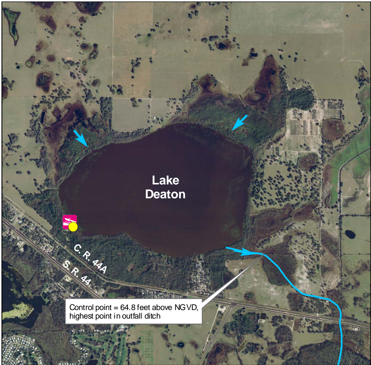
Figure 2. Location of lake water level gauge, public boat ramp, hydrologic indicators, inlets, outlet, outlet conveyance system, water control structure, and control point for Lake Deaton.
