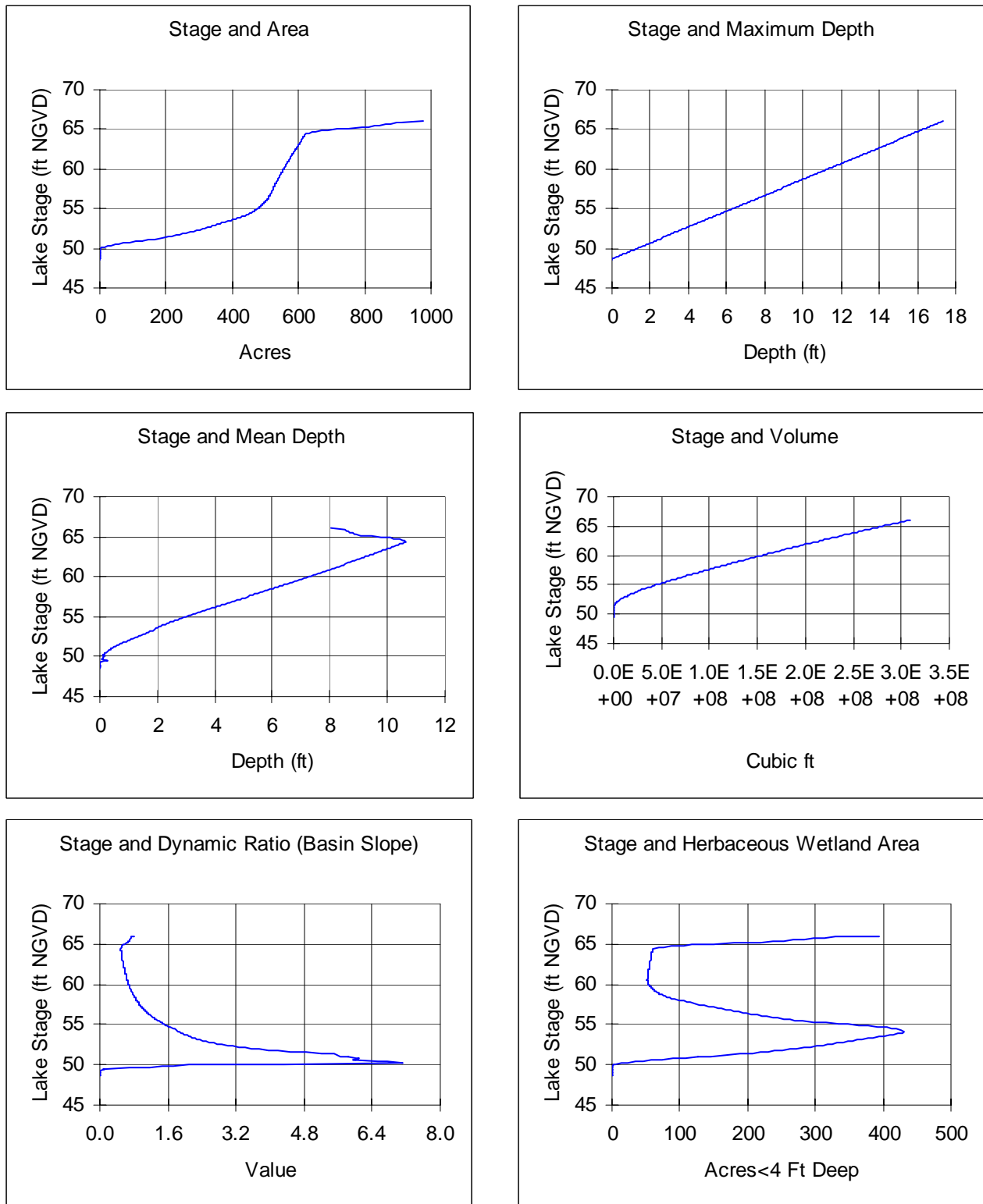
Figure 6. Surface area, maximum depth, mean depth, volume, dynamic ratio (basin slope), and potential herbaceous wetland area versus lake stage for Lake Deaton.
