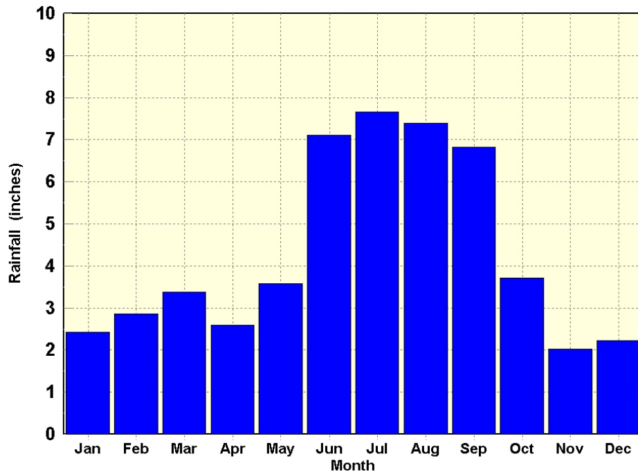
Figure 3. Average monthly rainfall from NWS Regions 3 and 4 (period-of-record 1895-2000).
