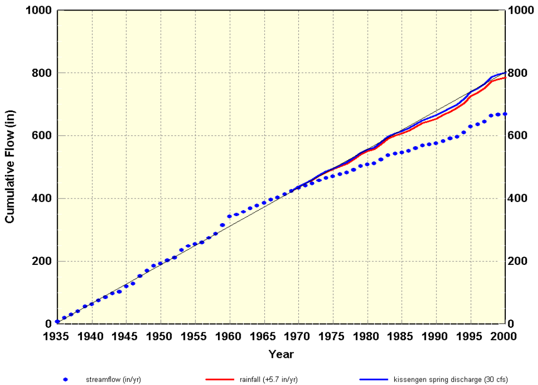
Figure 35. Single mass plot of Peace River flow at Zolfo Springs with streamflow adjusted to account for rainfall decline and Kissengen Spring discharge.
