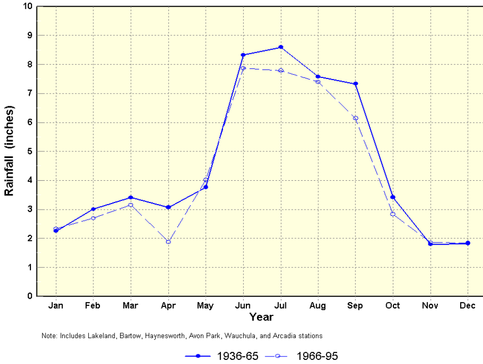
Figure 12. Comparison of monthly rainfall between two 30-year periods (1936-1965 and 1966-1995).
