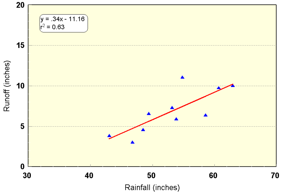
Figure 31. Regression of annual rainfall versus flow at the Bartow gaging station based on a 10-year HSPF simulation.
