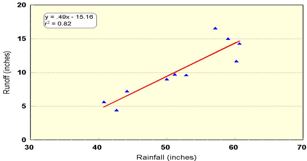
Figure 33. Regression of annual rainfall versus flow at the Arcadia gaging station based on a 10-year HSPF simulation.
