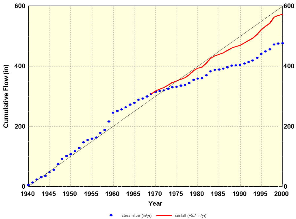
Figure 34. Single mass plot of Peace River flow at Bartow with streamflow adjusted to account for rainfall decline.
