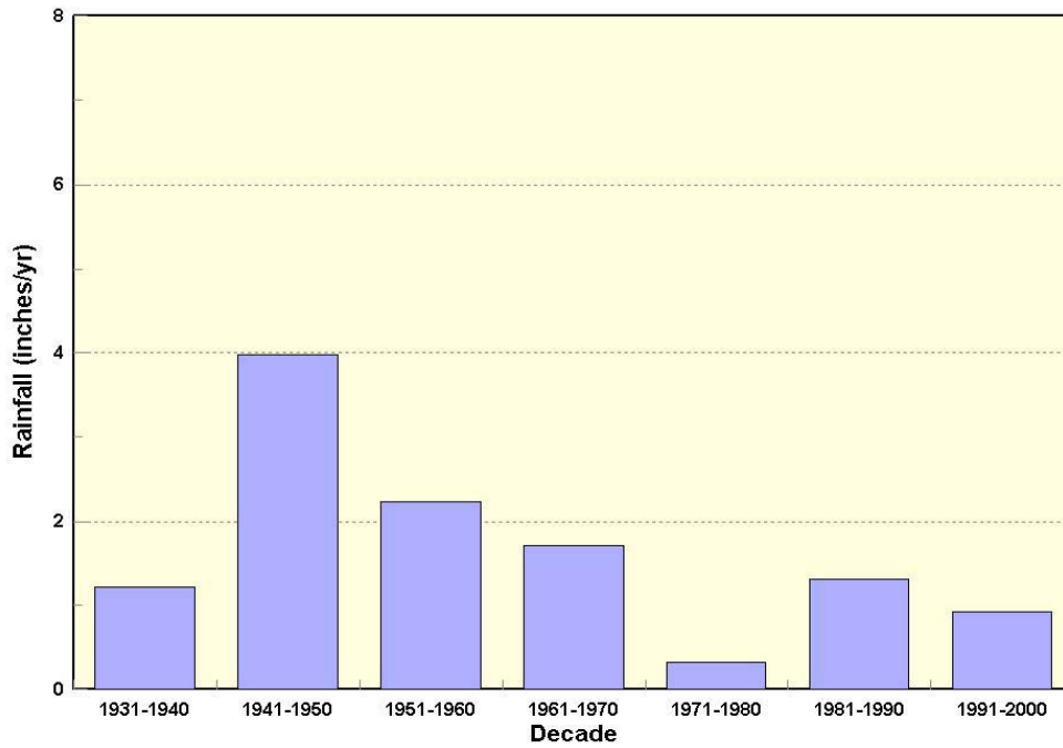
Figure 23. Tropical cyclone rainfall contribution by decade in the Peace River basin (1931-2000).
