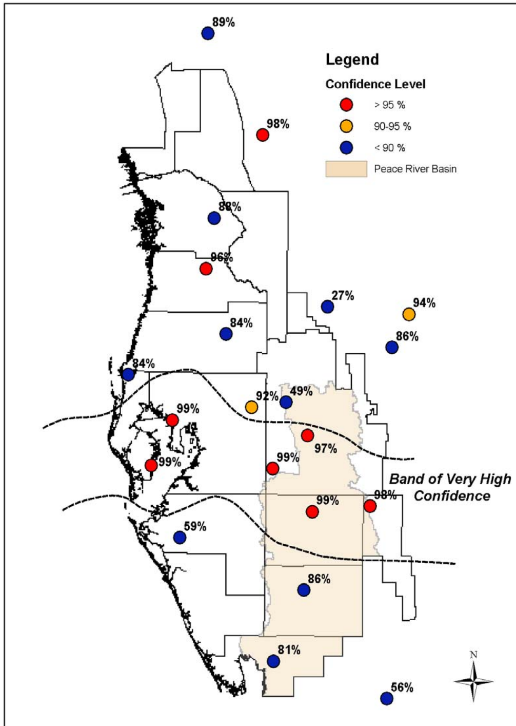
Figure 26. Probability that Post-1965 Precipitation is Less Than Pre-1965 Precipitation.
