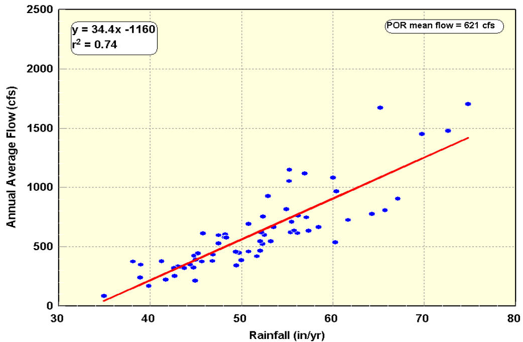
Figure 28. Regression of annual rainfall versus flow at the Bartow gaging station.
