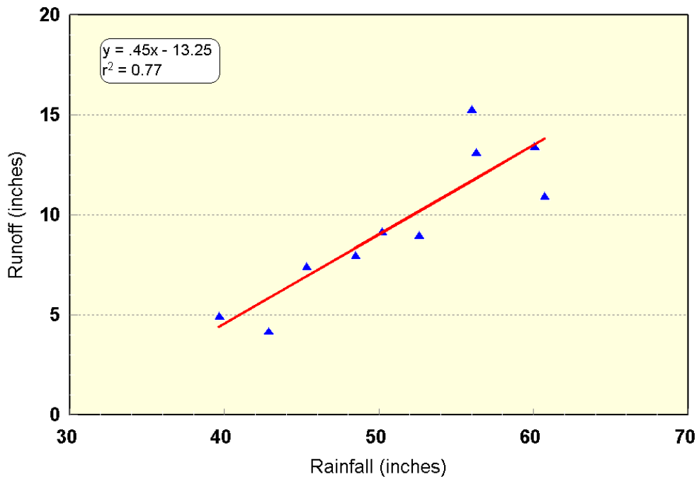
Figure 31. Regression of annual rainfall versus flow at the Bartow gaging station based on a 10-year HSPF simulation.
