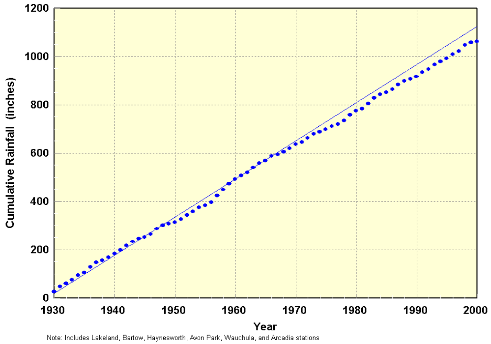
Figure 18. Single mass plot of dry season rainfall (January through May).
