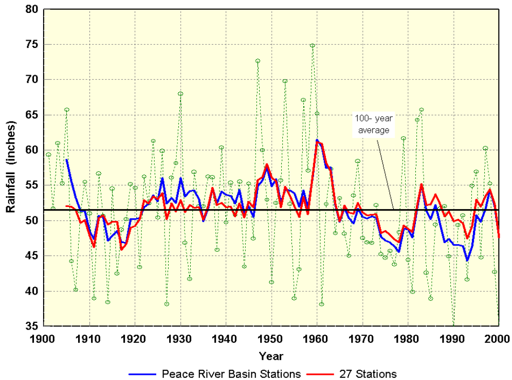
Figure 8. Annual and 5-year running mean rainfall averaged from Peace River basin stations compared with 5-year running mean from 27 long-term stations.
