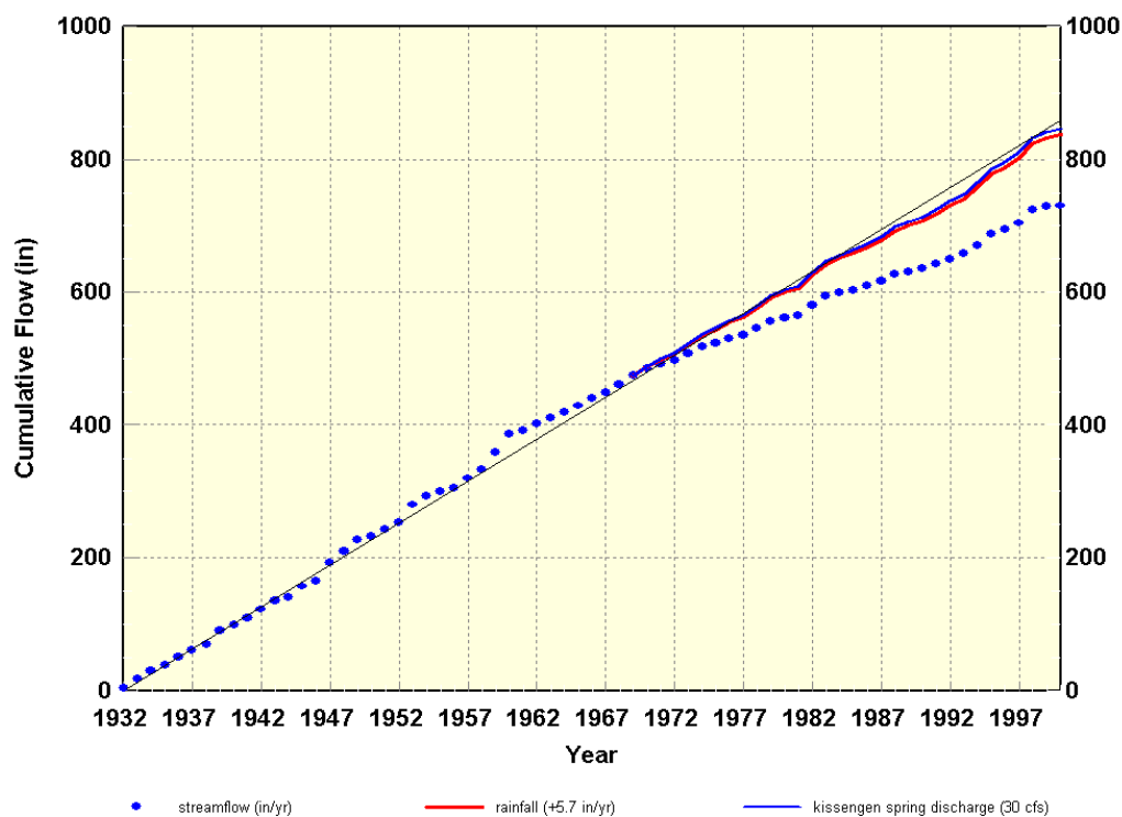
Figure 36. Single mass plot of Peace River flow at Arcadia with streamflow adjusted for rainfall decline and Kissengen Spring discharge.
