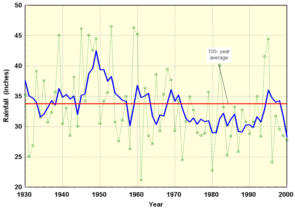
Figure 16. Annual and 5-year running mean of wet season rainfall (June through September).
