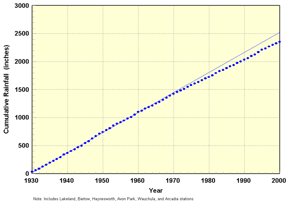
Figure 14. Single mass plot of wet season rainfall (June through September).
