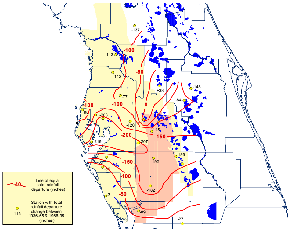
Figure 11. Total change in rainfall departure between two 30-year periods (1966-1995 minus 1936-1965).
