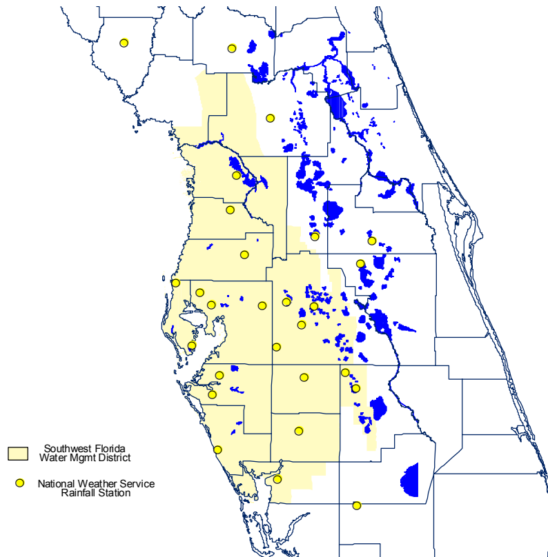
Figure 1. Location of 27 long-term rainfall stations.
