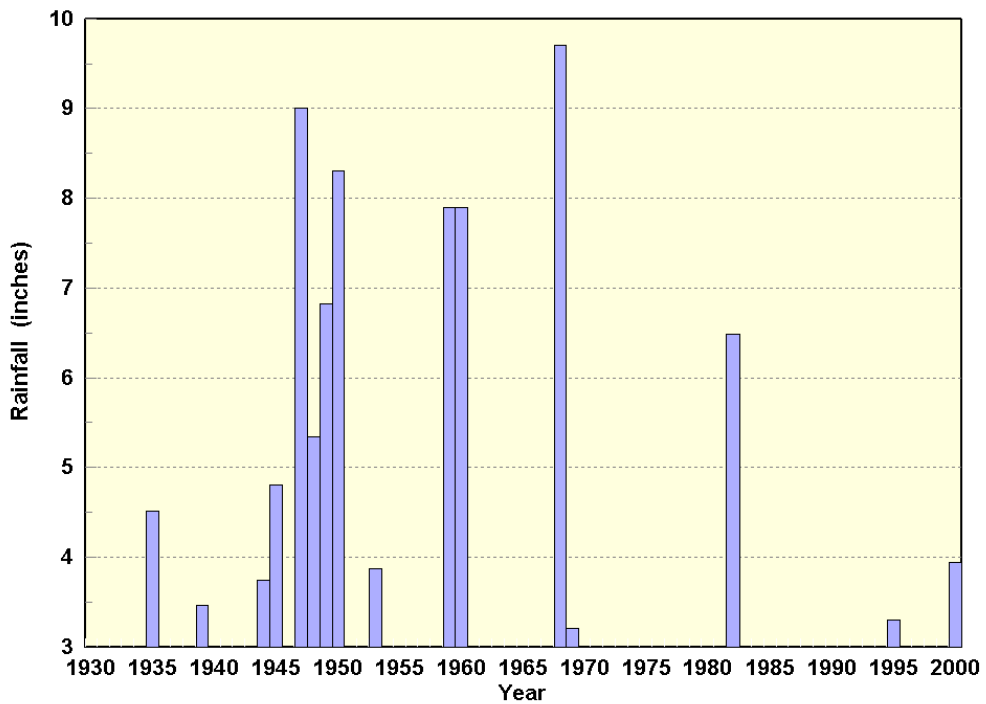
Figure 24. Tropical cyclone contribution (>3 inches) to wet season rainfall in the Peace River basin (1930-2000).
