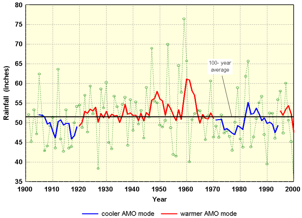
Figure 5. Annual and 5-year running mean rainfall averaged from 27 long-term stations.
