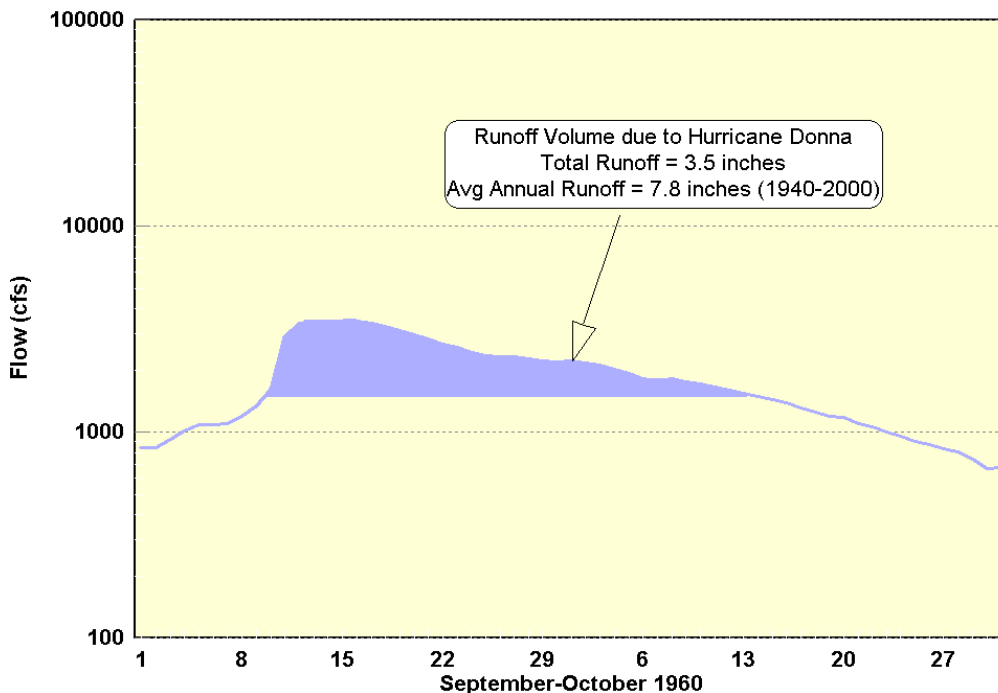
Figure 25. Runoff contribution at Bartow from Hurricane Donna.
