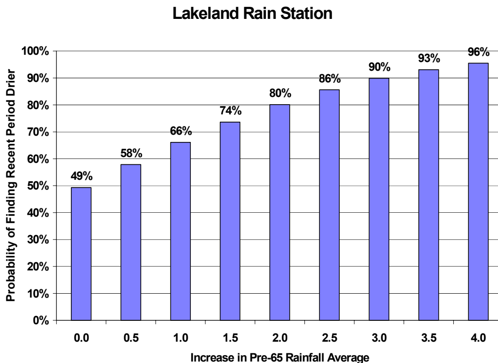
Figure 27. Change in probability of finding recent 30-year period drier by increasing pre-1965 mean rainfall.
