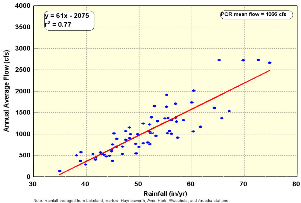
Figure 30. Regression of annual rainfall versus flow at the Arcadia gaging station.
