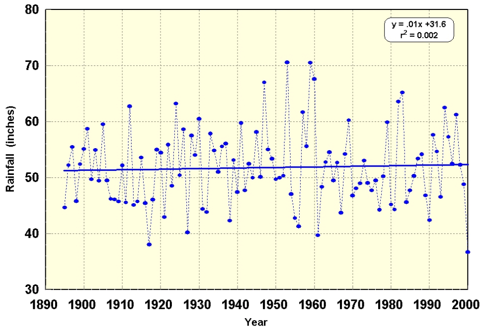
Figure 4. Linear regression of 105 years of annual rainfall from National Weather Service Regions 3 and 4 (see Figure 2 for location).
