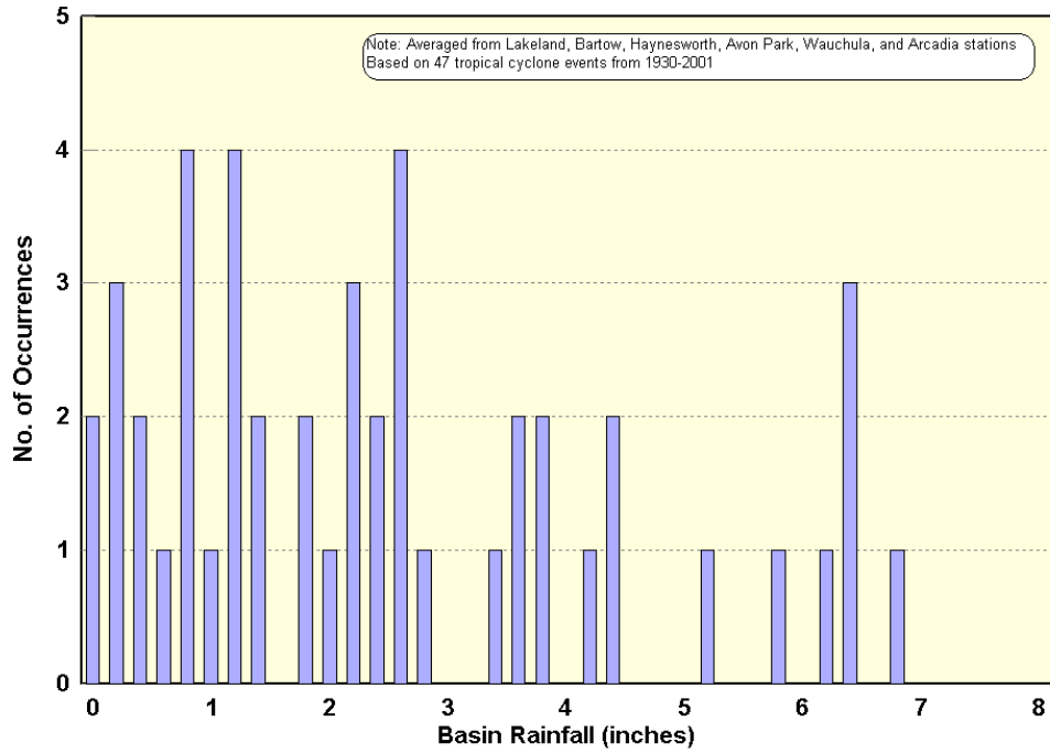
Figure 21. Histogram of tropical cyclone precipitation totals affecting the Peace River basin (1930-2001).
