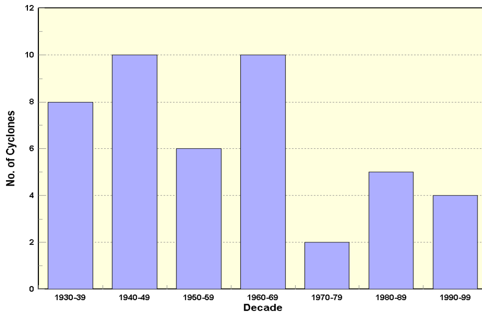
Figure 20. Number of tropical cyclones affecting the Peace River basin (1930-1999).
