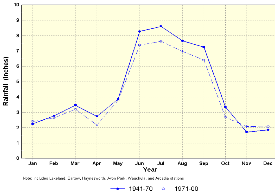
Figure 13. Comparison of monthly rainfall between two 30-year periods (1941-1970 and 1971-2000).
