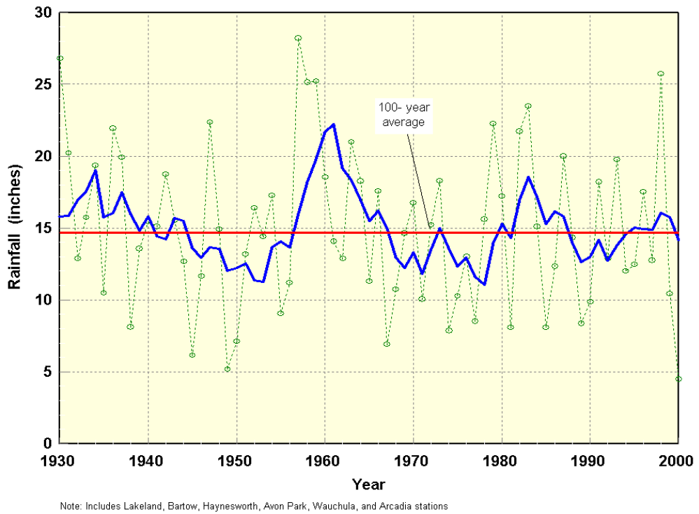
Figure 19. Annual and 5-year running mean of dry season rainfall (January through May).
