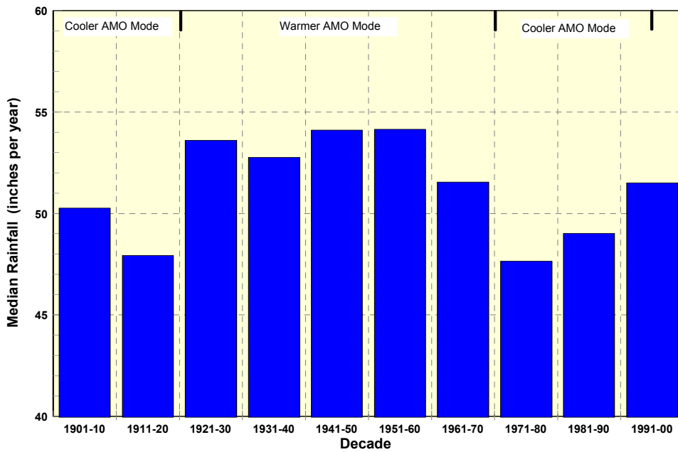
Figure 6. Median rainfall by decade averaged from 27 long-term stations.
