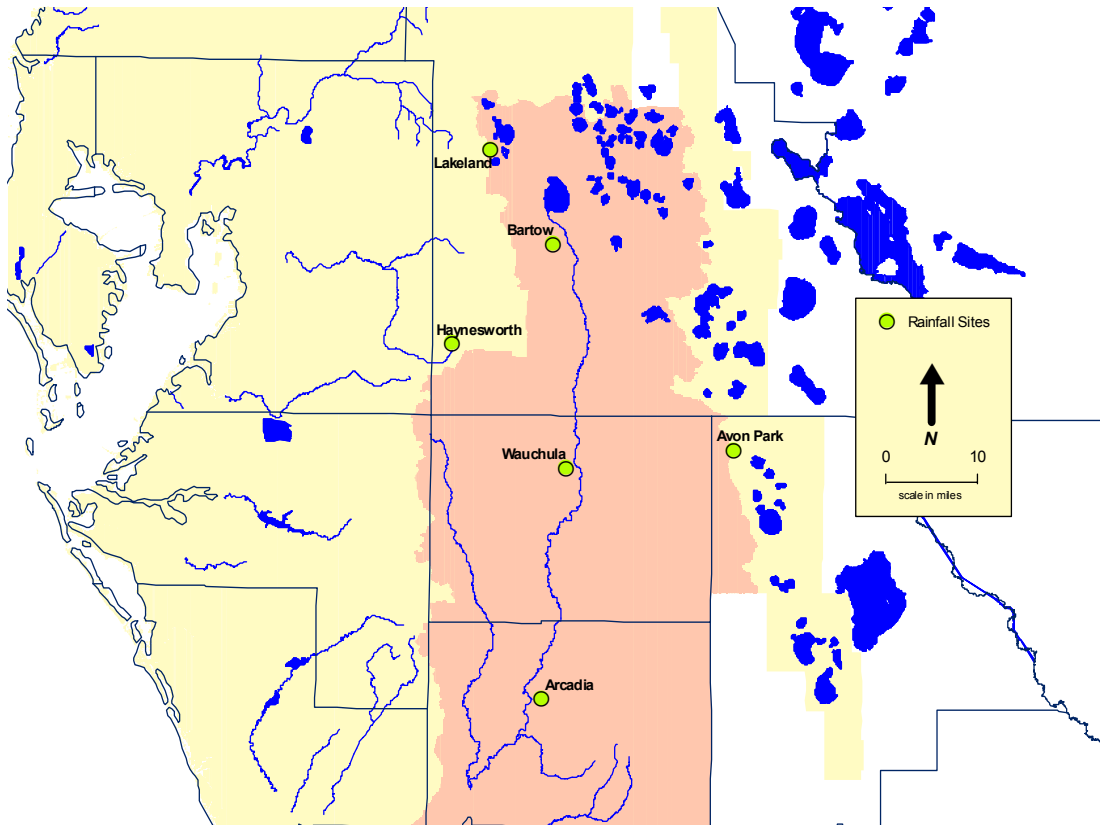
Figure 7. Location of long-term rainfall stations within or adjacent to the Peace River basin.
