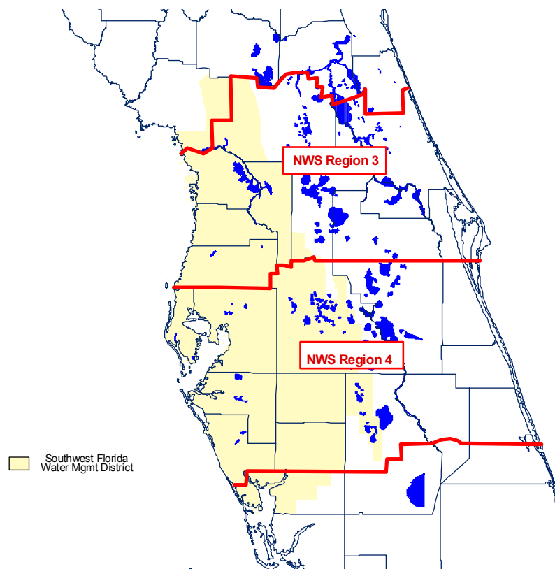
Figure 2. Location of National Weather Service's North-Central (Region 3) and South-Central (Region 4) rainfall zones.
